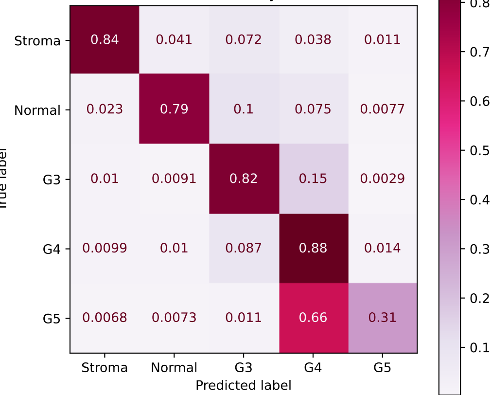
Confusion matrix using optimal_transport_loss_v1_no_detach for KFBio balanced accuracy = 72.94%
