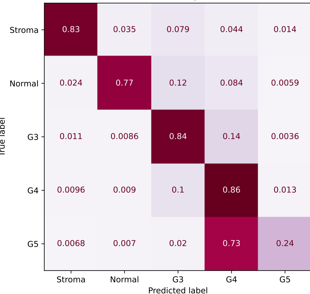
Confusion matrix using optimal_transport_loss_v3_p=5 for KFBio balanced accuracy = 70.61%
