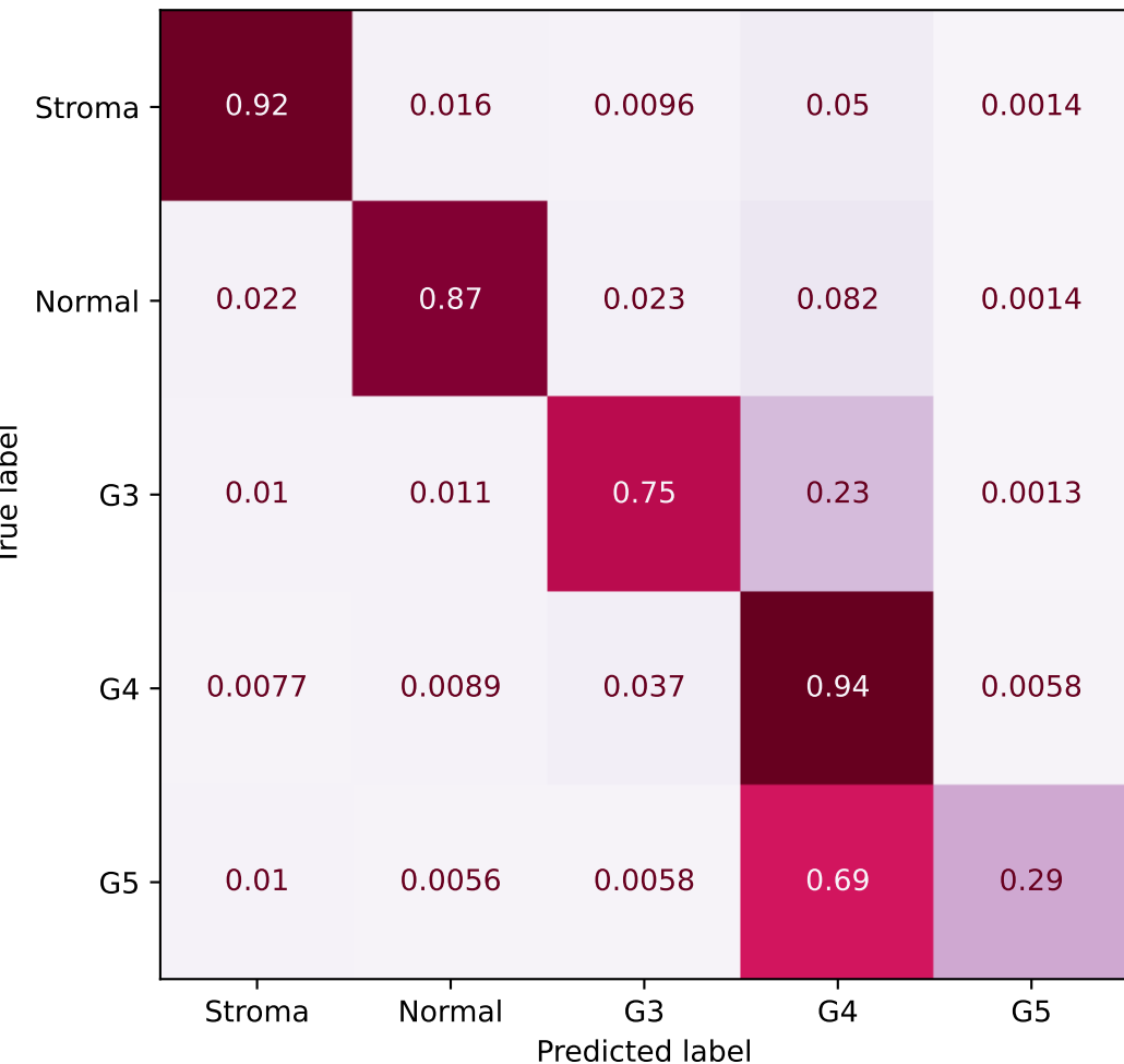
Confusion matrix using baseline_multi for KFBio balanced accuracy = 75.45%
