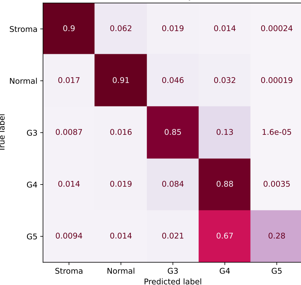
Confusion matrix using baseline_multi for KFBio_FDA balanced accuracy = 76.41%
