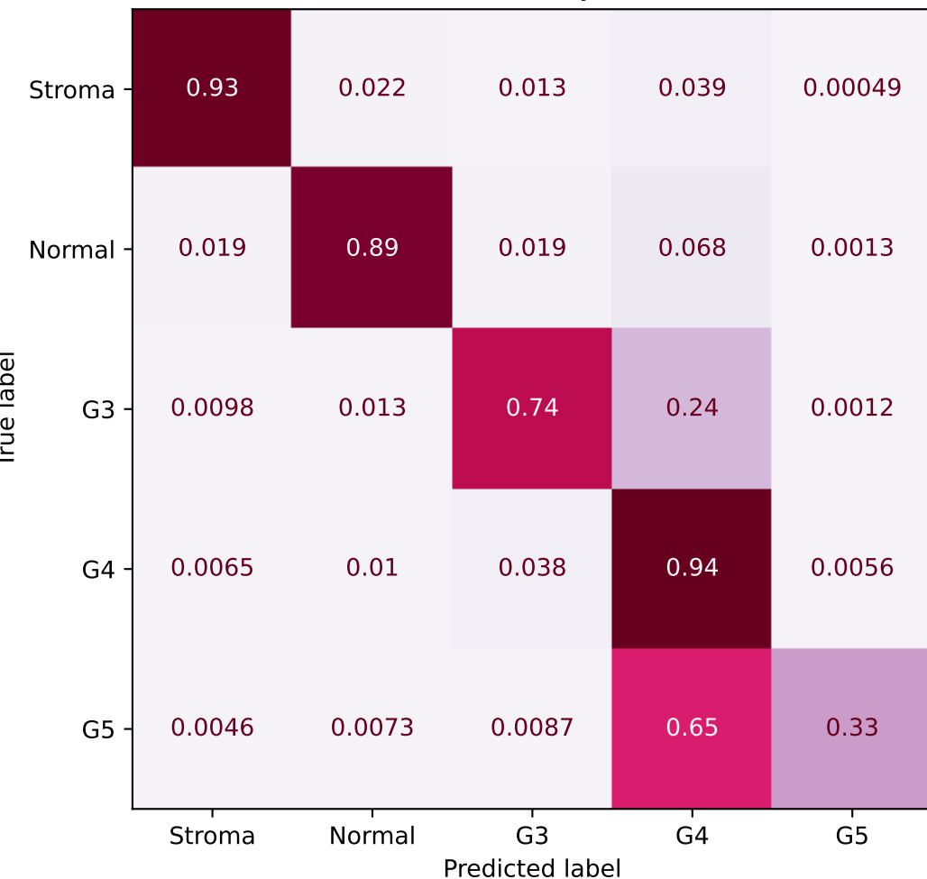
Confusion matrix using OT_multi for KFBio balanced accuracy = 76.51%
