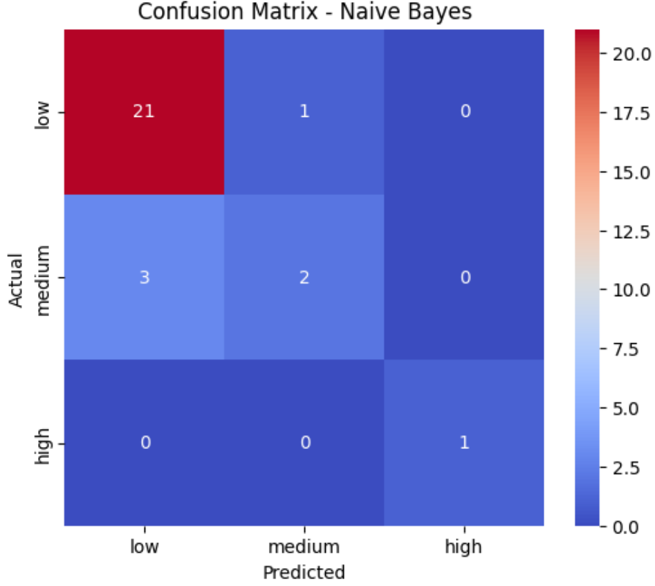
Figure 3: Confusion Matrix
