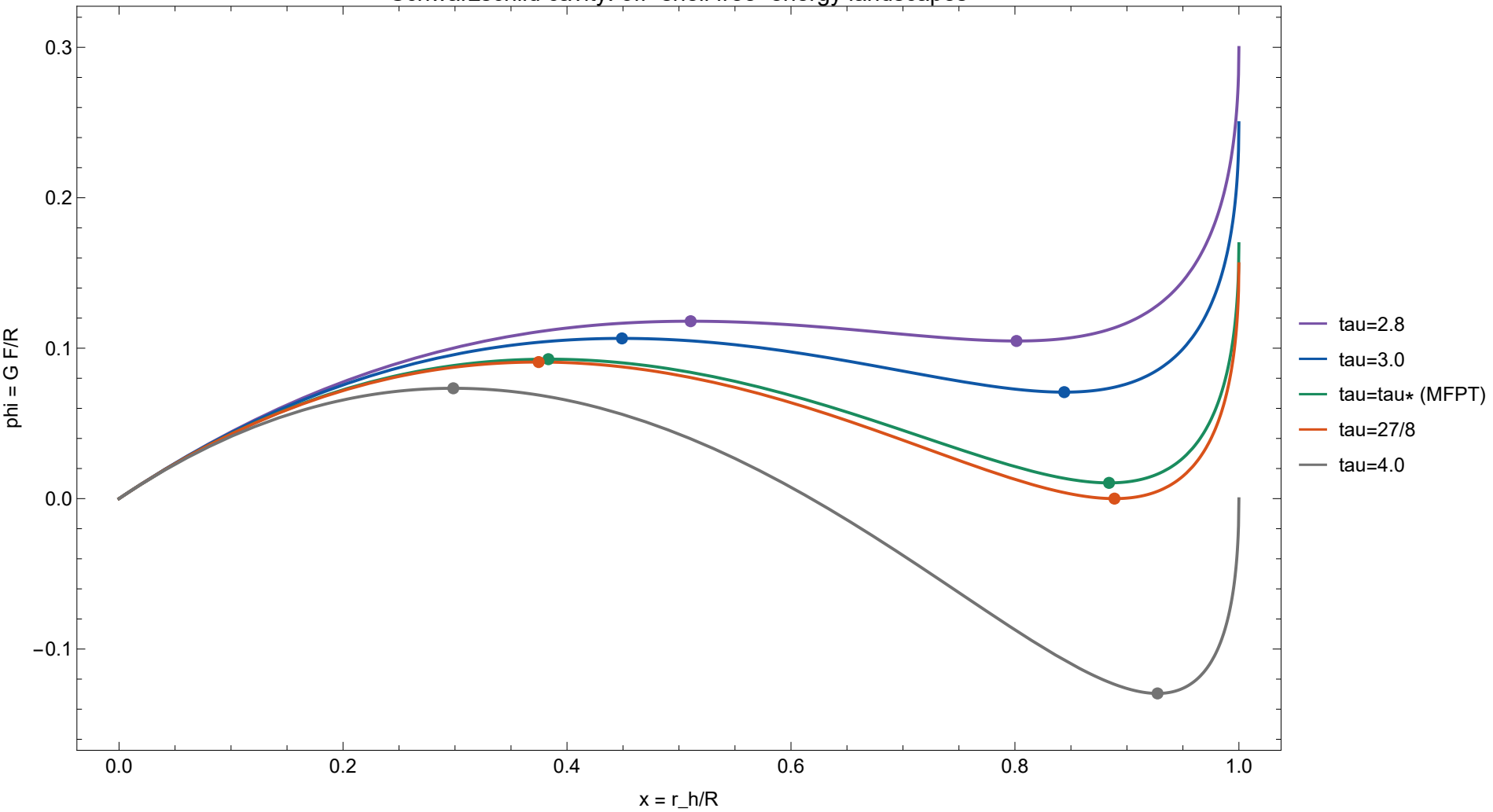
Schwarzschild cavity: off-shell free-energy landscapes
