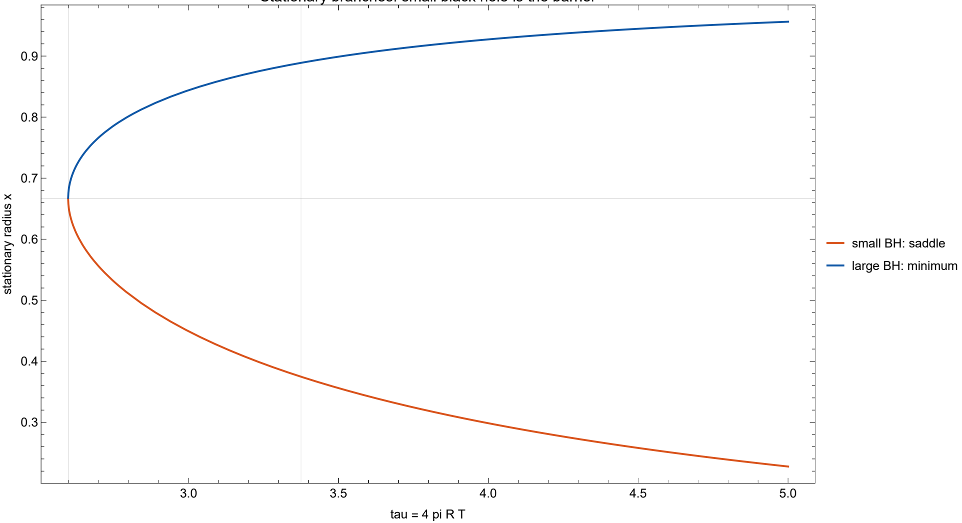
Stationary branches: small black hole is the barrier
