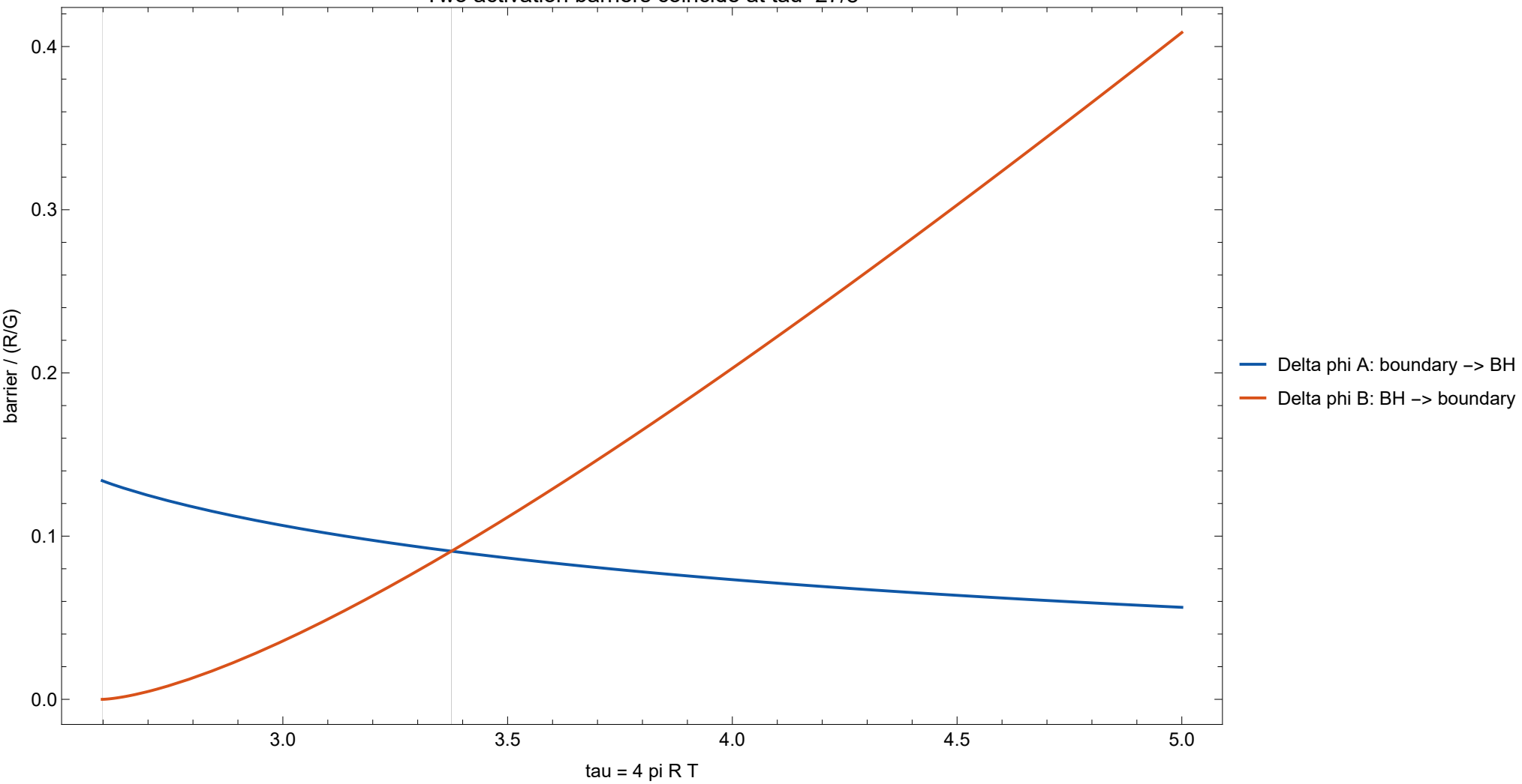
Two activation barriers coincide at \tau=27/8
