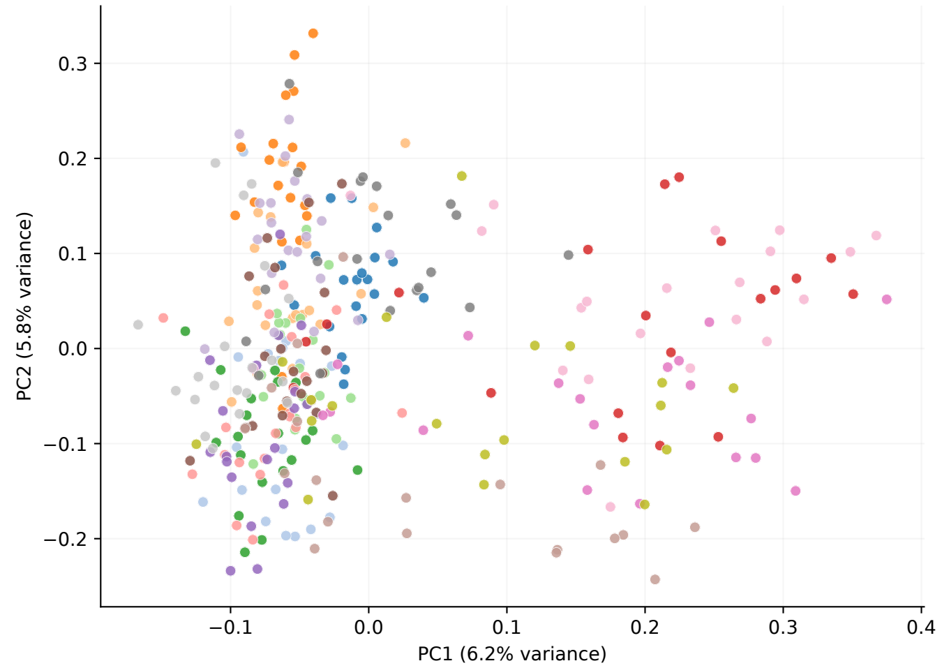
DLRSD | RemoteCLIP ViT-L-14 340 attribute suffixes, 17 classes
