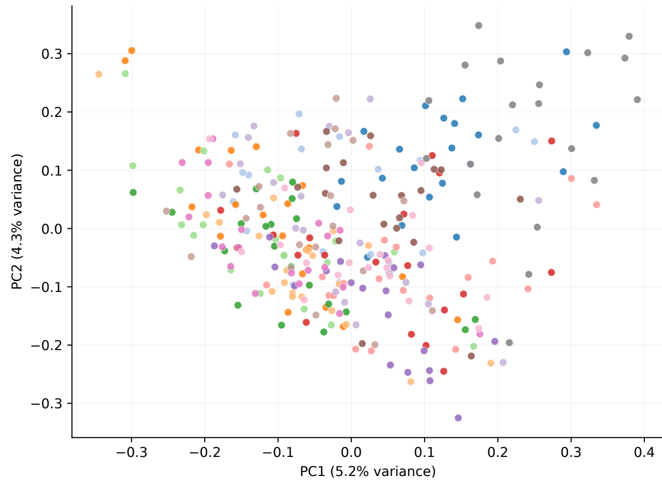
iSAID | RemoteCLIP ViT-B-32 300 attribute suffixes, 15 classes
