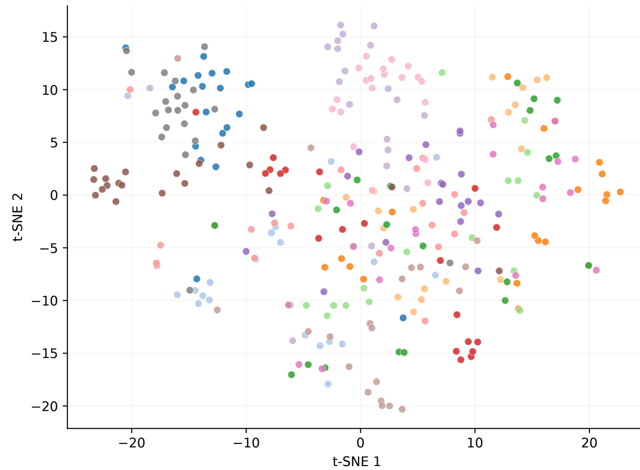
iSAID | RemoteCLIP ViT-L-14 300 attribute suffixes, 15 classes
