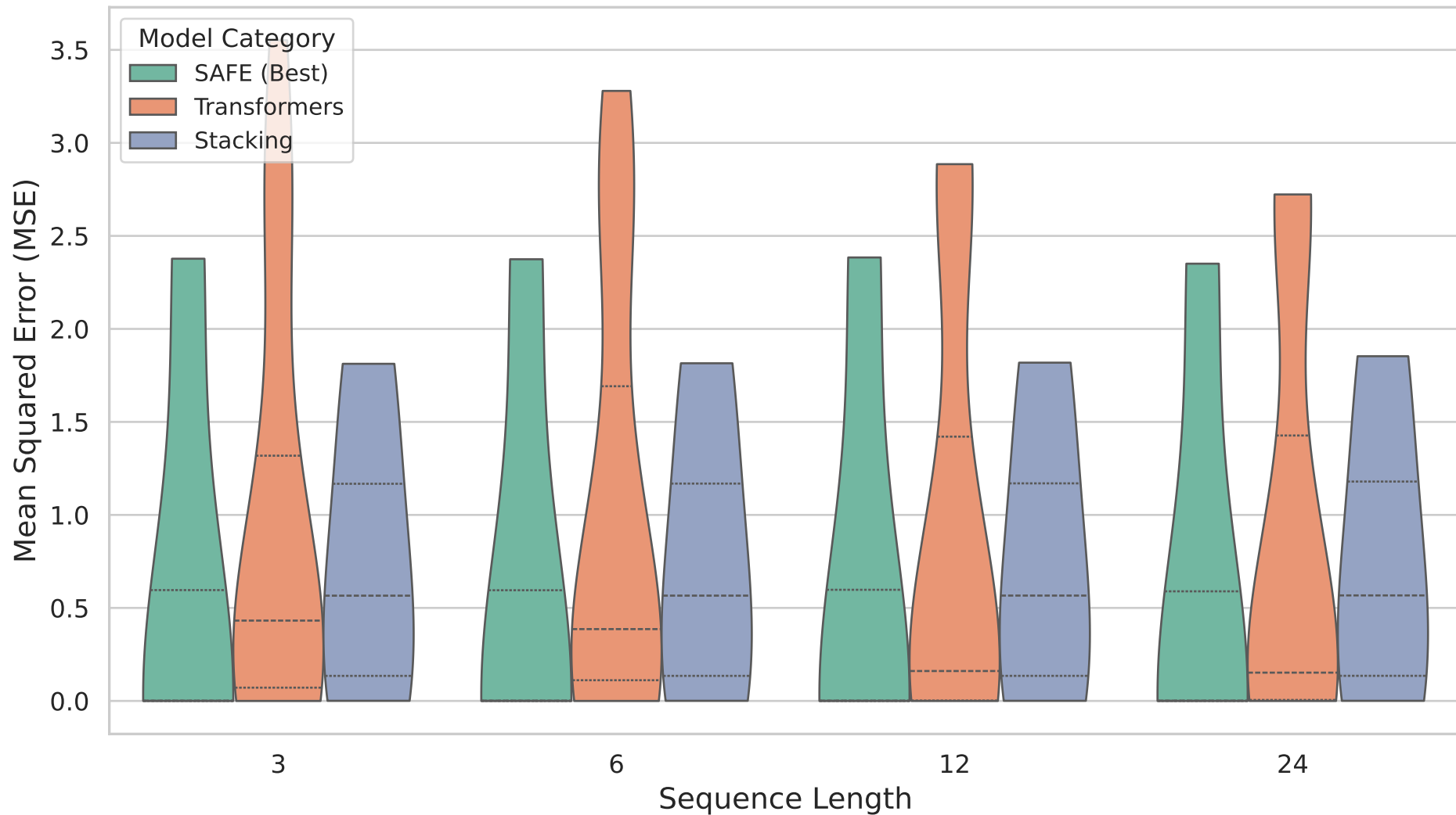
Performance Distribution: SAFE vs. Baselines
