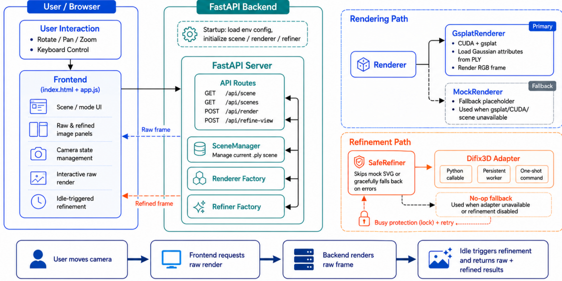
Figure 1: System overview of the web-based 3DGS viewer. The browser controls the camera and display state, while the backend performs raw 3DGS rendering and idle-time Difix3D+-based refinement.
