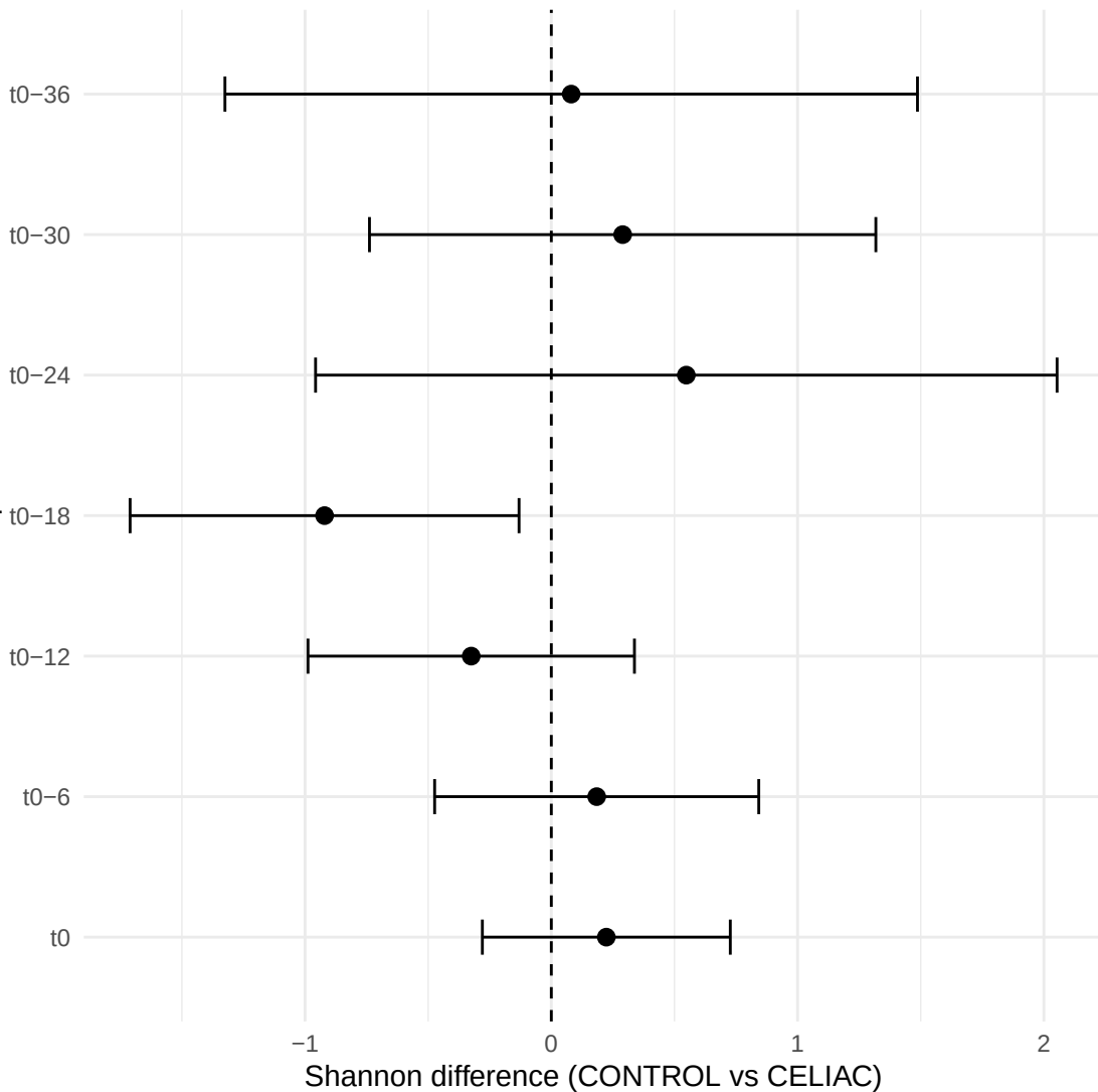
Italy Shannon diversity: per-timepoint difference with 95% CI
