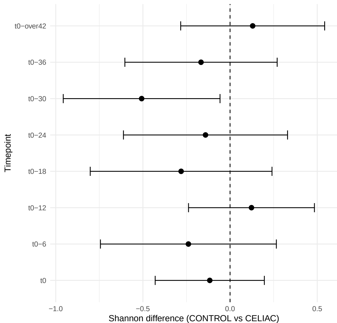
Total Shannon diversity: per-timepoint difference with 95% CI
