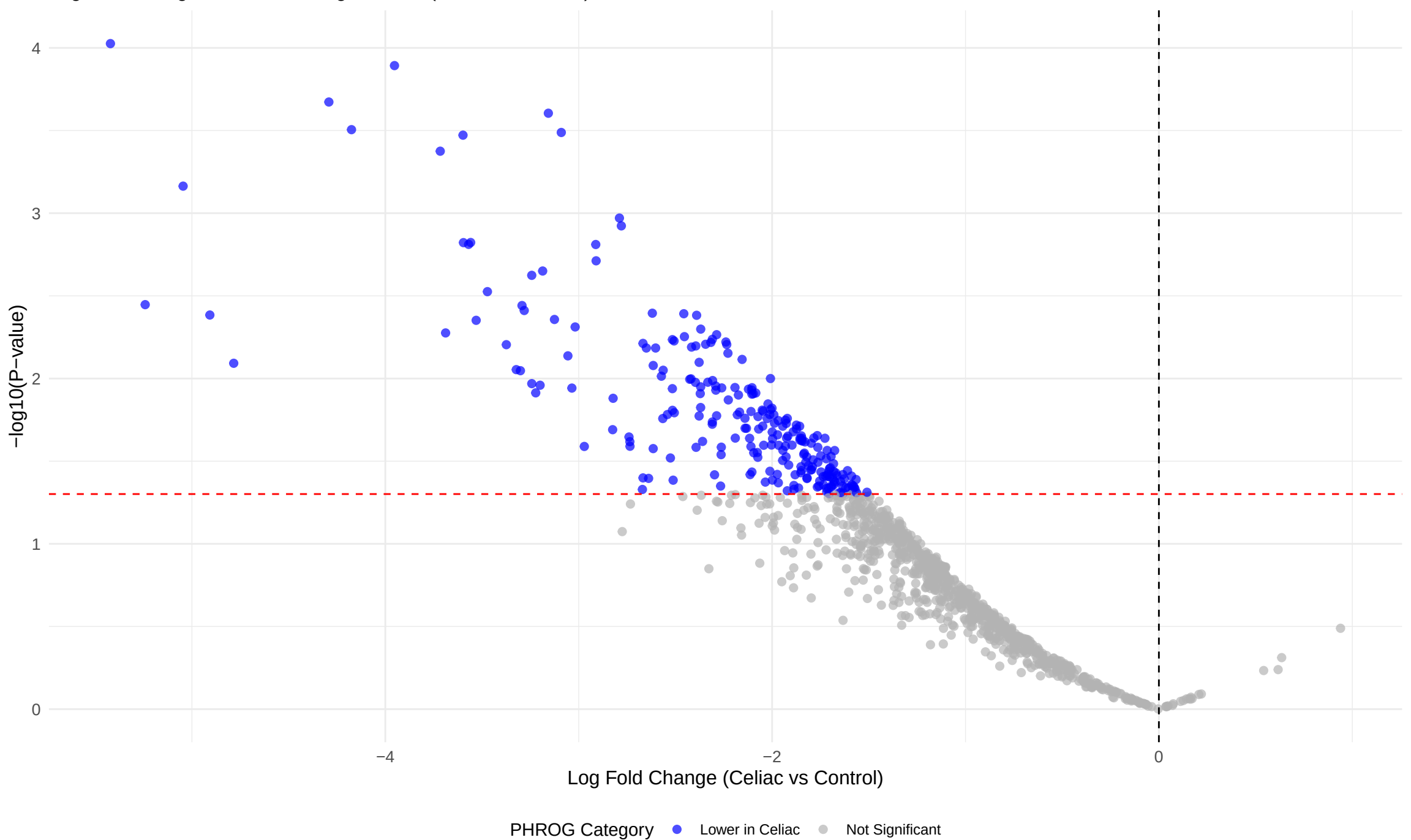
PHROG Abundance Analysis: Volcano Plot Log Fold Change vs Statistical Significance (Celiac vs Control)
