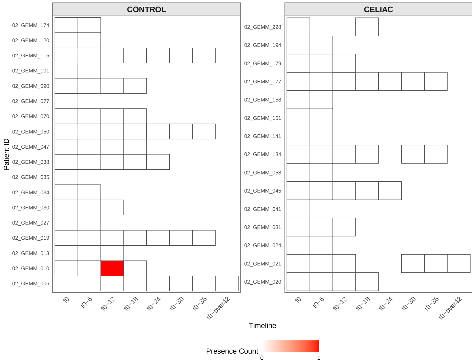
Presence/Absence of contig_8111
