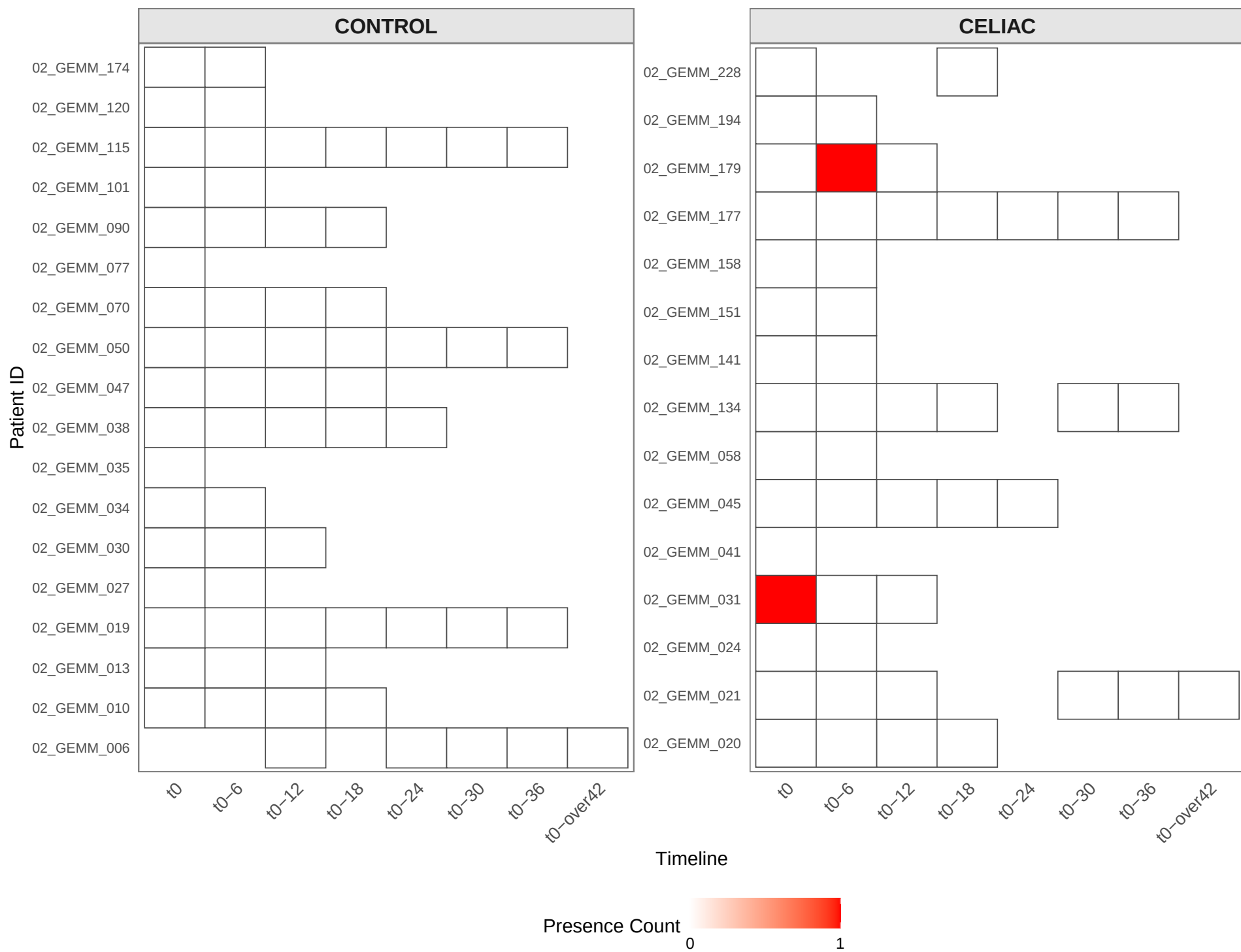
Presence/Absence of contig_8612
