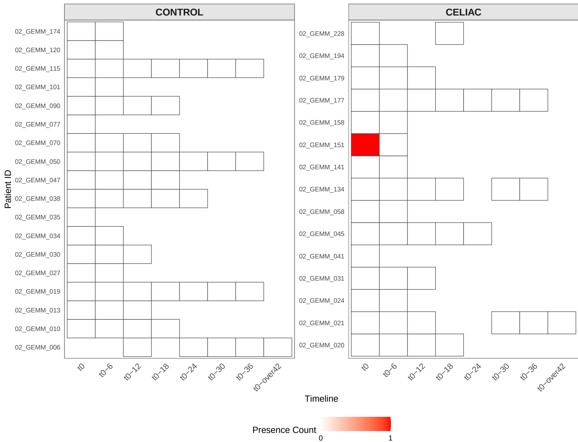
Presence/Absence of contig_8872
