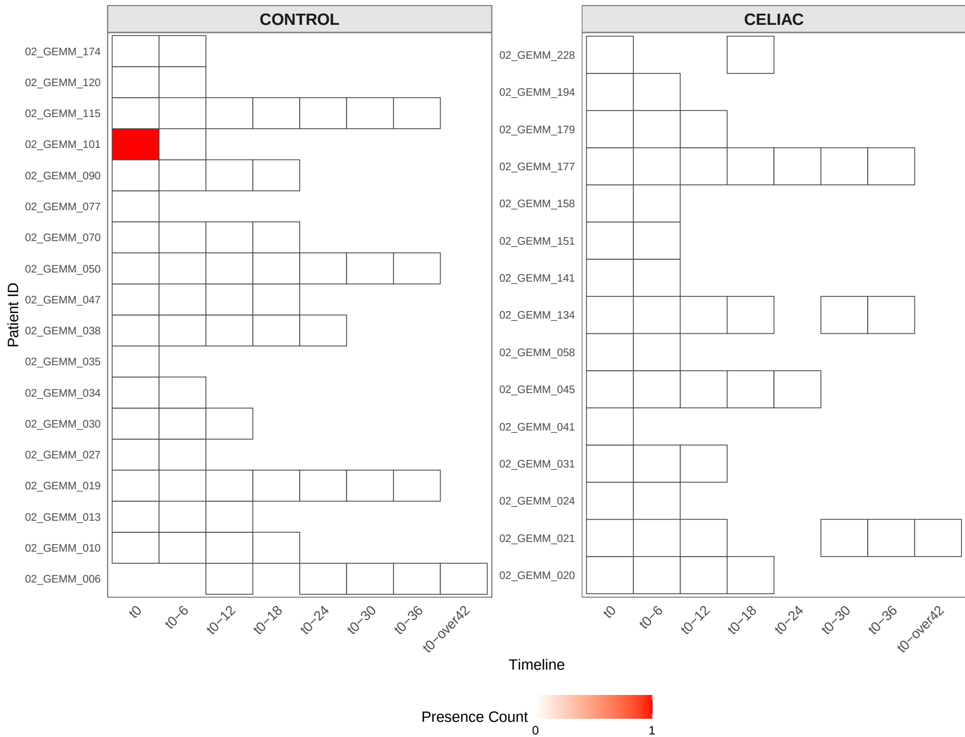
Presence/Absence of contig_9685
