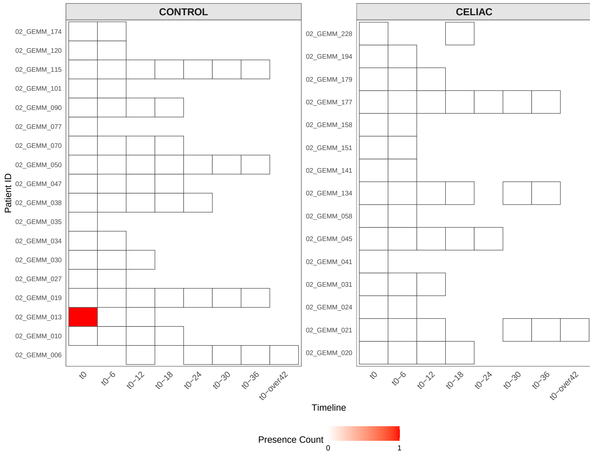
Presence/Absence of contig_3176
