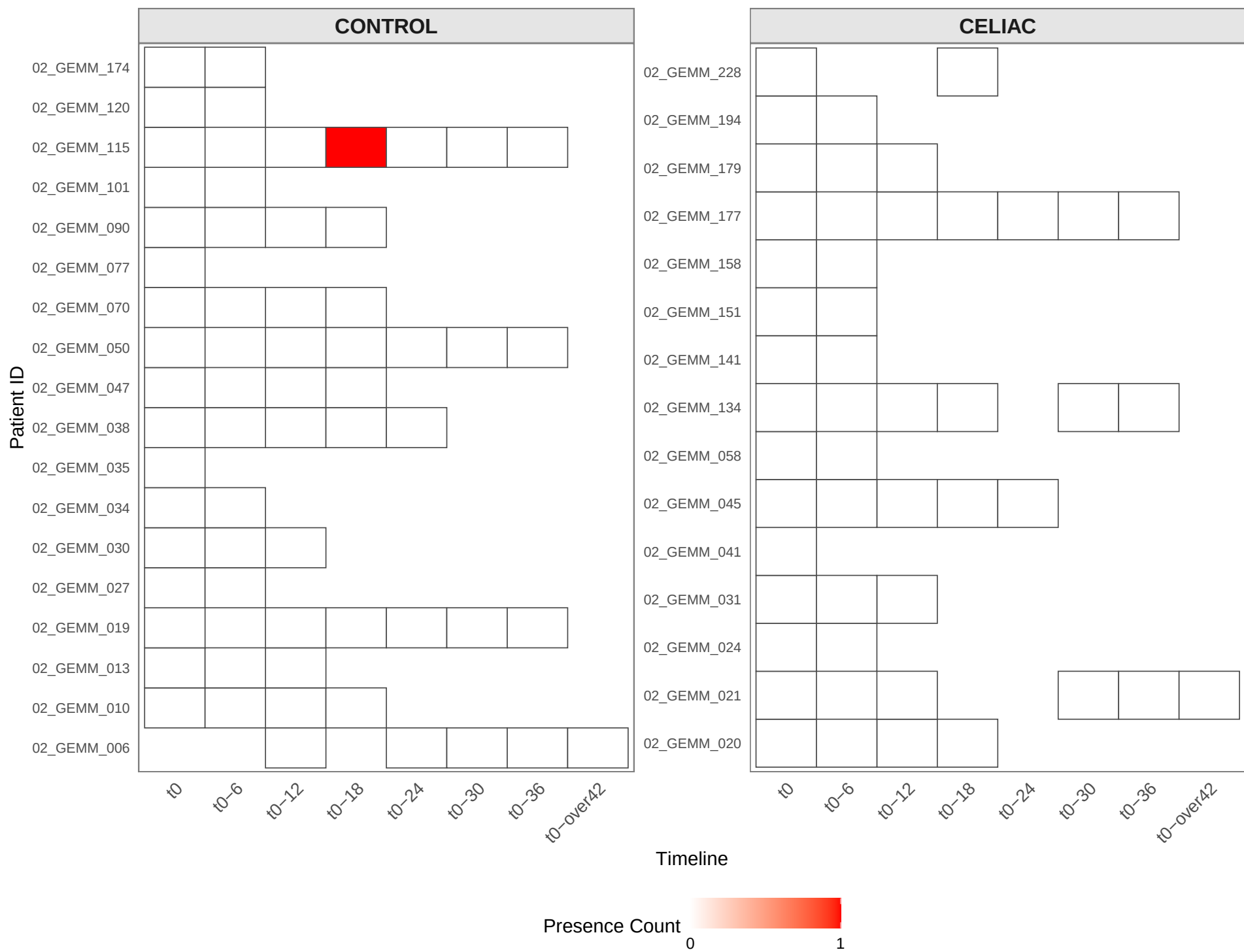
Presence/Absence of contig_9184
