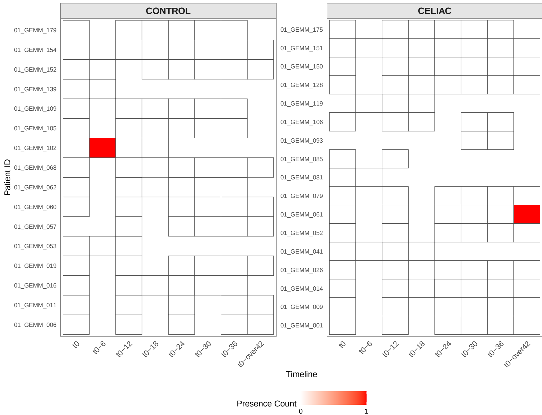
Presence/Absence of contig_2664
