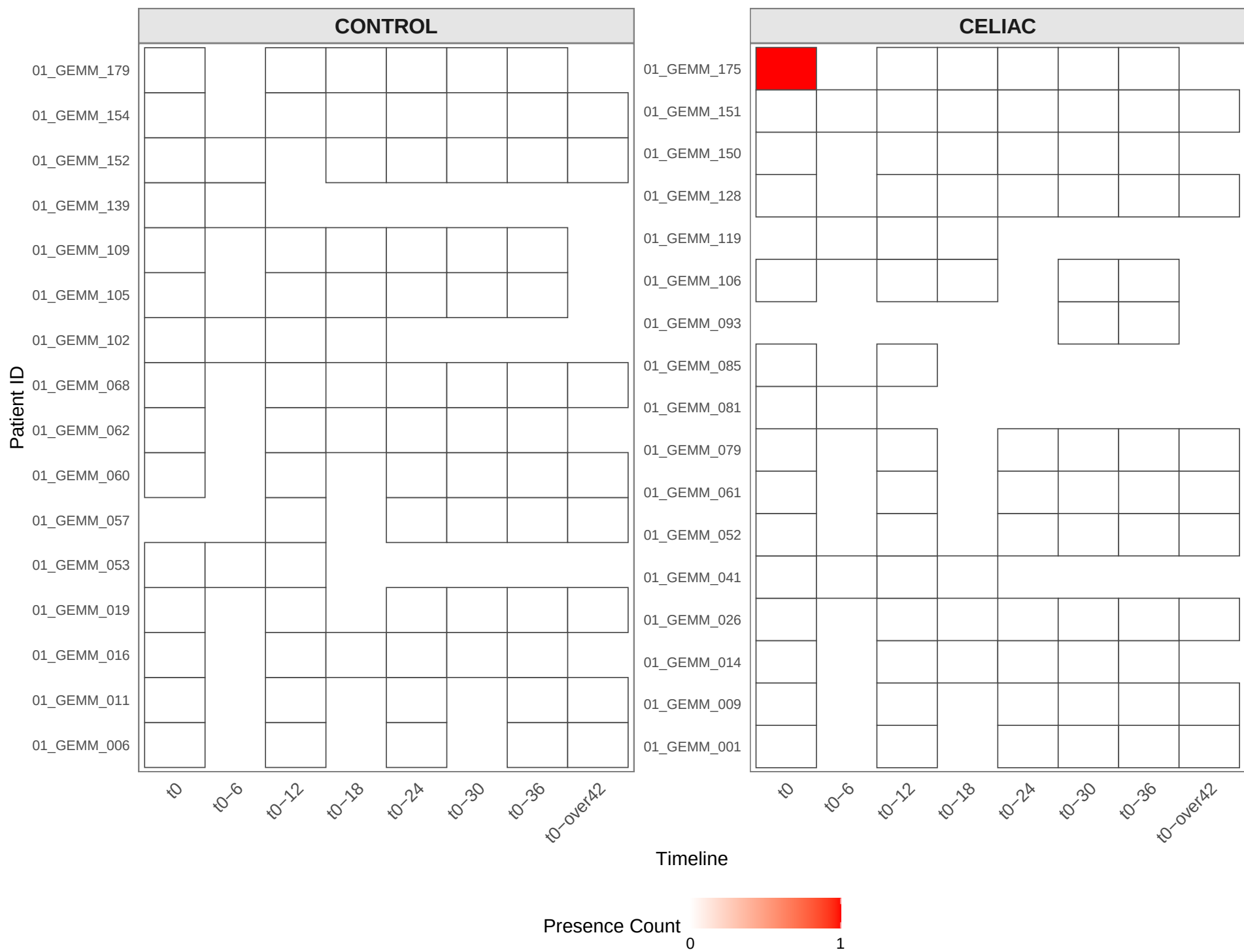
Presence/Absence of contig_43766
