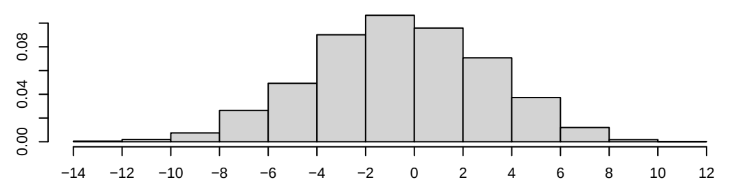
Density of edgecov.net_1lm25
