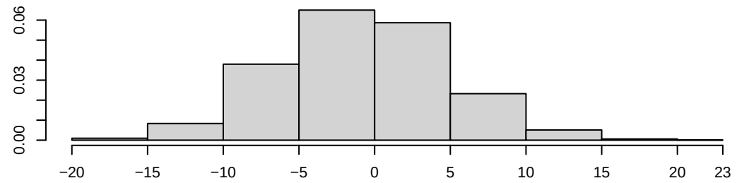
Density of mutual
