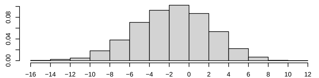
Density of edgecov.net_raw25
