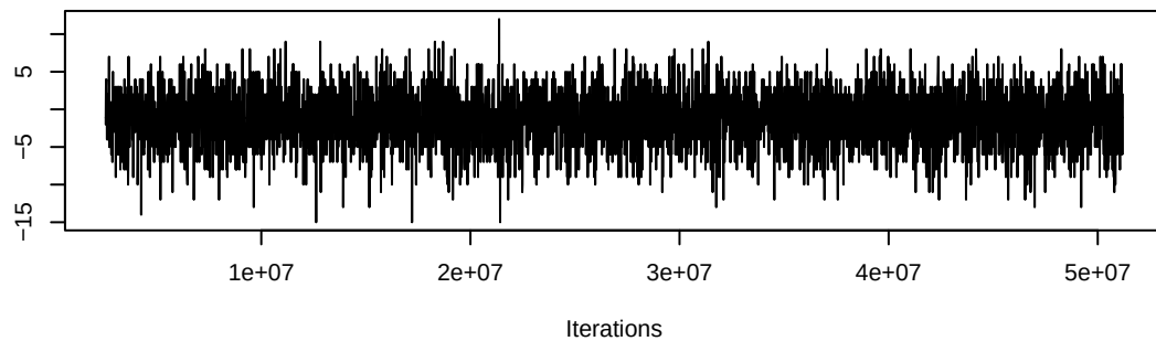
Trace of edgecov.net_raw25
