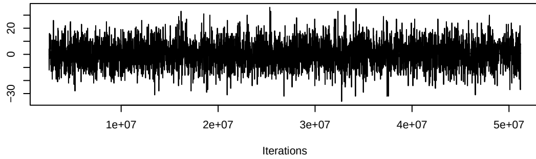
Trace of edges
