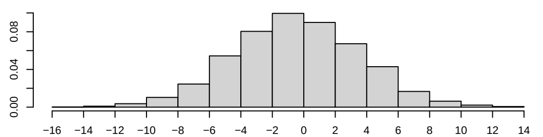
Density of nodematch.category
