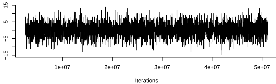
Trace of nodematch.category
