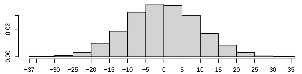
Density of edges
