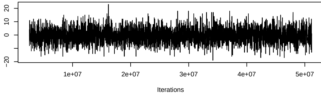
Trace of mutual
