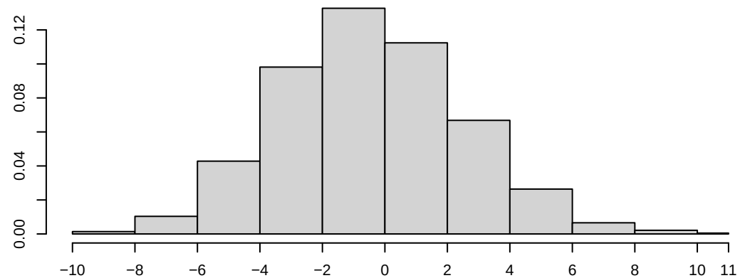
Density of nodeifactor.category.sectoral
