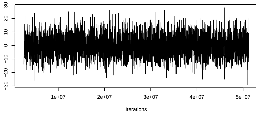
Trace of edges
