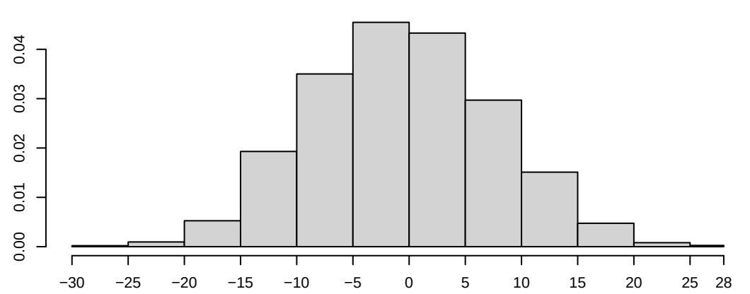
Density of edges
