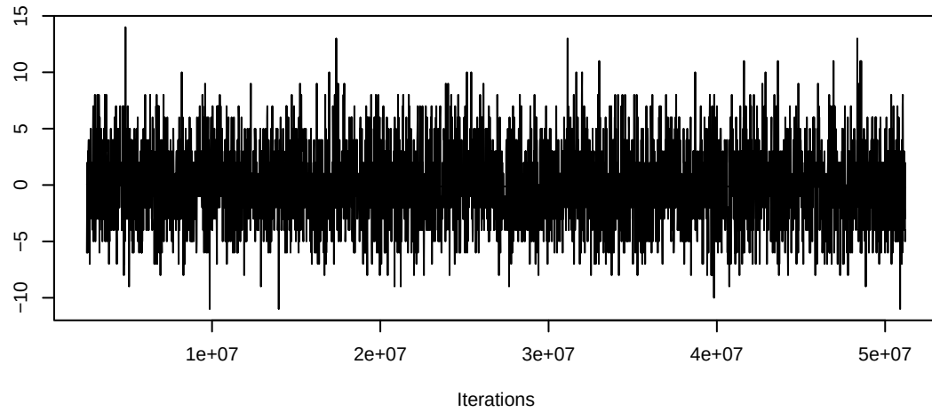
Trace of mutual
