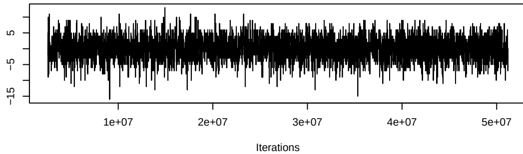
Trace of edgecov.net_1lm2425
