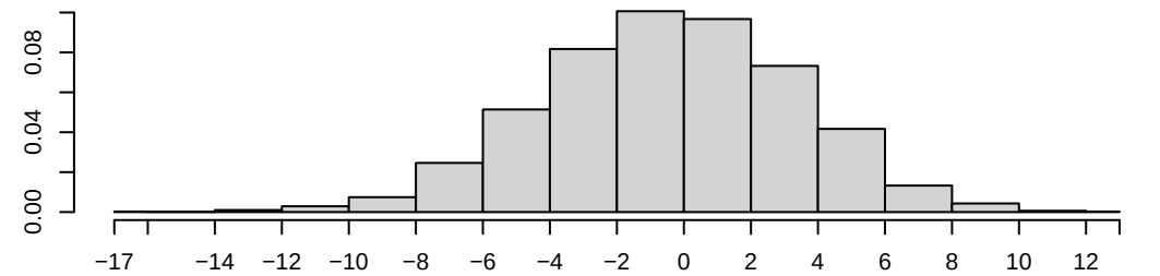
Density of edgecov.net_1lm2425
