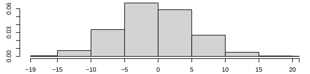
Density of mutual
