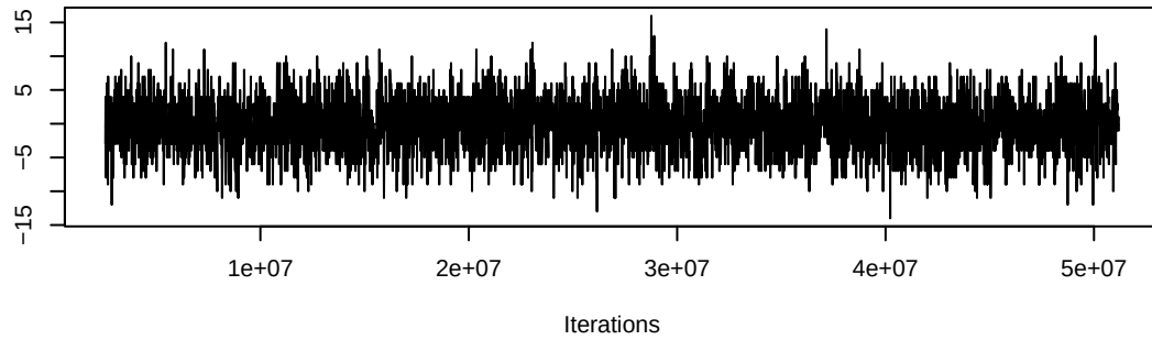
Trace of nodematch.category
