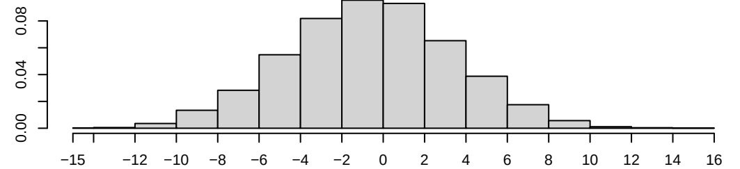
Density of nodematch.category
