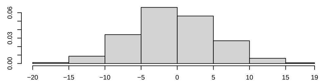
Density of mutual
