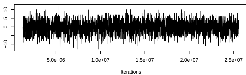
Trace of edgecov.net_1lm25
