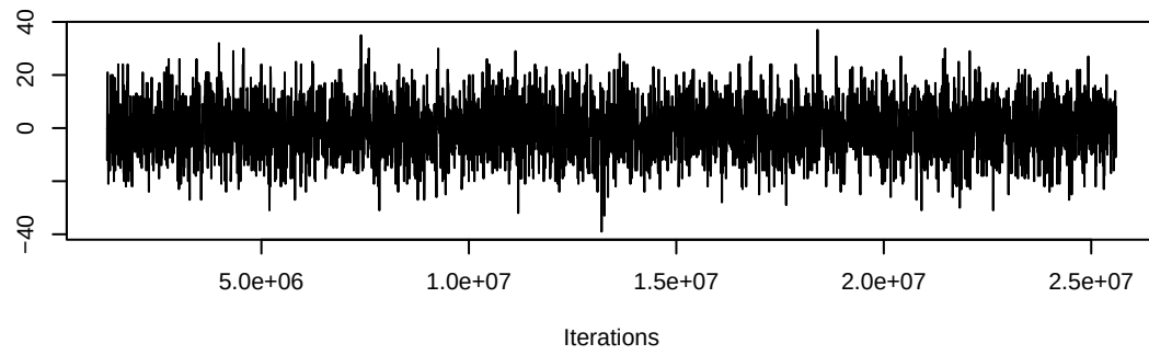
Trace of edges
