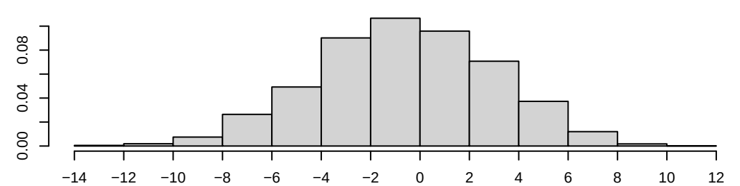
Density of edgecov.net_1lm25
