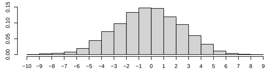
Density of nodeifactor.category.umbrella
