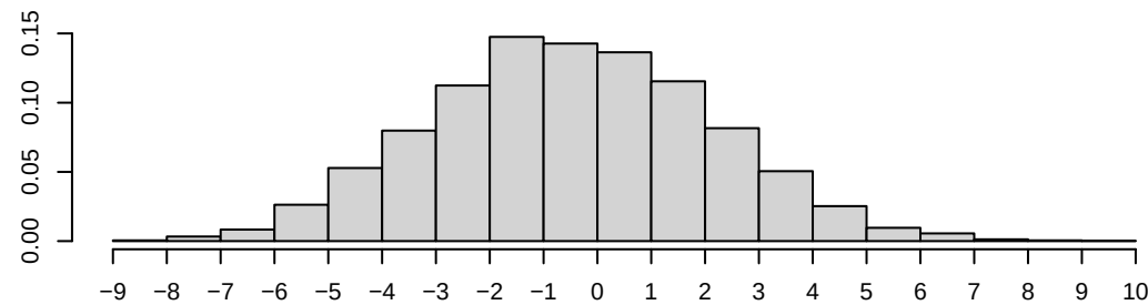
Density of nodematch.category.specialist
