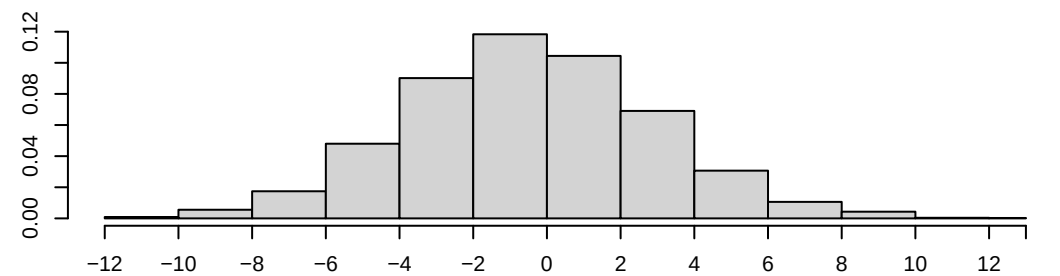
Density of nodeofactor.category.radical
