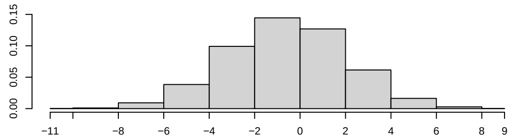
Density of nodematch.category.advocacy
