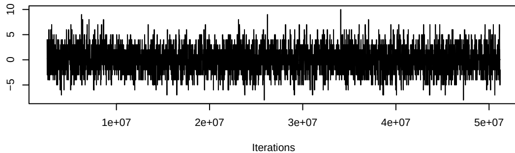
Trace of nodematch.category.specialist
