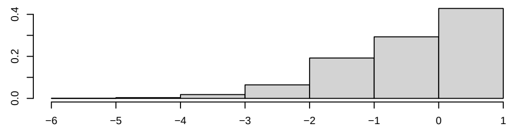
Density of nodematch.category.radical
