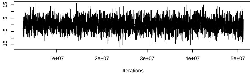
Trace of nodeifactor.category.specialist
