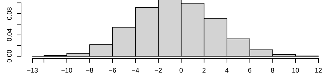
Density of nodeifactor.category.sectoral
