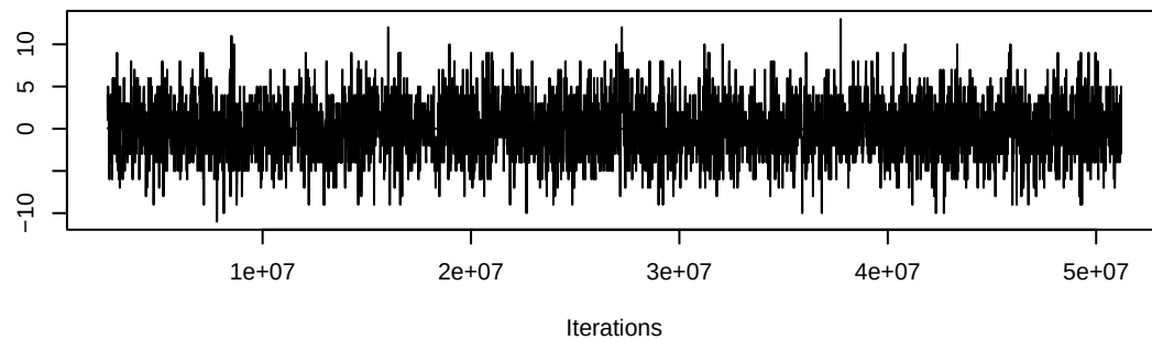
Trace of nodeofactor.category.radical
