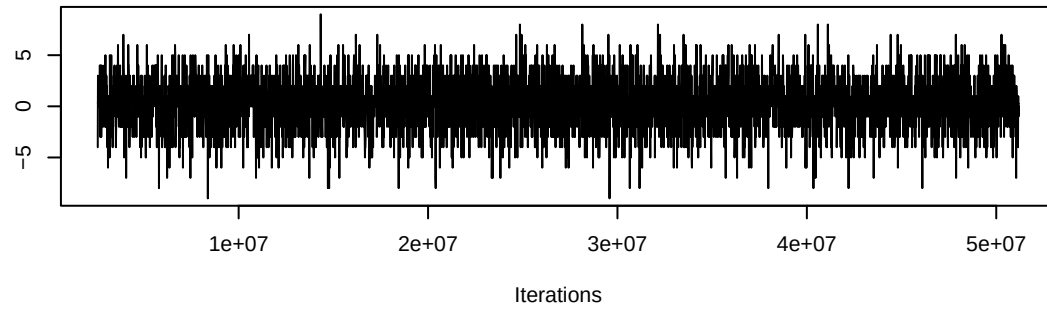
Trace of nodeifactor.category.umbrella
