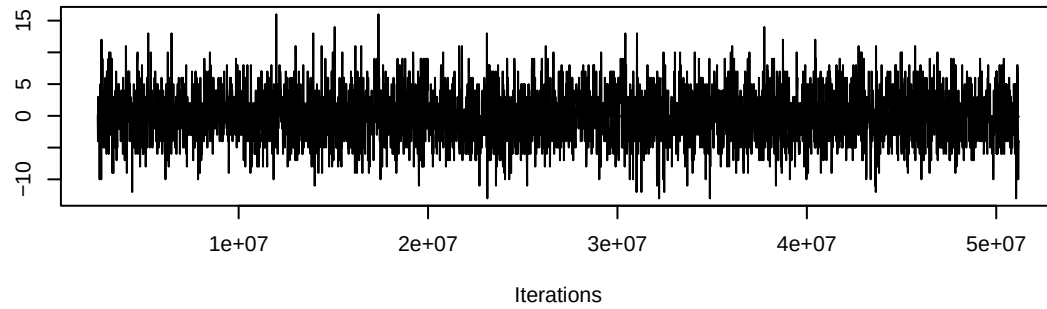
Trace of nodeofactor.category.specialist
