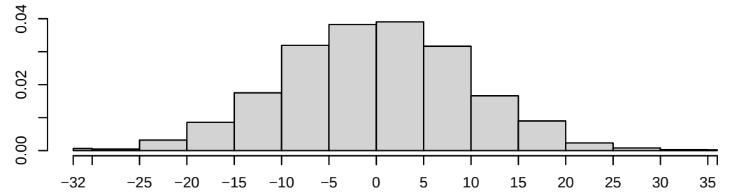
Density of edges
