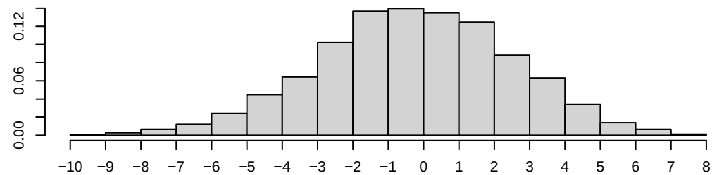
Density of nodefactor.category.umbrella
