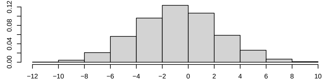
Density of nodeifactor.category.radical
