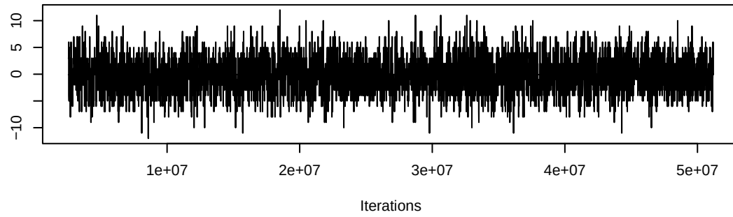
Trace of nodeifactor.category.sectoral
