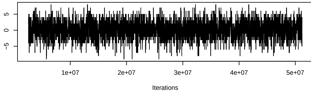
Trace of nodefactor.category.umbrella
