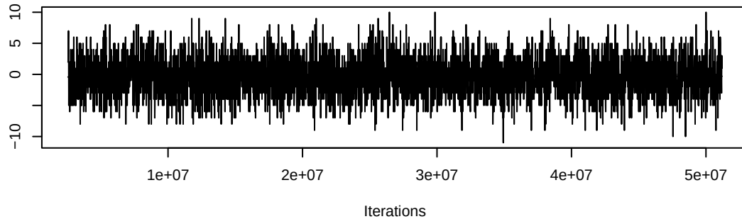
Trace of nodeifactor.category.radical
