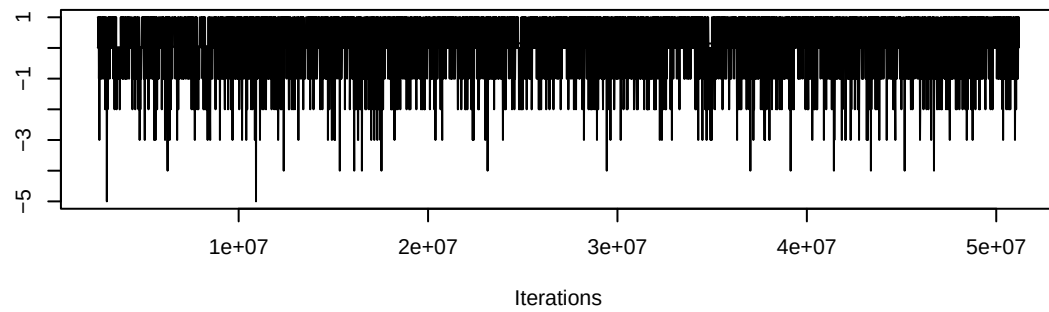
Trace of nodematch.category.radical
