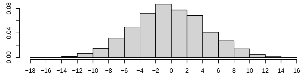
Density of nodeifactor.category.specialist
