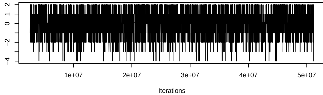
Trace of nodematch.category.sectoral
