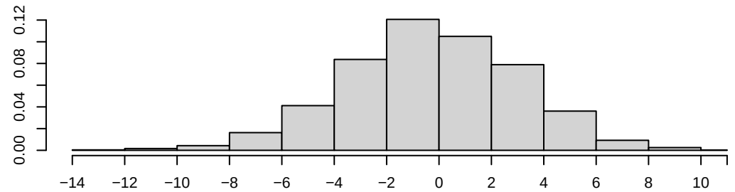
Density of nodefactor.category.sectoral
