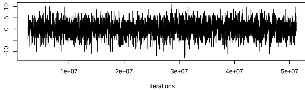
Trace of nodefactor.category.sectoral
