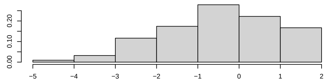
Density of nodematch.category.sectoral
