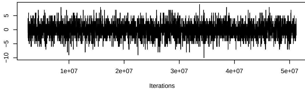
Trace of nodematch.category.advocacy
