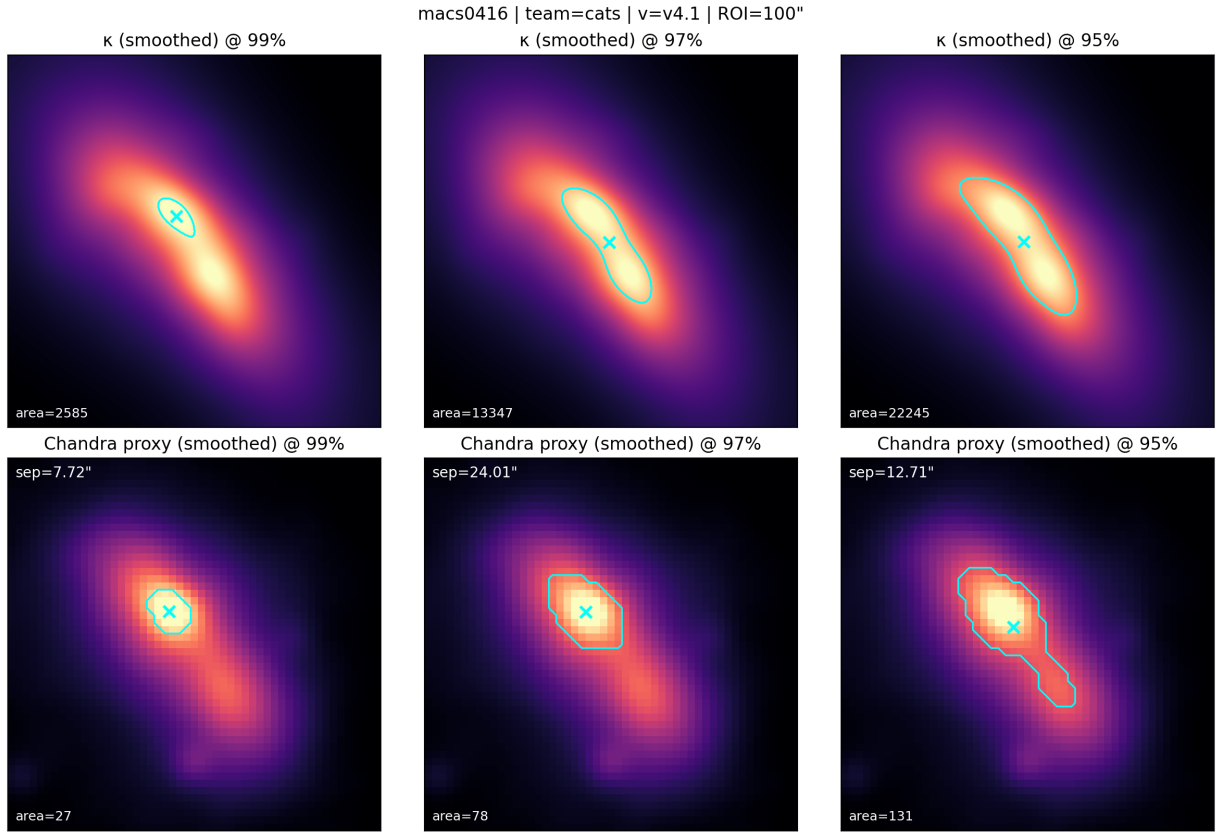
Figure 9: Figure 8. MACS J0416.1–2403 (CATS v4.1), ROI = 100".
