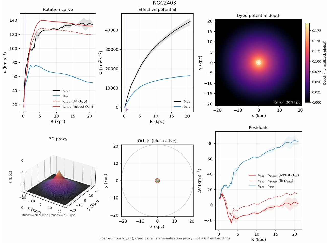
Figure 3: NGC 2403—a well-resolved, intermediate-mass spiral. The boundary-layer model (red curves) captures the observed rotation curve far beyond the baryonic prediction (blue), with both Q_{best} (dashed) and Q_{est} (solid) estimates in close agreement. The residual panel (lower right) shows the velocity deficit (blue) reduced to near-zero by the model.
