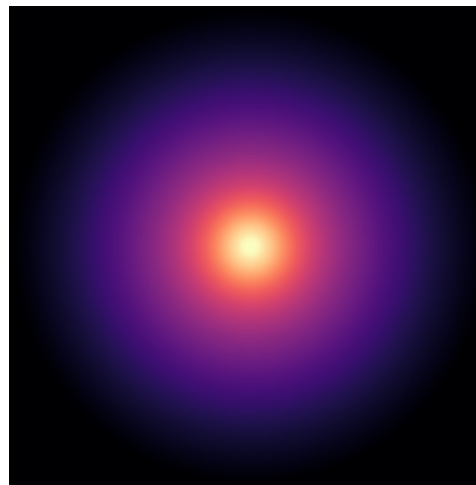
IC4202
