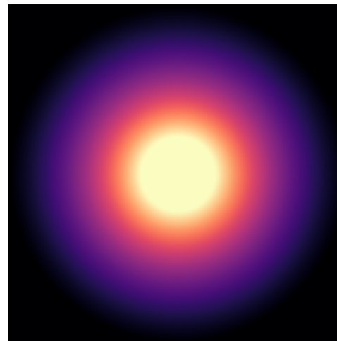
NGC4013
