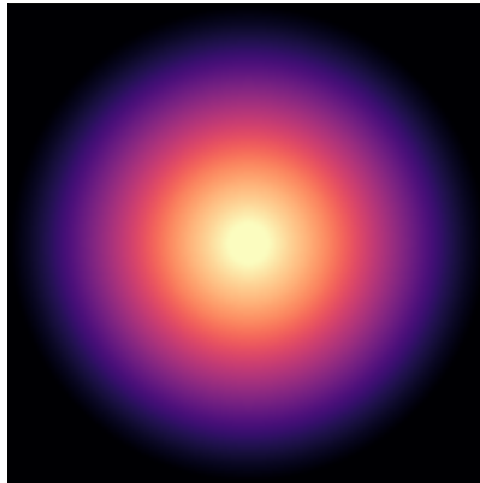
NGC4085
