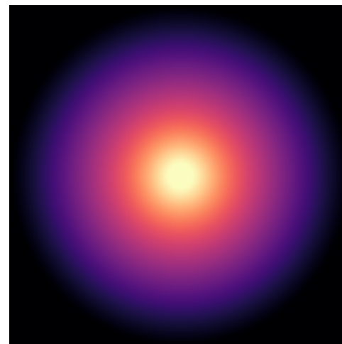
NGC0247
