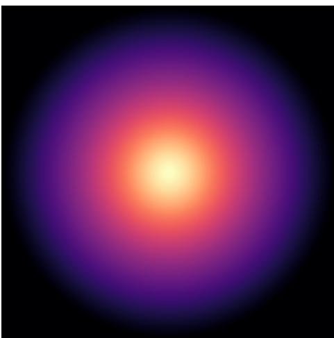
NGC0024
