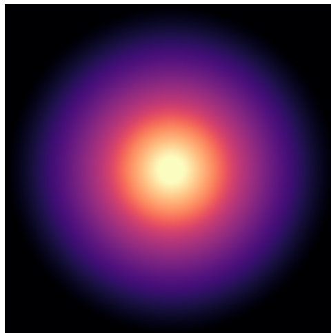
NGC1090
