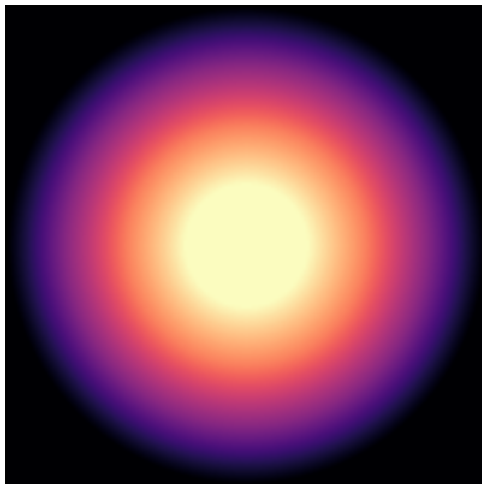
UGC07524
