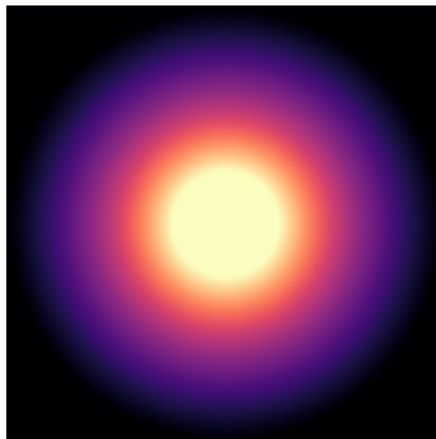
NGC4010
