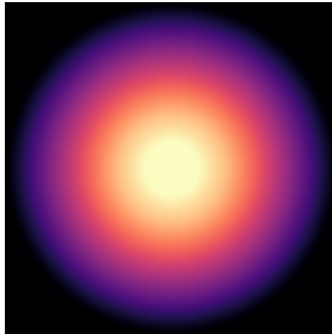
NGC5055
