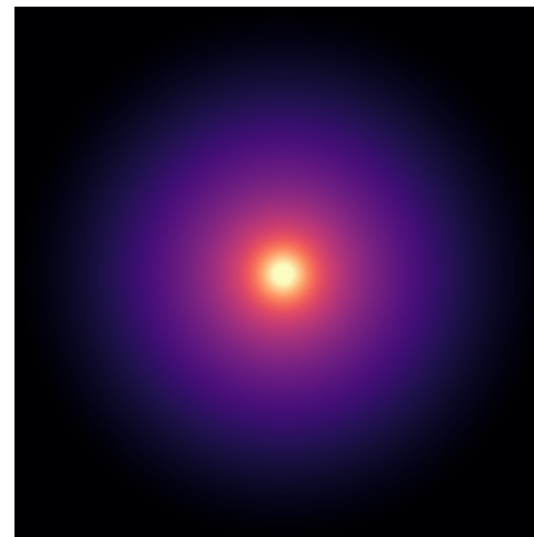
NGC6946
