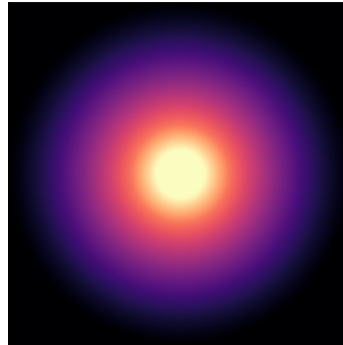
NGC4100
