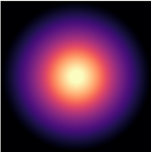
UGC07603
