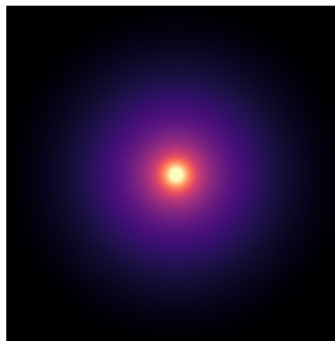
UGC11557
