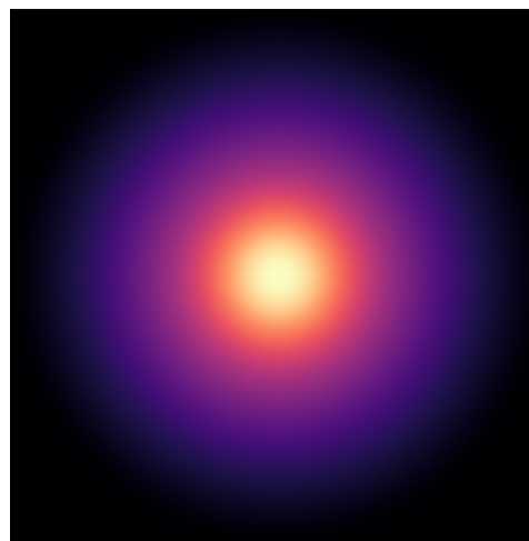
NGC0100
