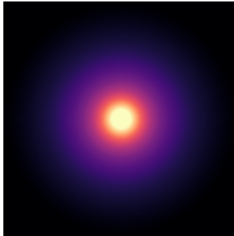
NGC2683
