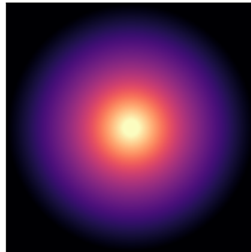
UGC12732
