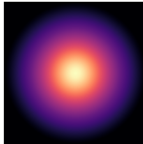
KK98-251
