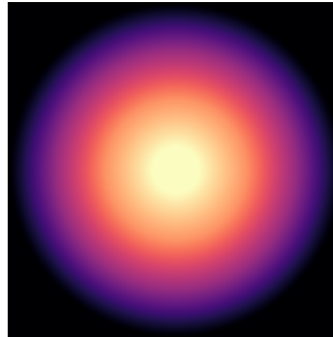
NGC7814
