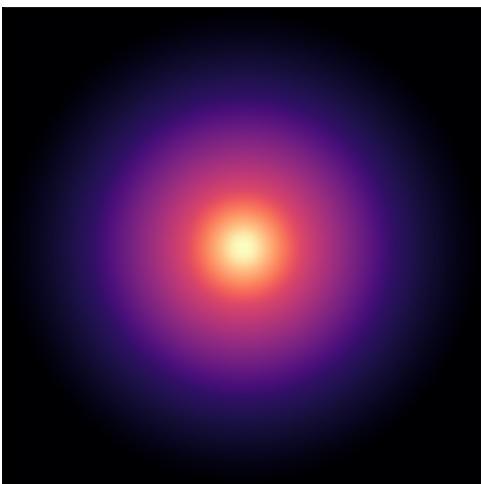
NGC0024
