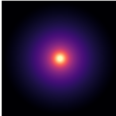
NGC7793
