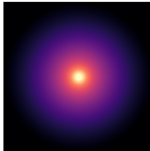
NGC5005
