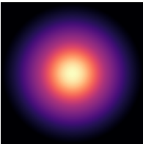
F568-3
