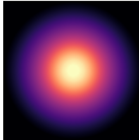
NGC3877
