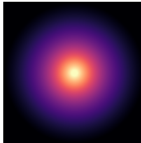
NGC4559
