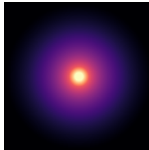
NGC2366
