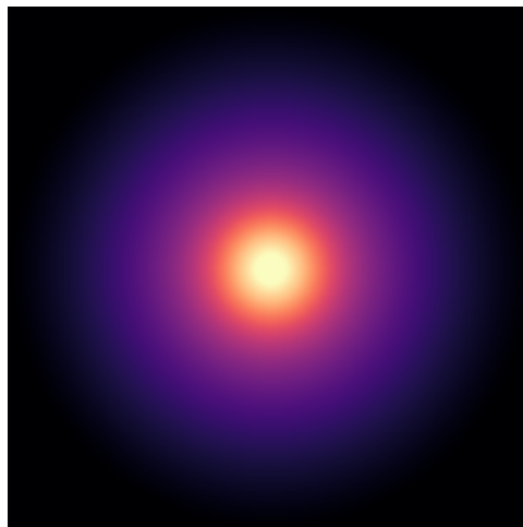
NGC4389
