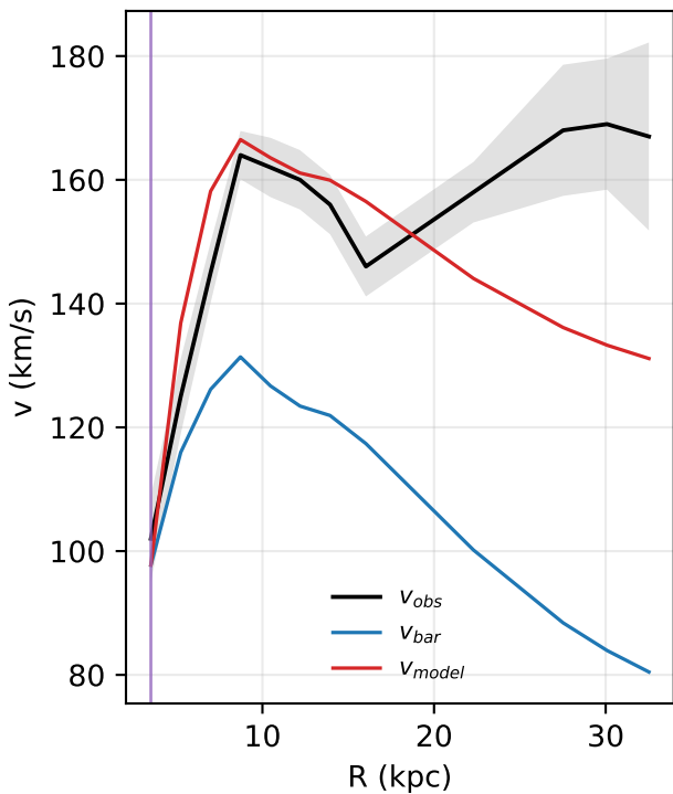
NGC3726: rotation curve
