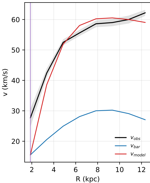
DDO170: rotation curve
