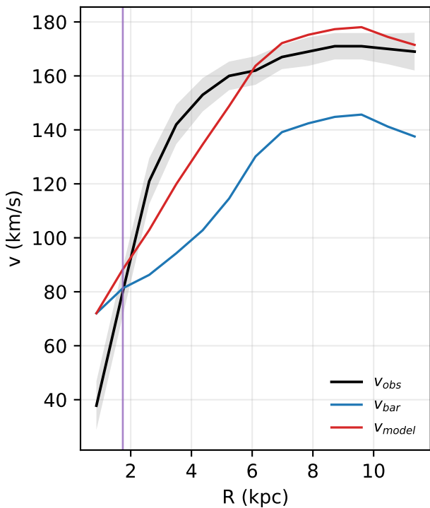
NGC3877: rotation curve
