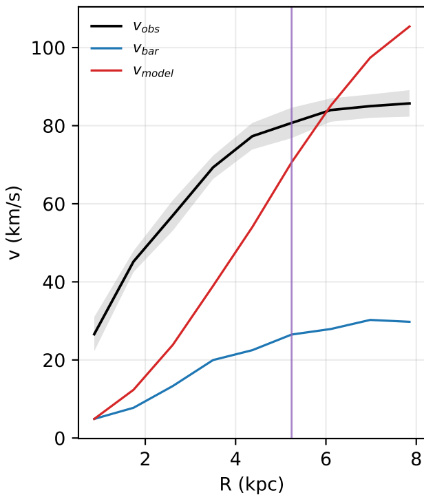
UGC06667: rotation curve
