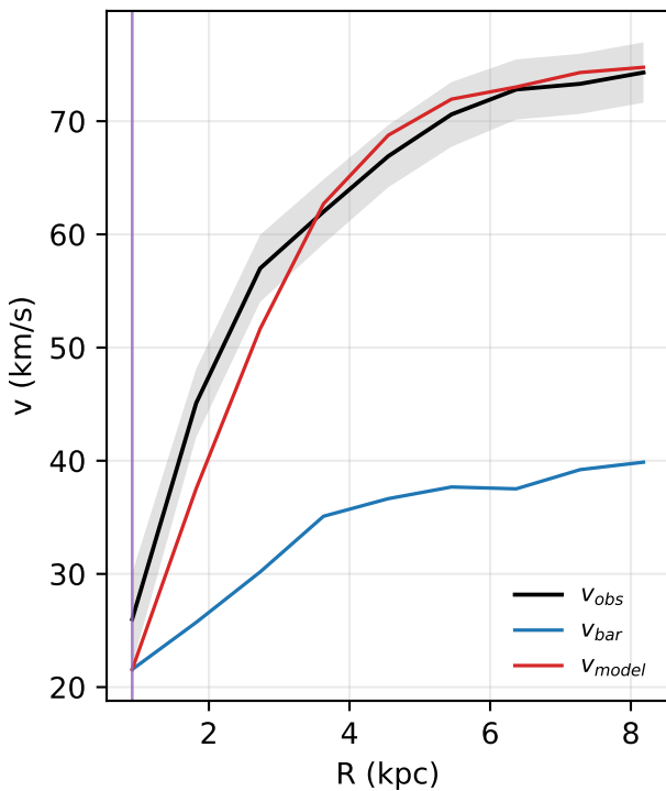
UGC04499: rotation curve
