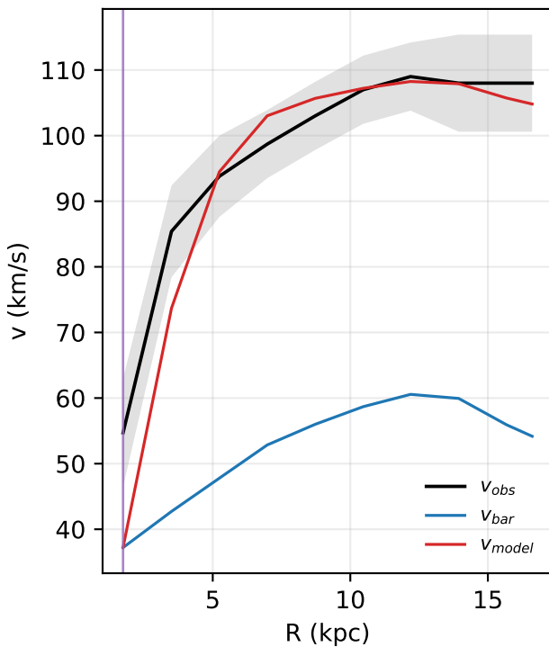
UGC06930: rotation curve
