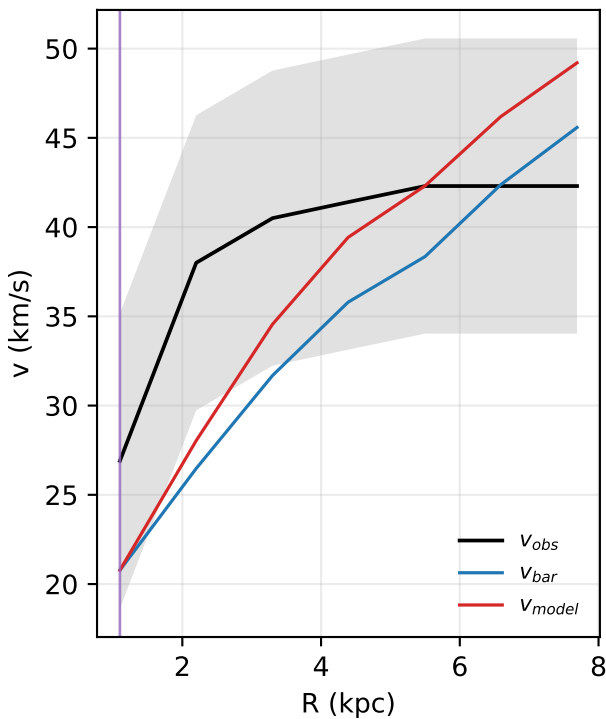
UGC06628: rotation curve
