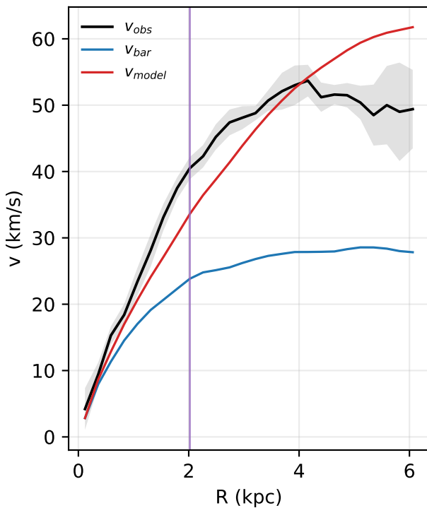
NGC2366: rotation curve
