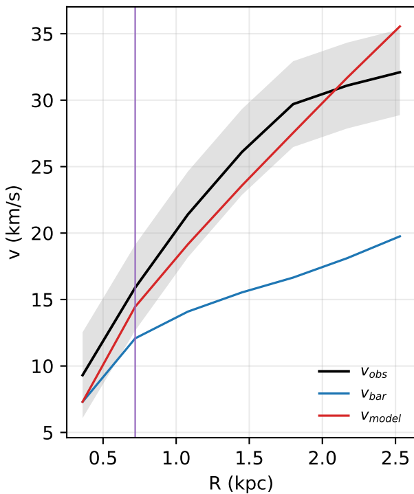
UGC07559: rotation curve
