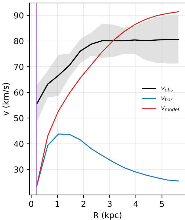
NGC4214: rotation curve
