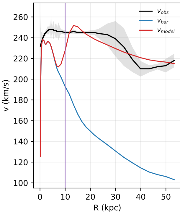
UGC05253: rotation curve
