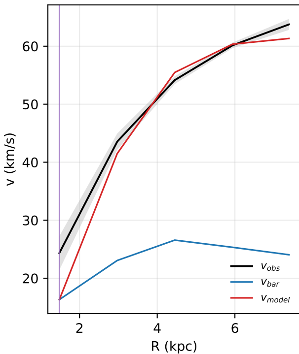
UGC00891: rotation curve
