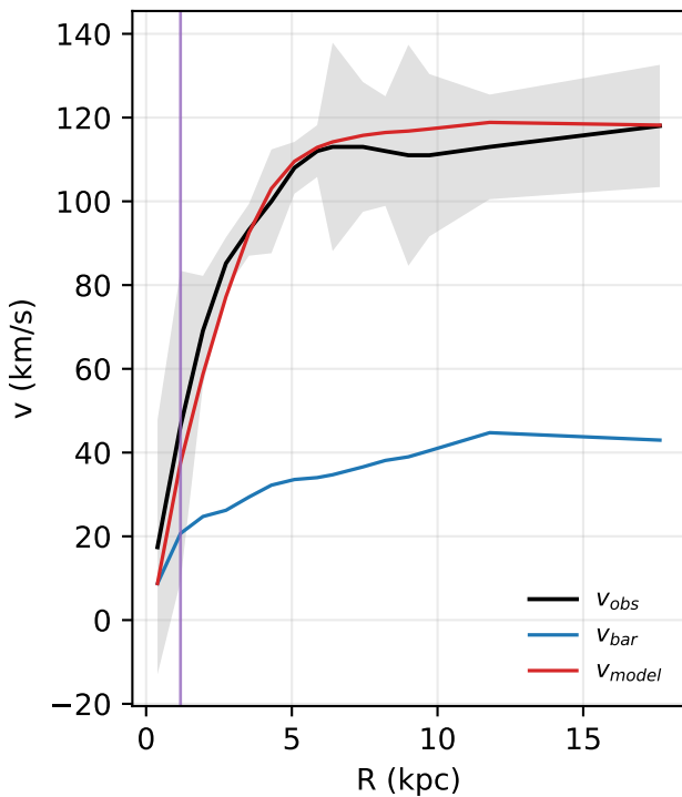
F568-V1: rotation curve
