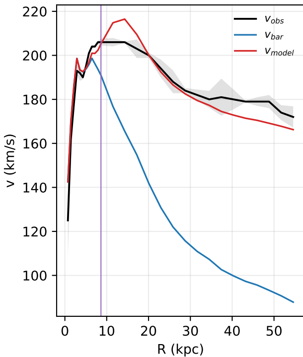
NGC5055: rotation curve
