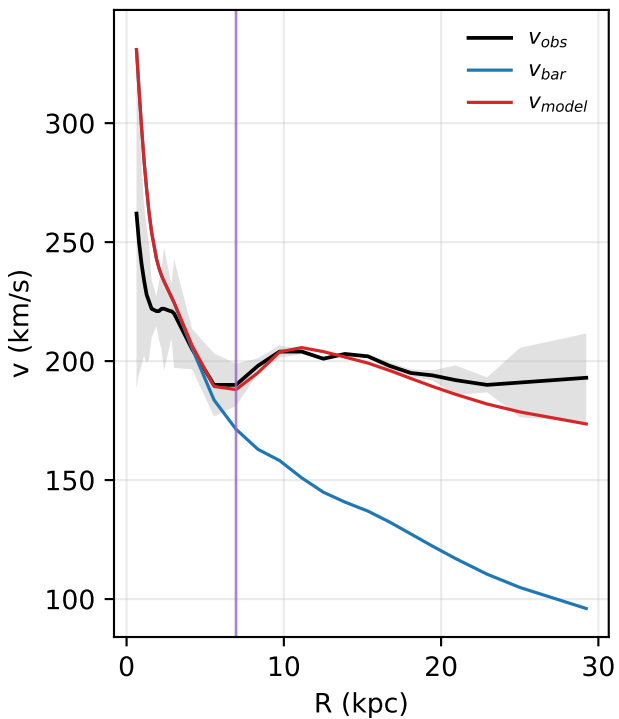
UGC03546: rotation curve
