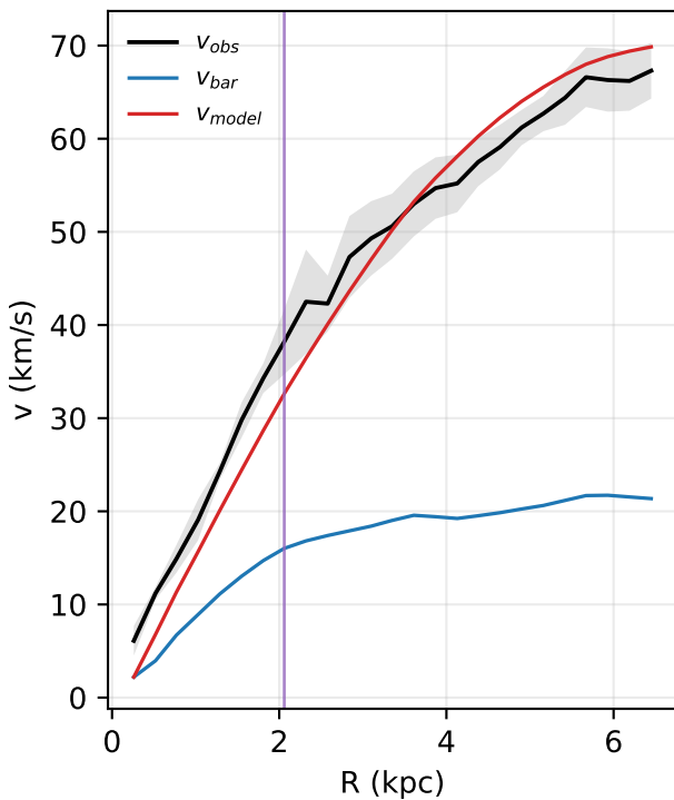
NGC3109: rotation curve
