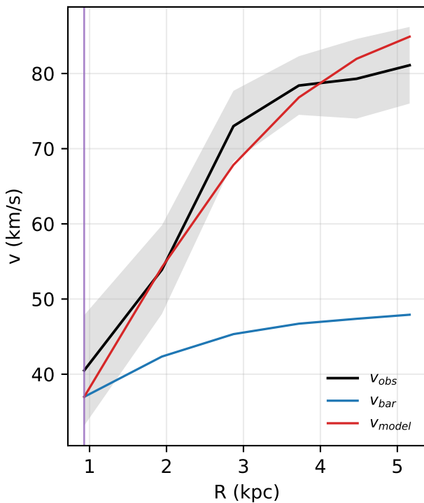
UGC06923: rotation curve
