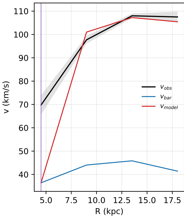
UGC00634: rotation curve
