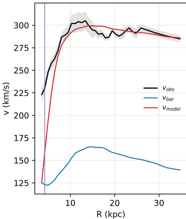
NGC5985: rotation curve
