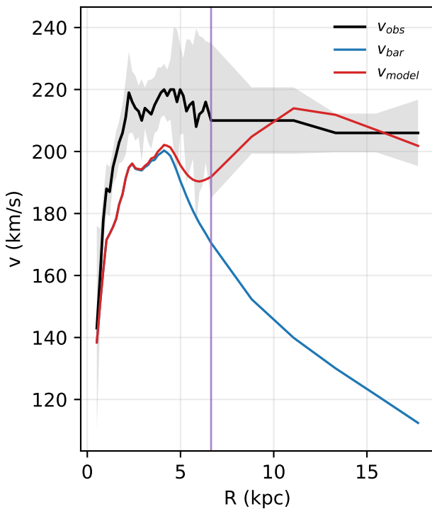
NGC3521: rotation curve
