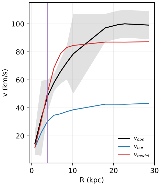
UGC05005: rotation curve
