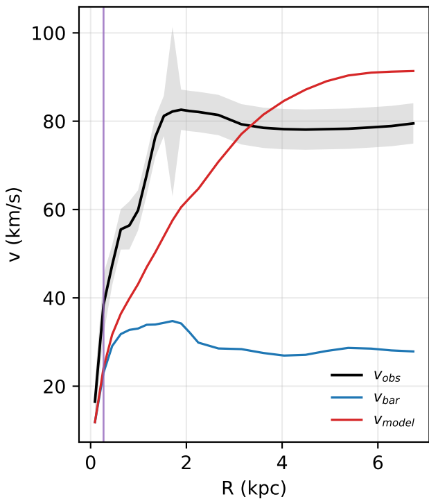
UGC05721: rotation curve
