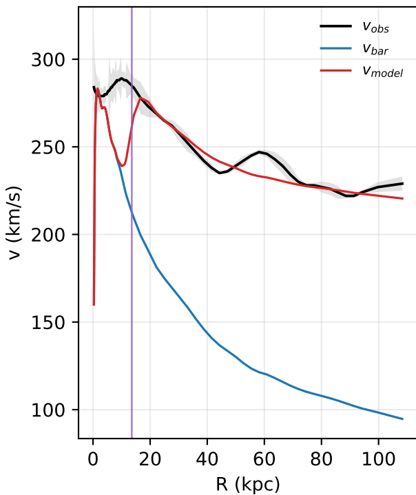
UGC09133: rotation curve
