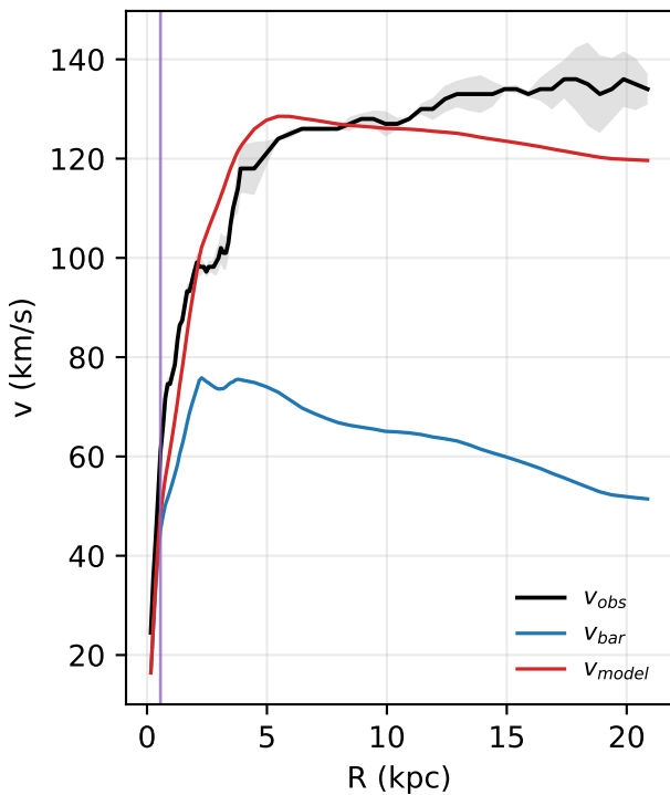
NGC2403: rotation curve
