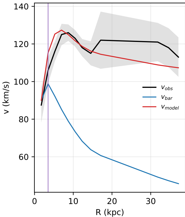
NGC3769: rotation curve
