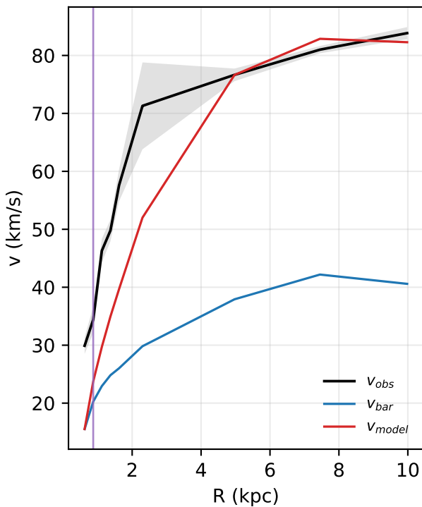
UGC00191: rotation curve
