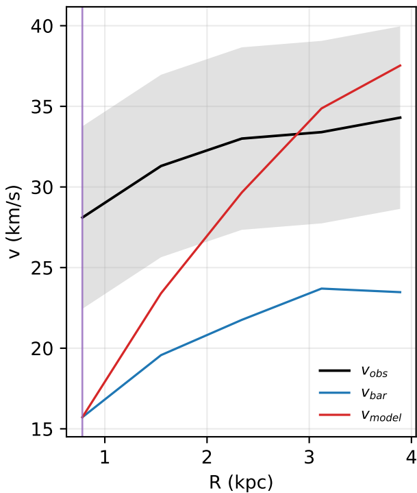
UGC09992: rotation curve
