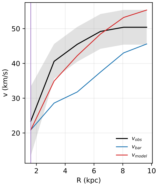
F561-1: rotation curve
