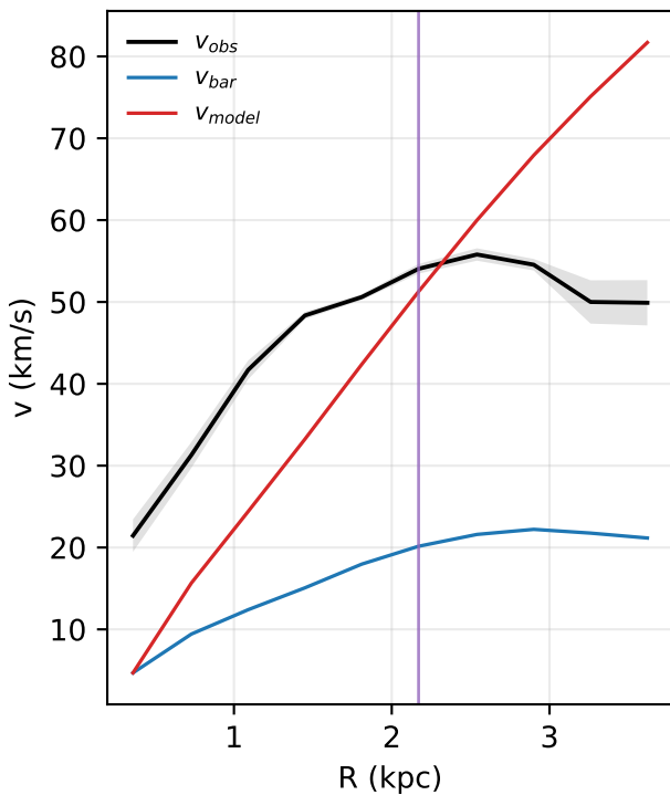
UGC05764: rotation curve
