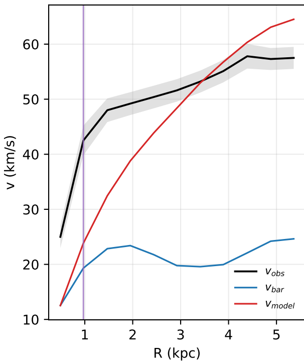
UGC08550: rotation curve
