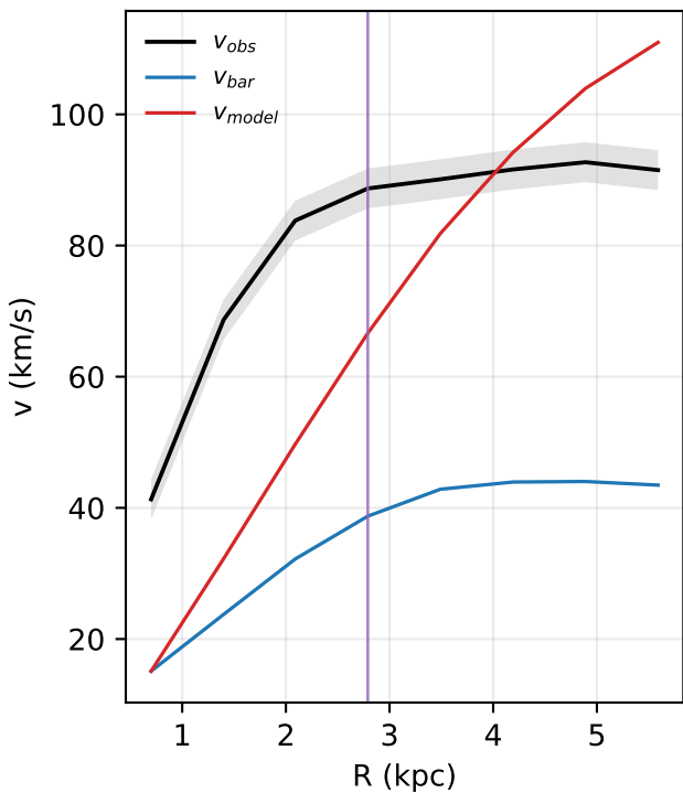
UGC04325: rotation curve
