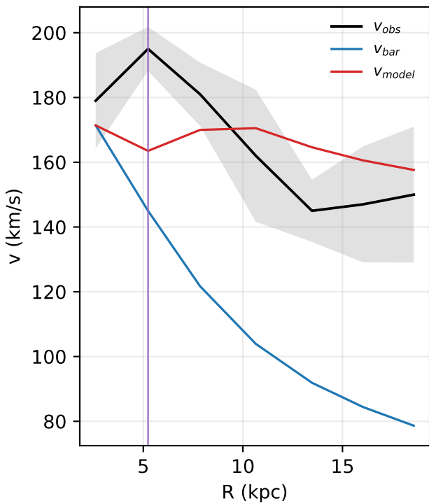
NGC4138: rotation curve
