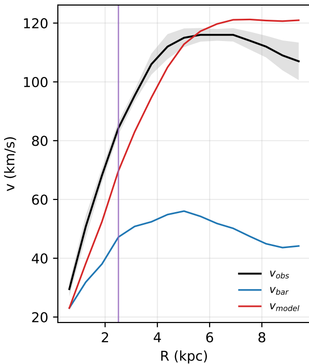
UGC05986: rotation curve
