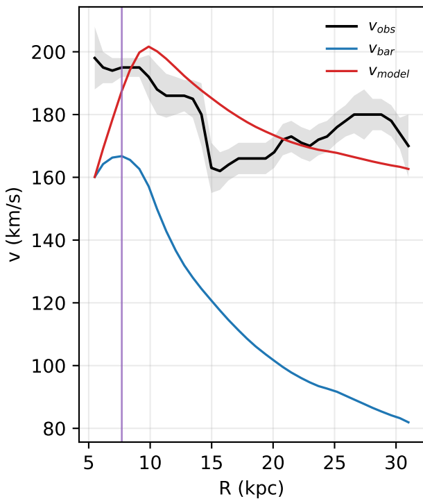
NGC4013: rotation curve
