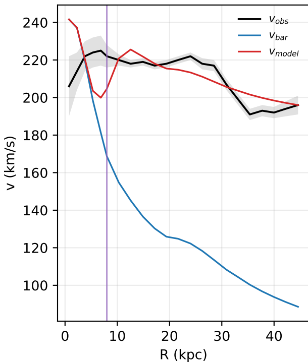
NGC5033: rotation curve
