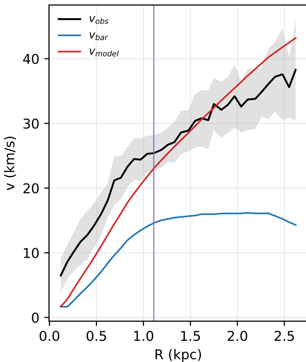
UGCA444: rotation curve
