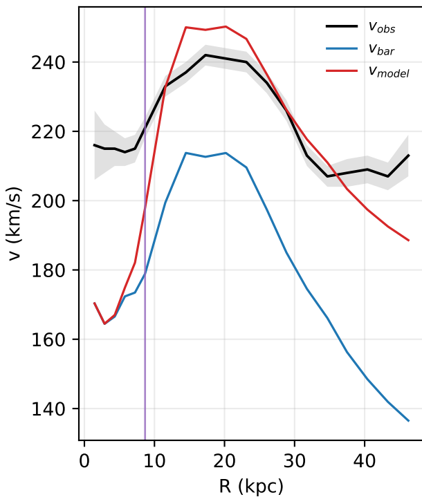
NGC5371: rotation curve
