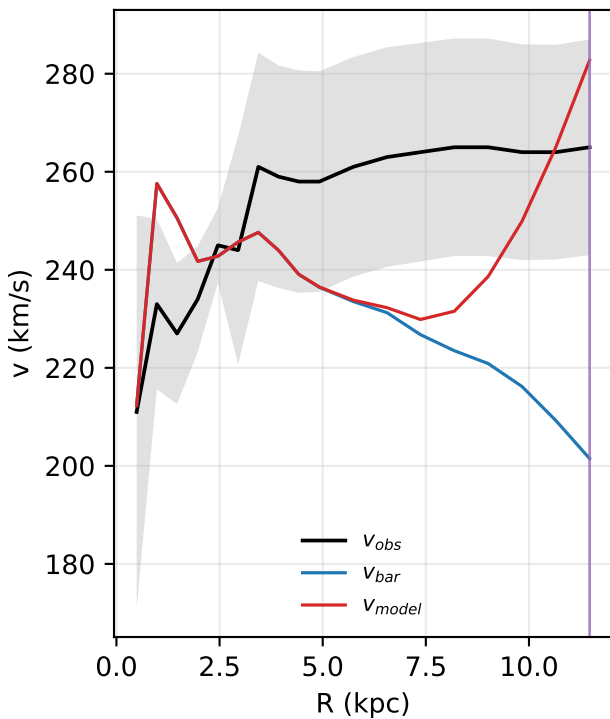
NGC5005: rotation curve
