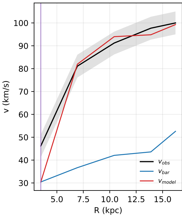
UGC05999: rotation curve
