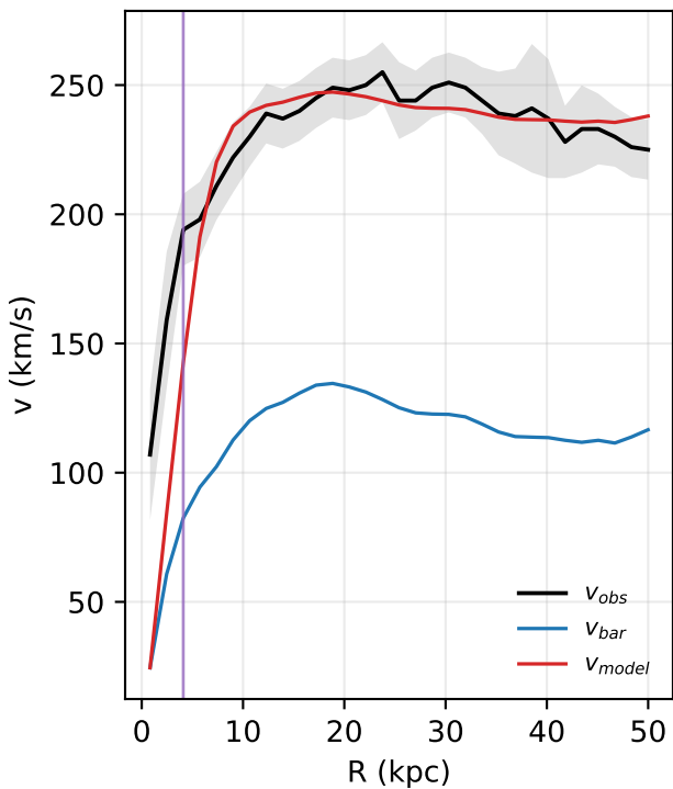
UGC12506: rotation curve
