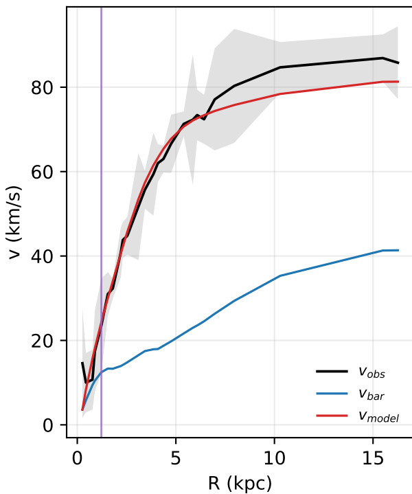
F583-1: rotation curve
