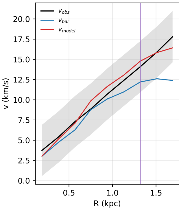
UGC07577: rotation curve
