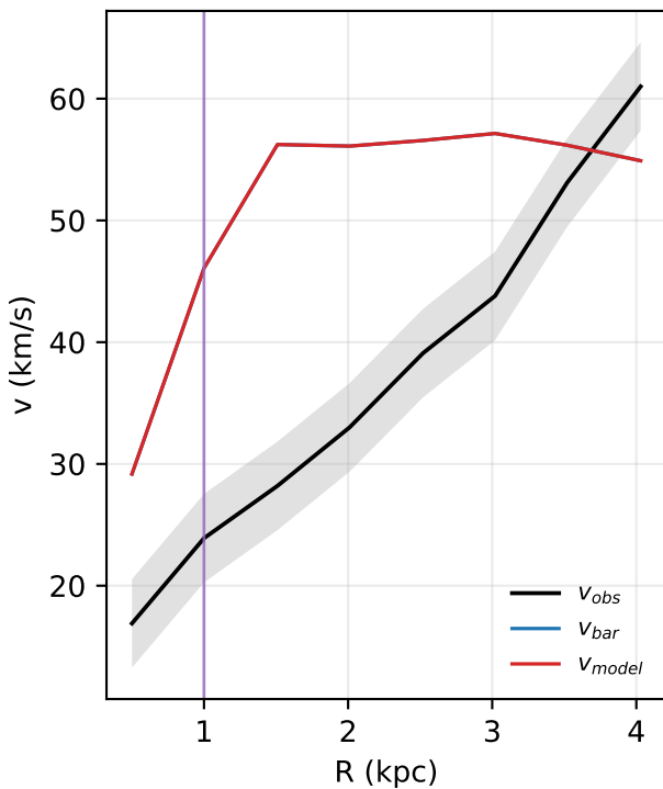
UGC02455: rotation curve
