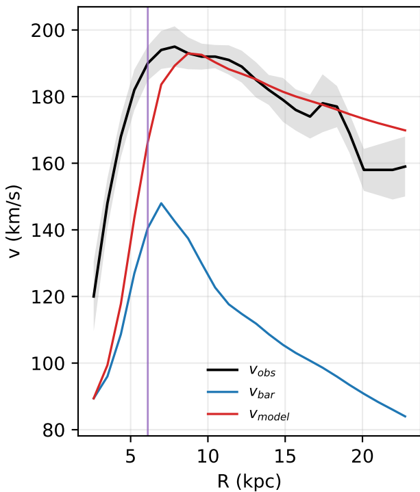
NGC4100: rotation curve
