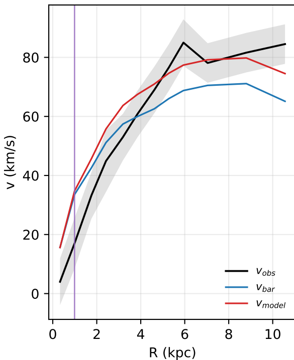
UGC11557: rotation curve
