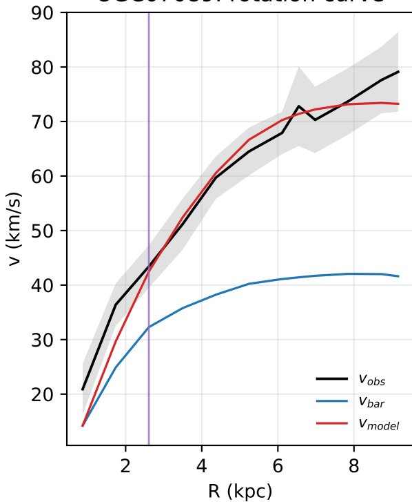
UGC07089: rotation curve
