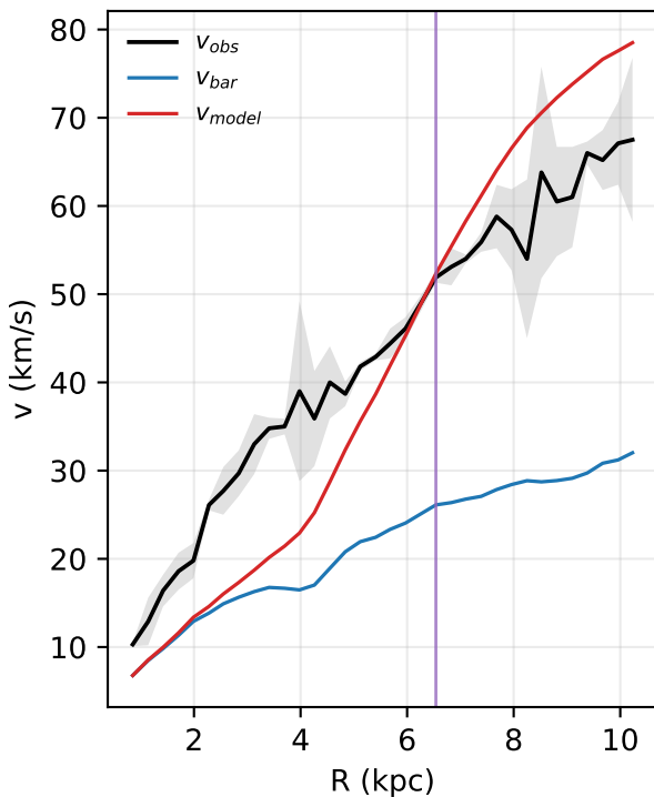
IC2574: rotation curve
