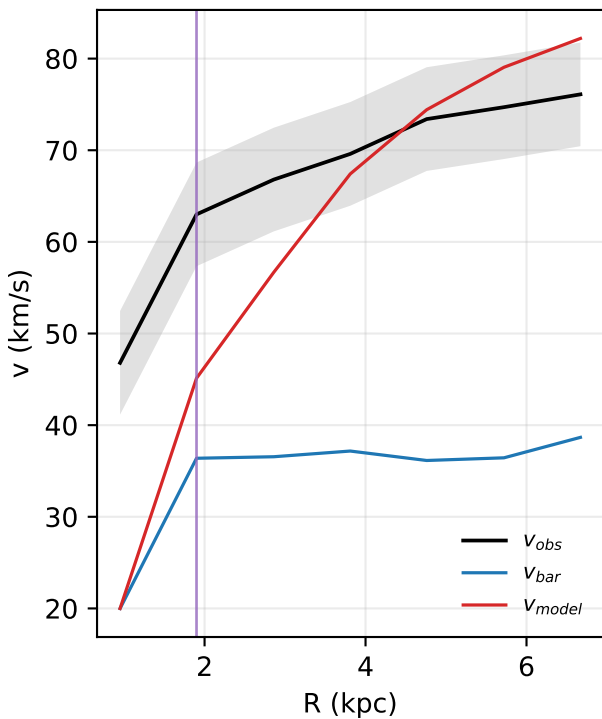
UGC07261: rotation curve
