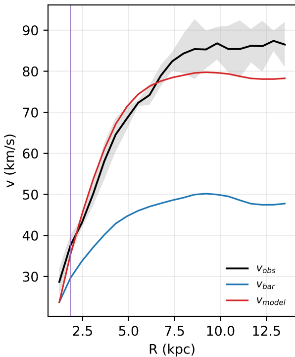
NGC0055: rotation curve
