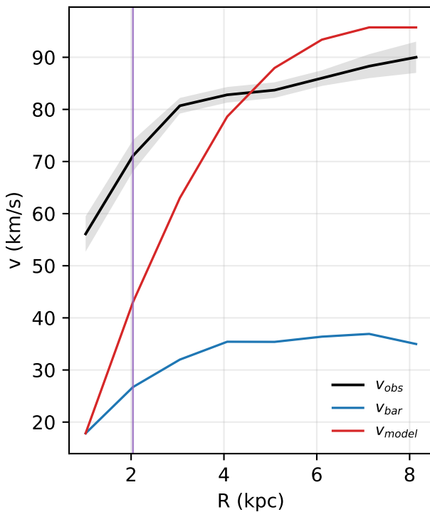
UGC02259: rotation curve
