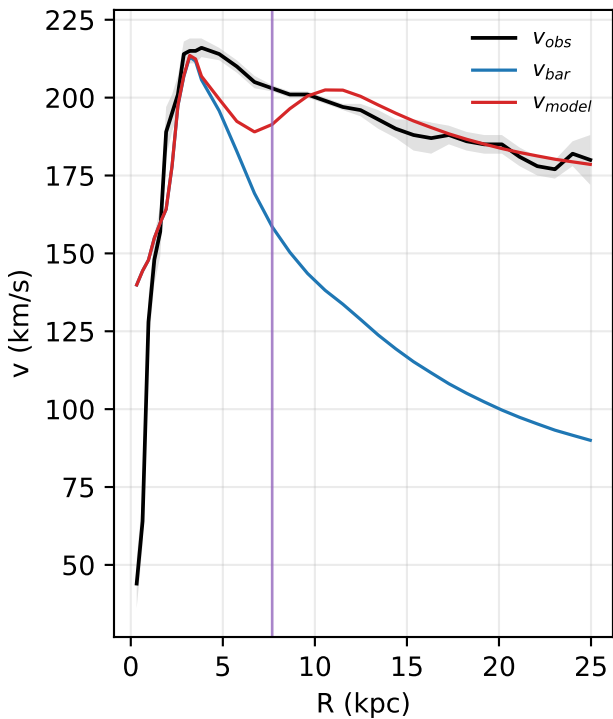
NGC2903: rotation curve
