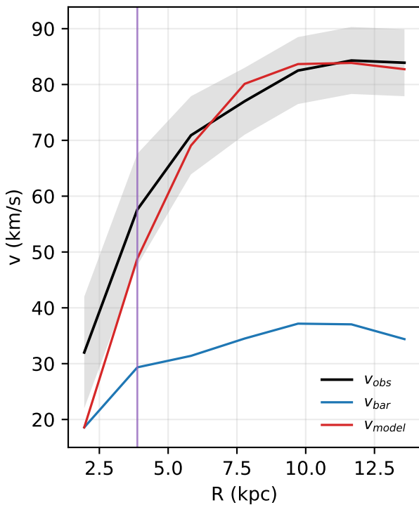
F571-V1: rotation curve
