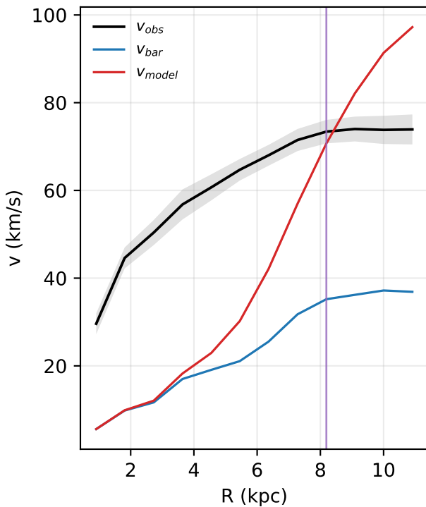
UGC00731: rotation curve
