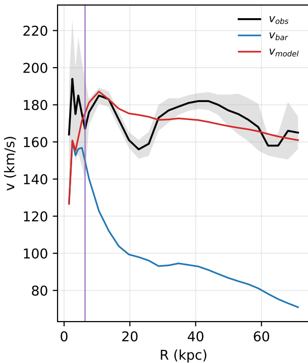
NGC0289: rotation curve
