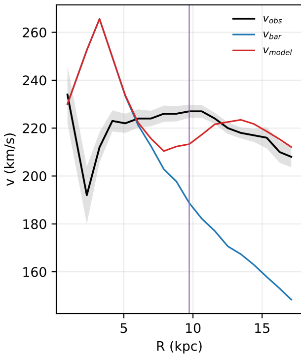
NGC0891: rotation curve
