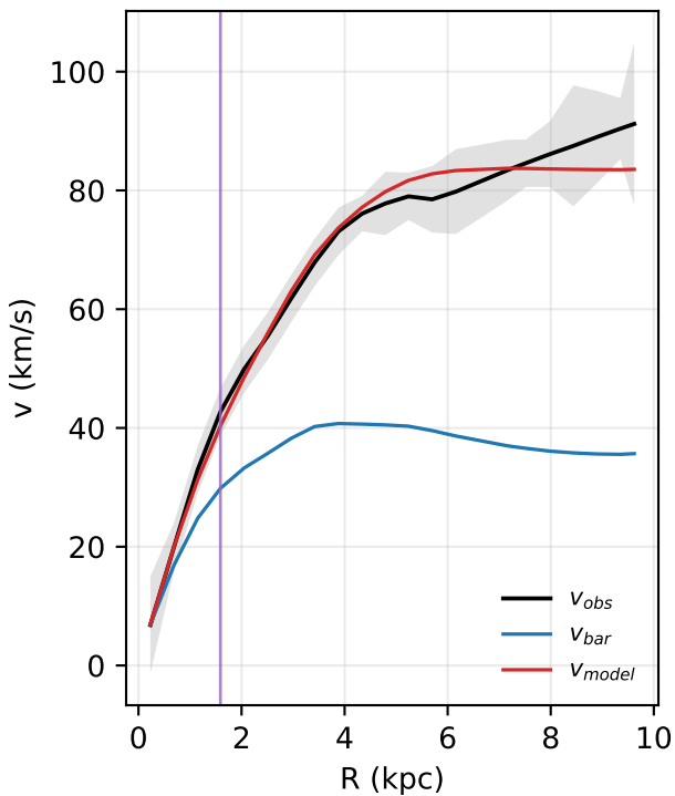
NGC0100: rotation curve
