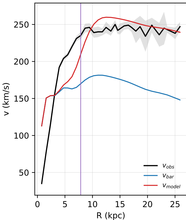
IC4202: rotation curve
