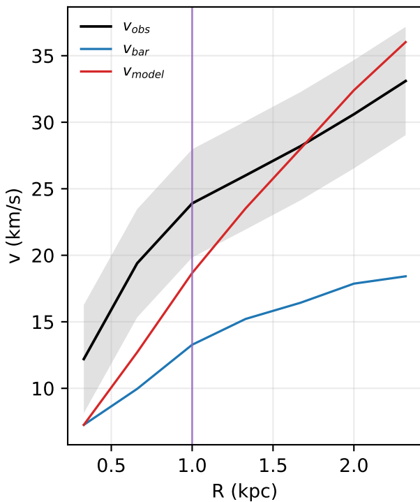
UGC07866: rotation curve
