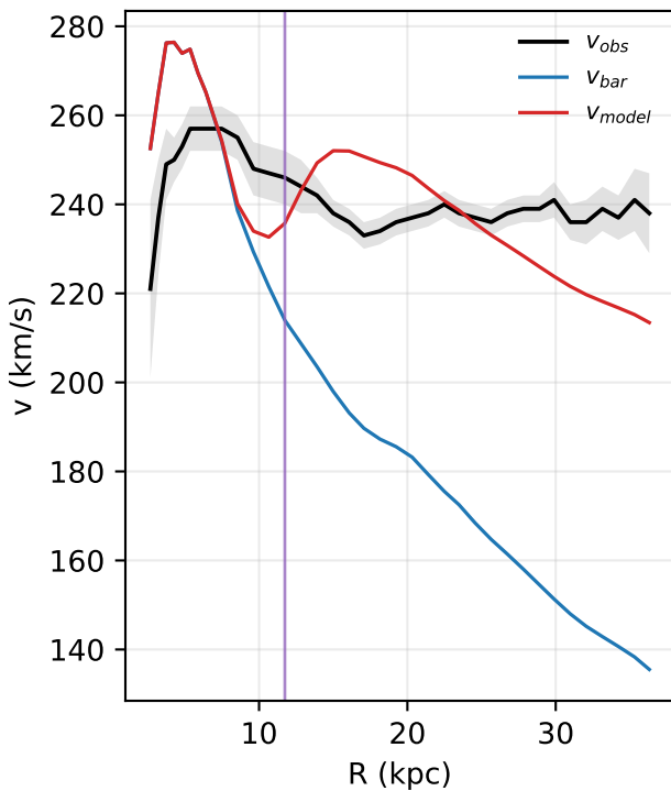
NGC7331: rotation curve
