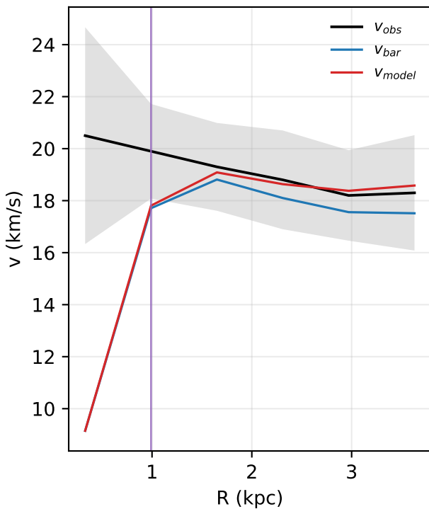
PGC51017: rotation curve
