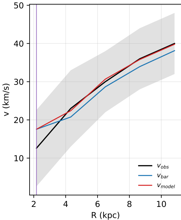
F574-2: rotation curve
