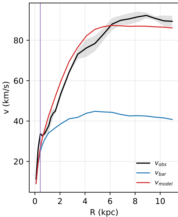
NGC5585: rotation curve
