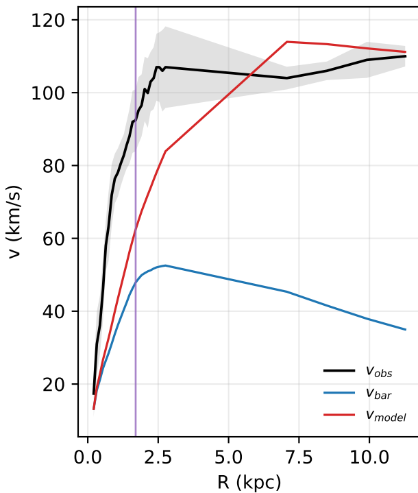
NGC0024: rotation curve
