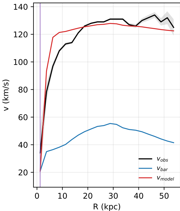
UGC00128: rotation curve
