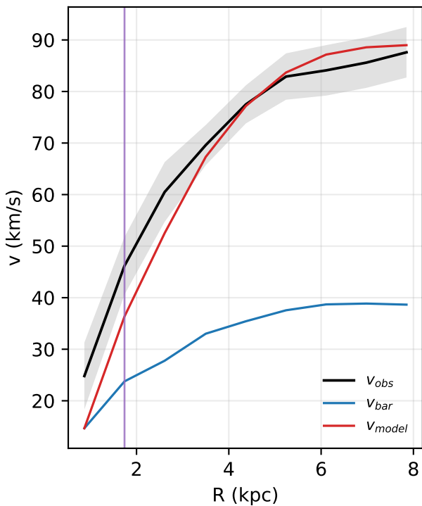
UGC06399: rotation curve
