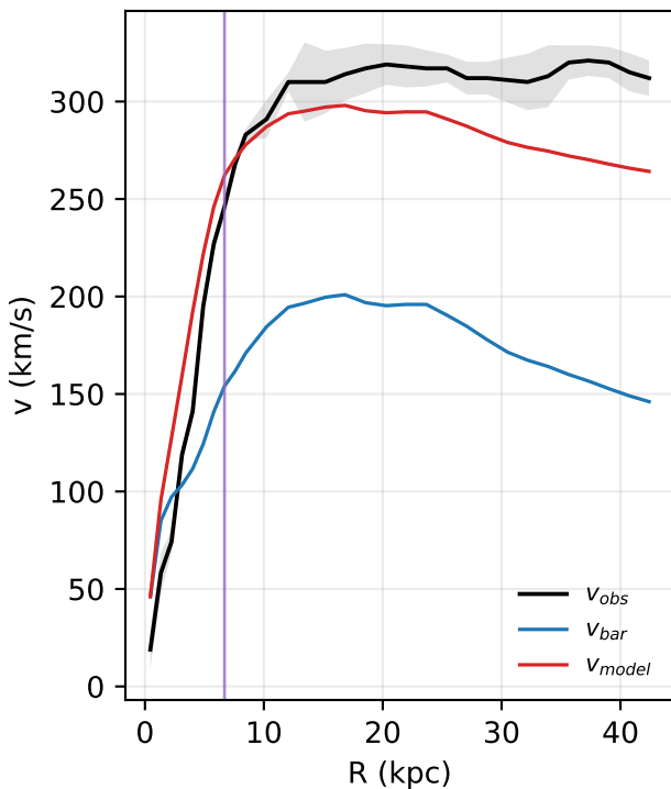
ESO563-G021: rotation curve
