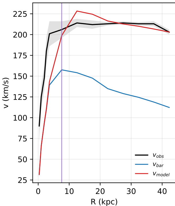
NGC2998: rotation curve
