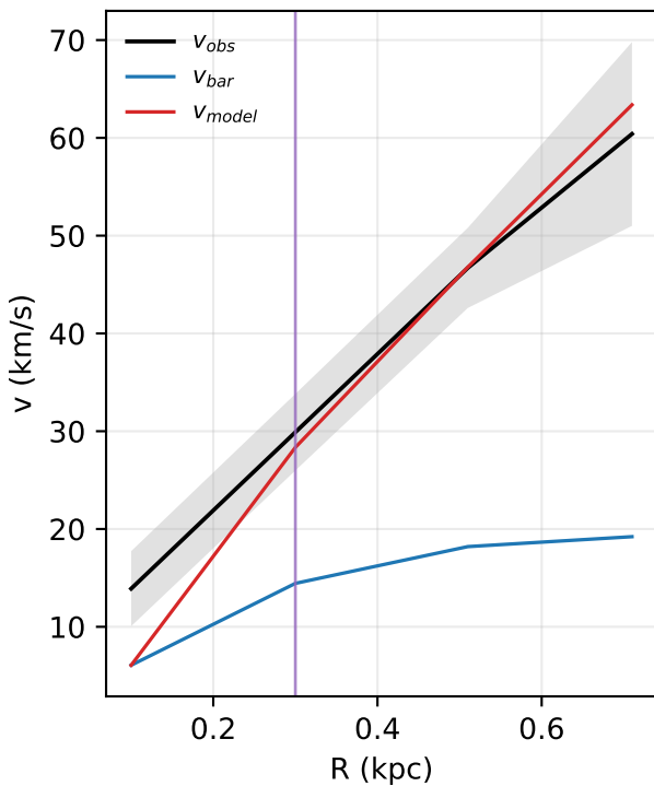
NGC6789: rotation curve
