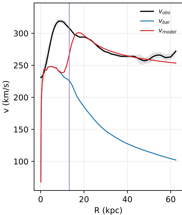
UGC02953: rotation curve
