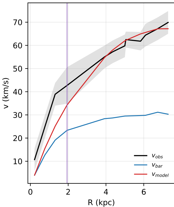
F583-4: rotation curve
