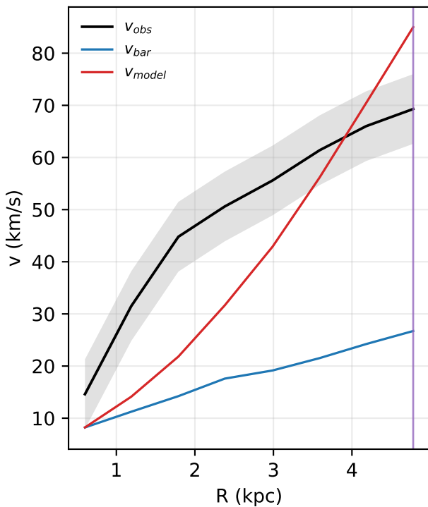
UGC07608: rotation curve
