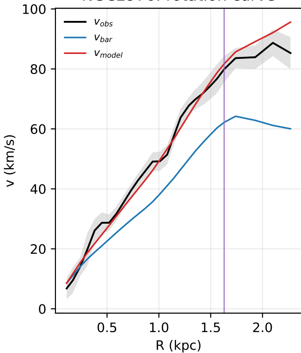
NGC2976: rotation curve
