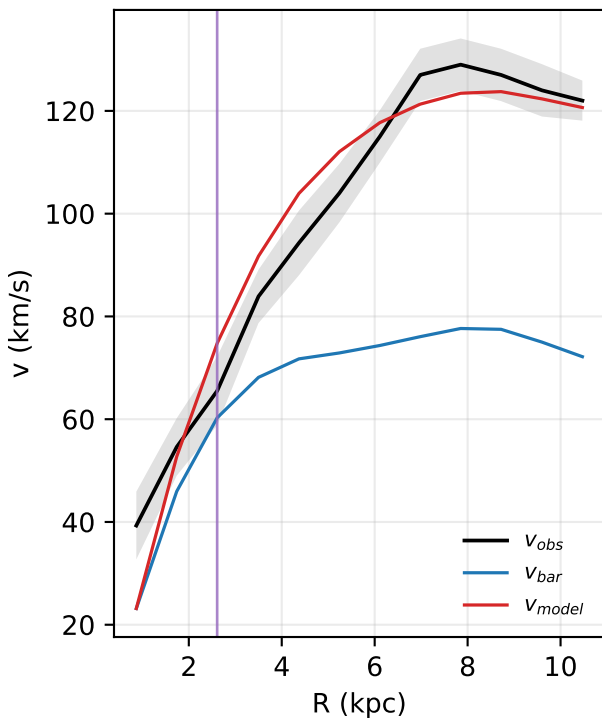
NGC4010: rotation curve
