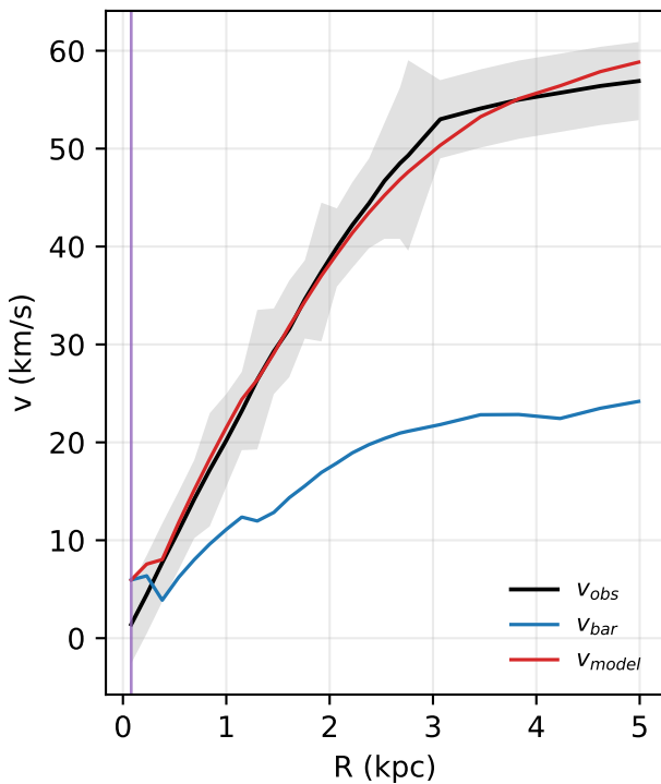
UGC01281: rotation curve
