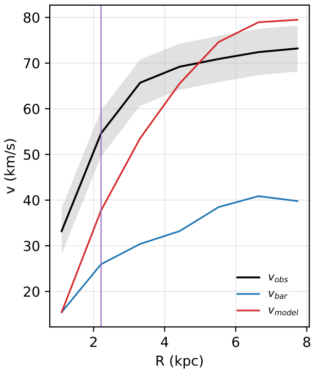
UGC10310: rotation curve
