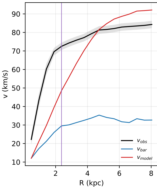
UGC08286: rotation curve
