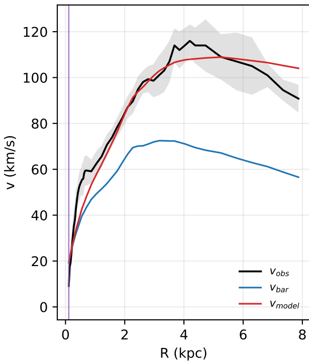
NGC7793: rotation curve
