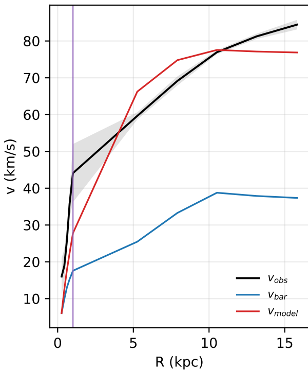
UGC11820: rotation curve
