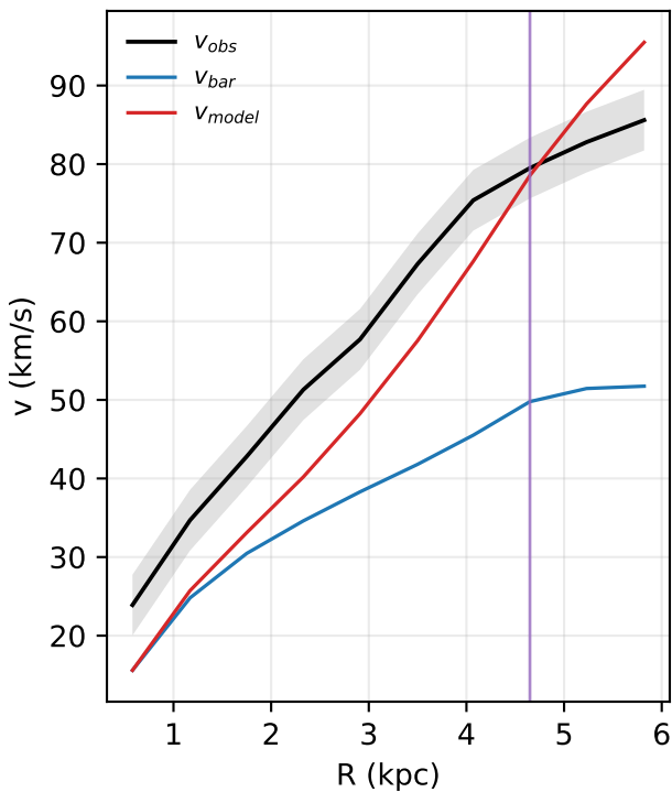
UGC07323: rotation curve
