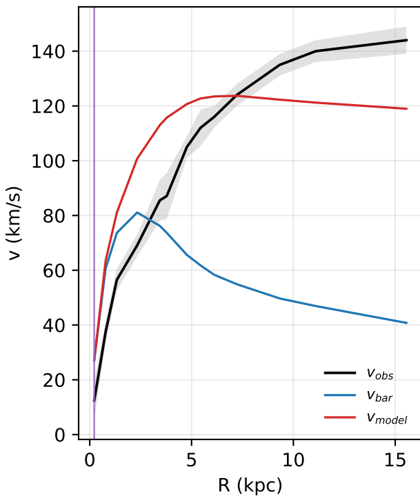
F571-8: rotation curve
