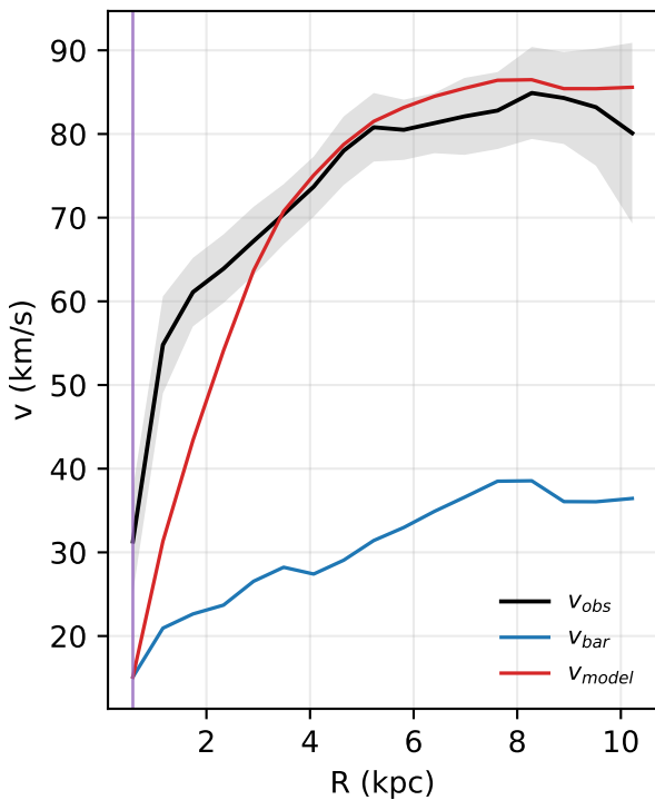
UGC06446: rotation curve
