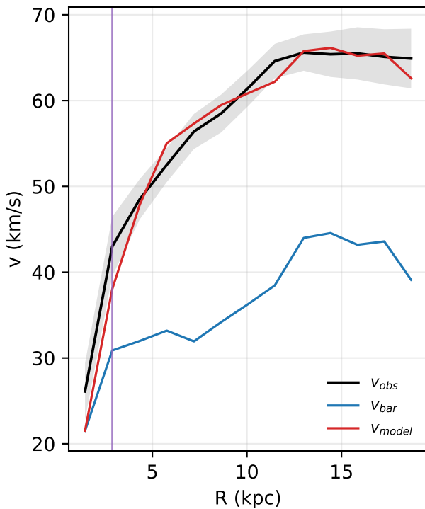
UGC07125: rotation curve
