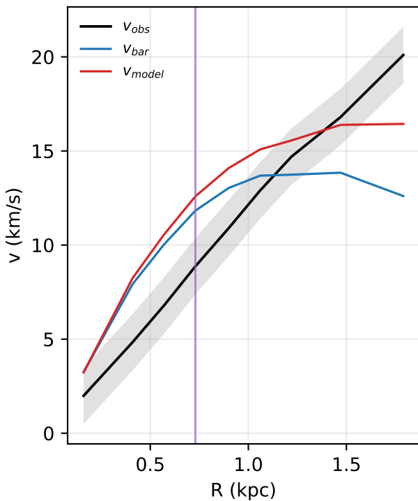
CamB: rotation curve
