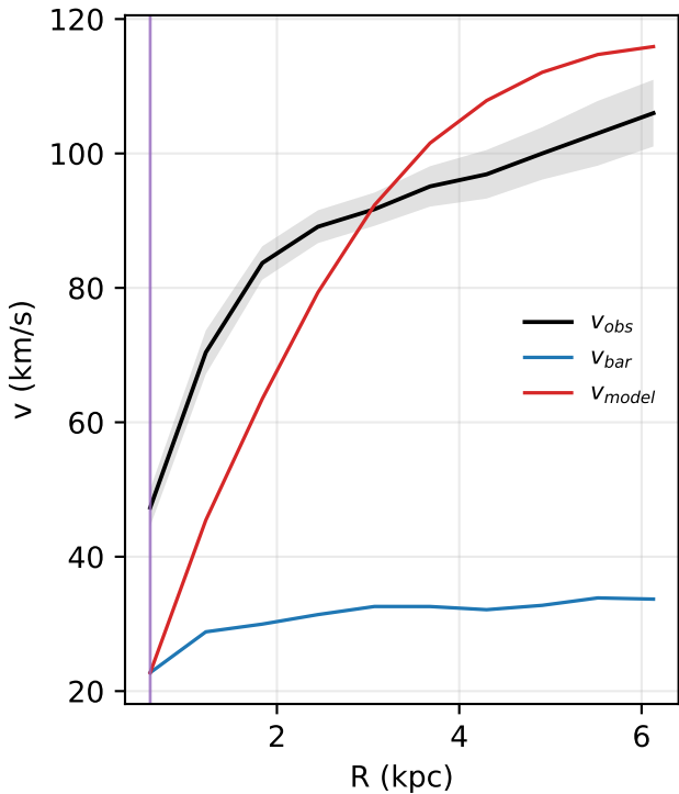
UGC07399: rotation curve
