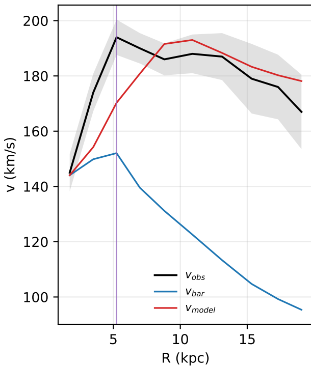
NGC3893: rotation curve
