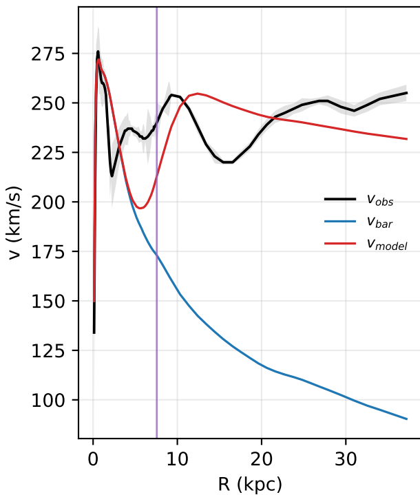
UGC06787: rotation curve
