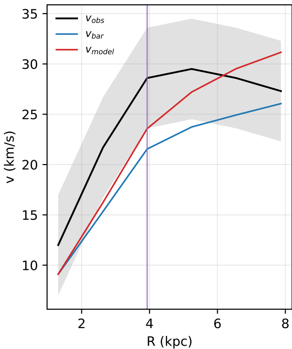
F563-V1: rotation curve
