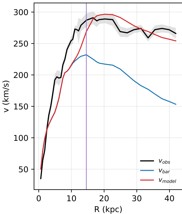
UGC11455: rotation curve
