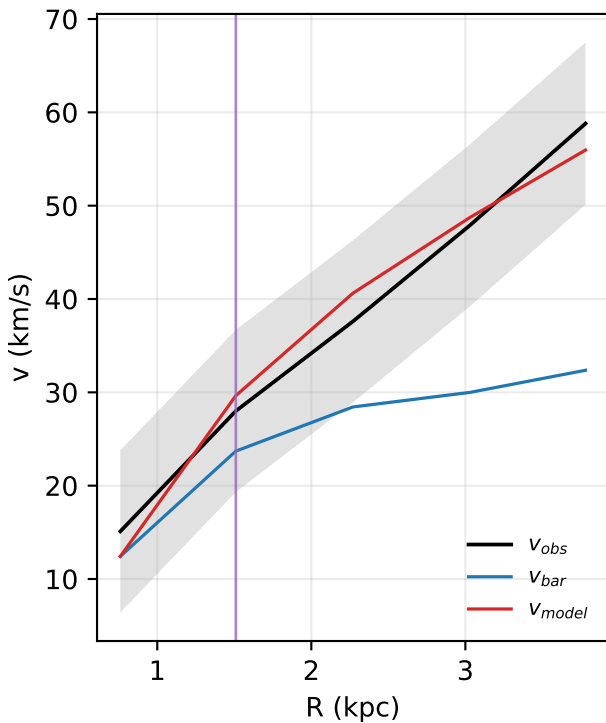
UGC02023: rotation curve
