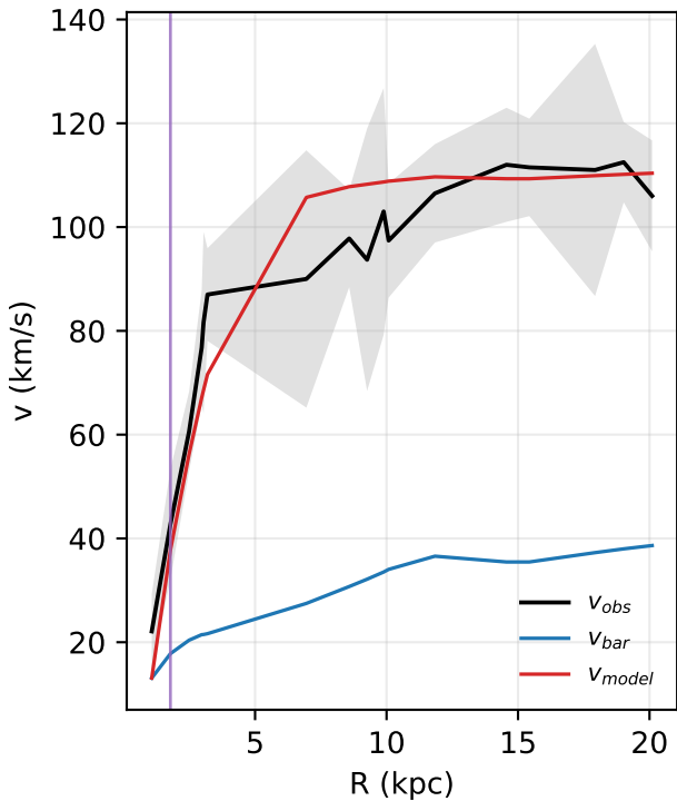
F563-1: rotation curve
