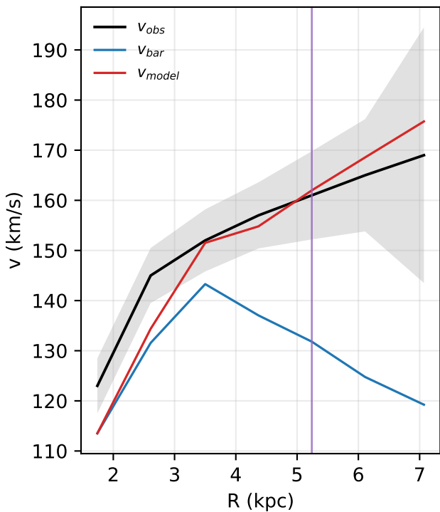
NGC3949: rotation curve
