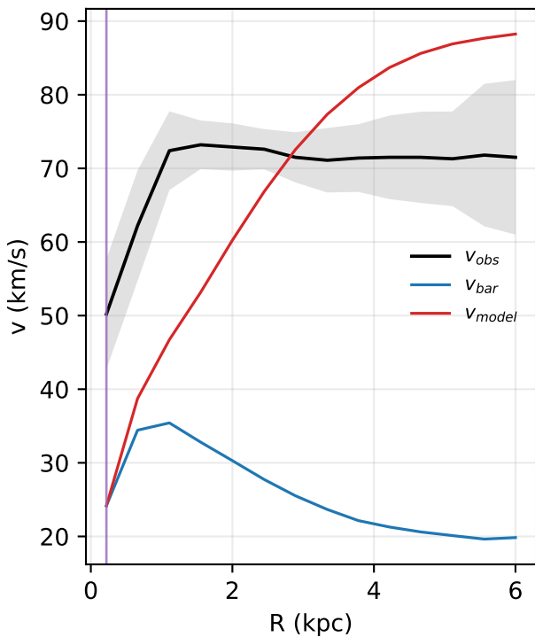
NGC1705: rotation curve
