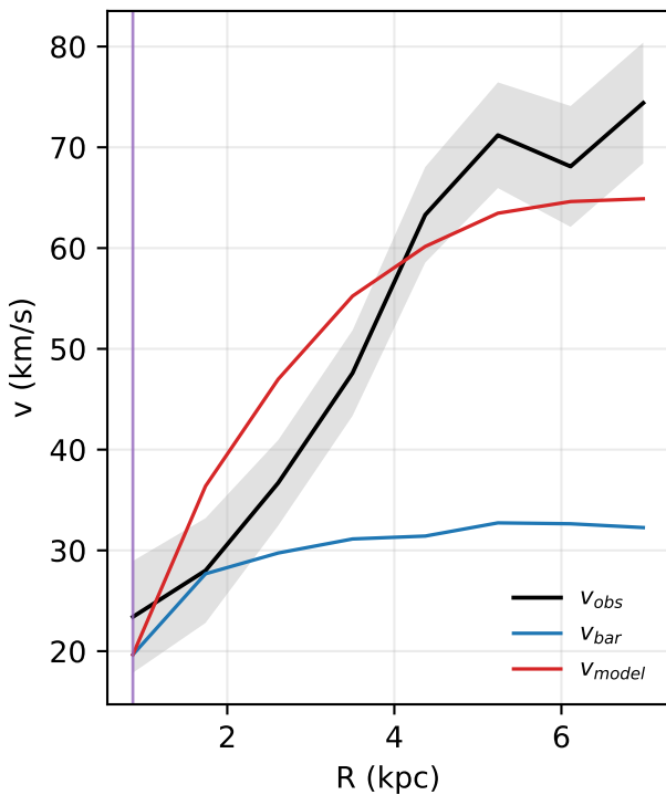
UGC06818: rotation curve
