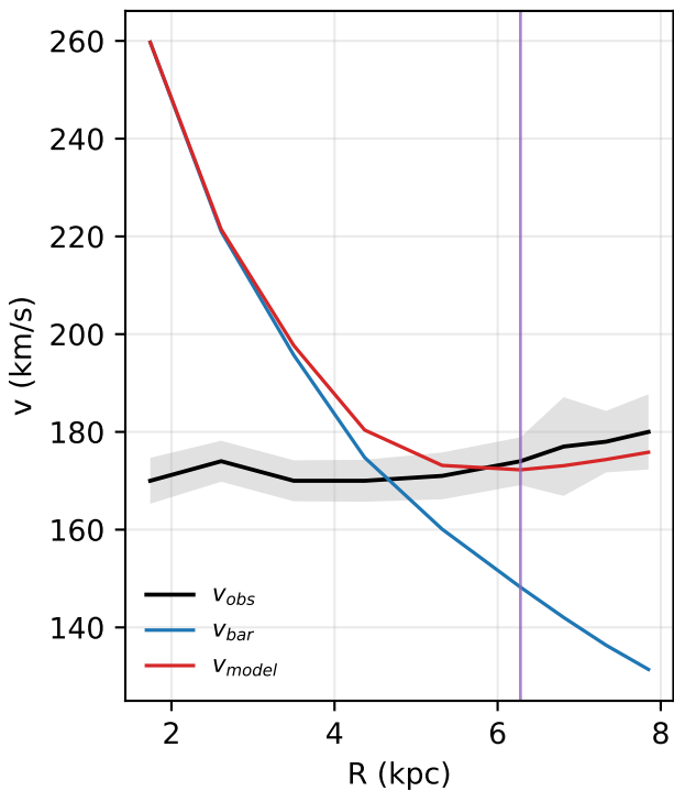
UGC06973: rotation curve
