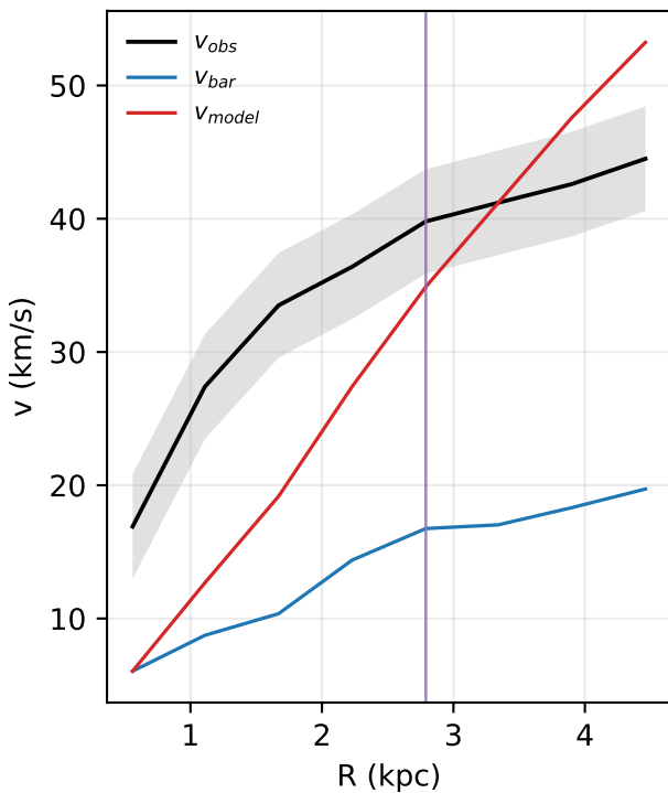
UGC05918: rotation curve
