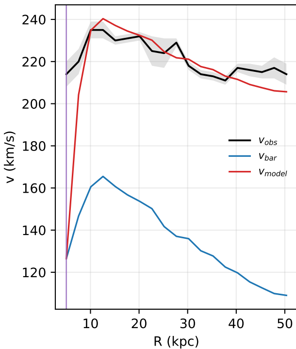
NGC5907: rotation curve
