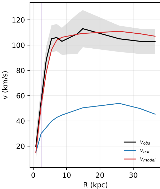
UGC01230: rotation curve
