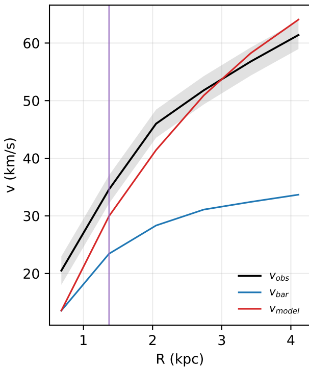
UGC05414: rotation curve
