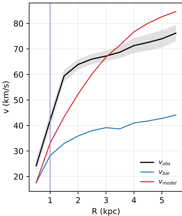
UGC07151: rotation curve
