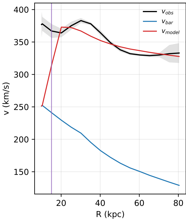
UGC02487: rotation curve
