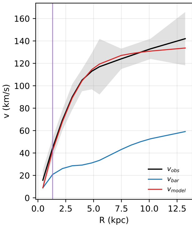
F568-1: rotation curve
