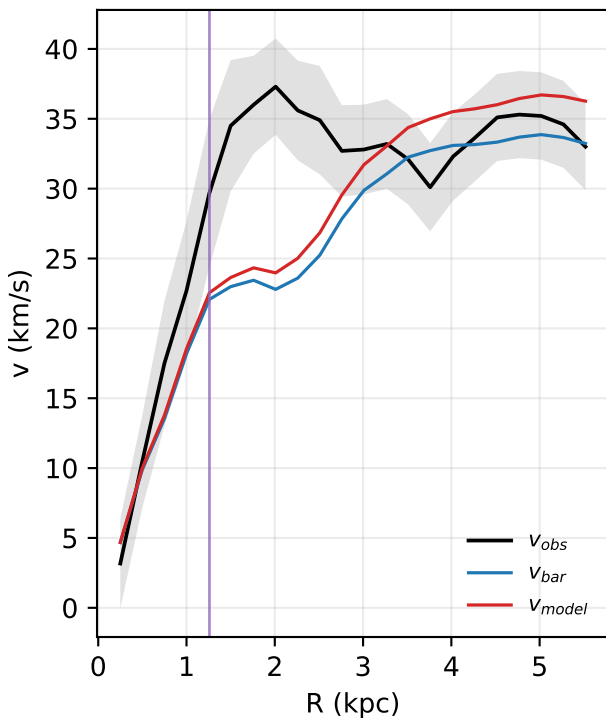
UGC04305: rotation curve
