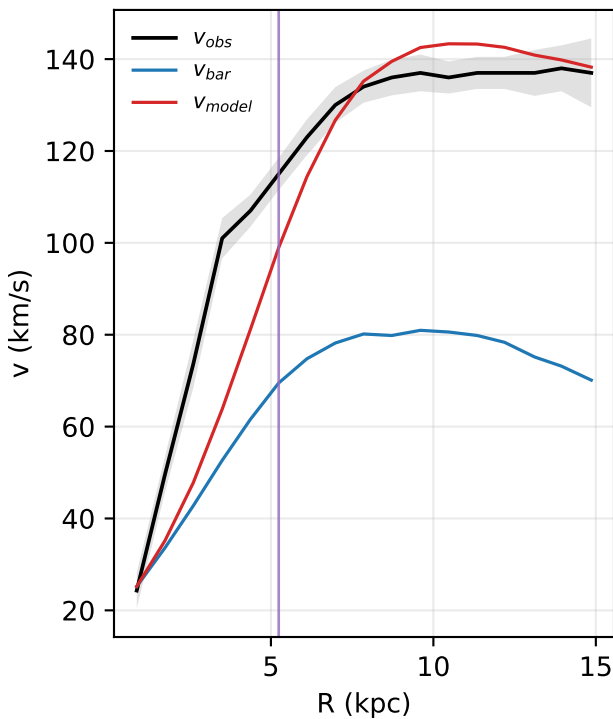
NGC3917: rotation curve
