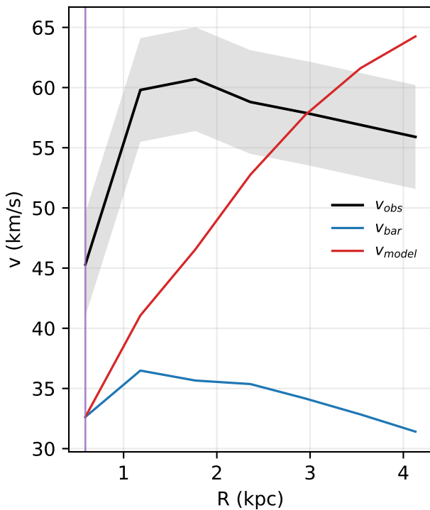
UGC07690: rotation curve
