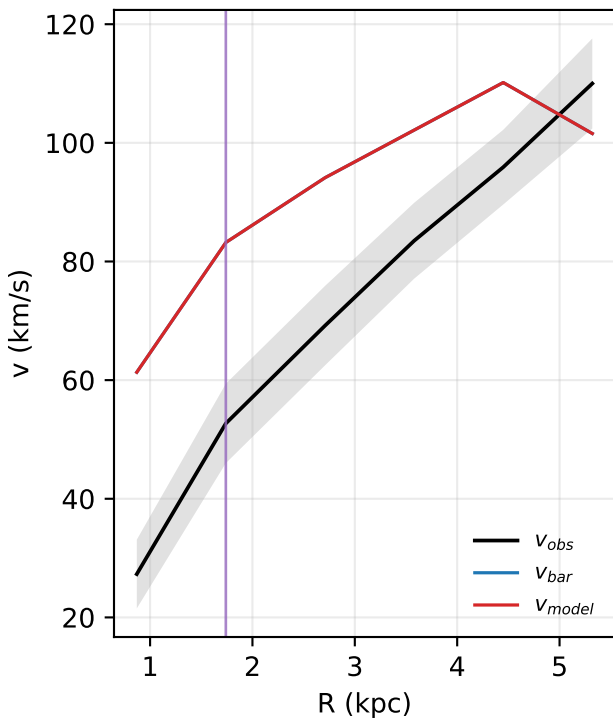
NGC4389: rotation curve
