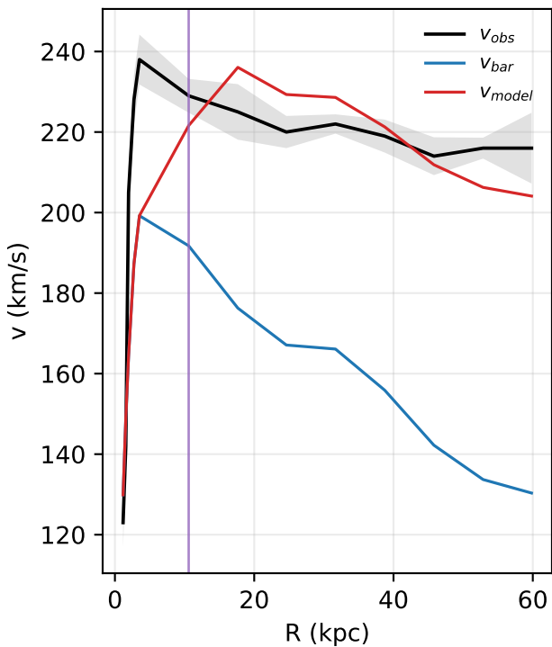
NGC0801: rotation curve
