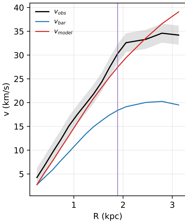
KK98-251: rotation curve
