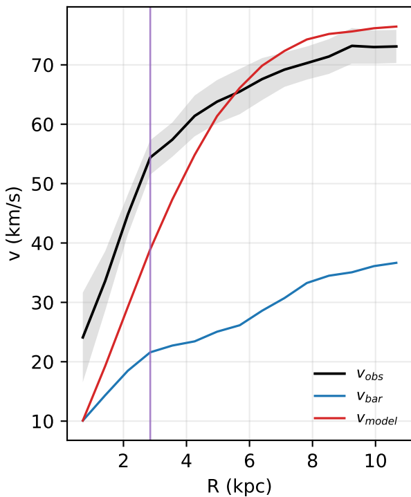
UGC12632: rotation curve
