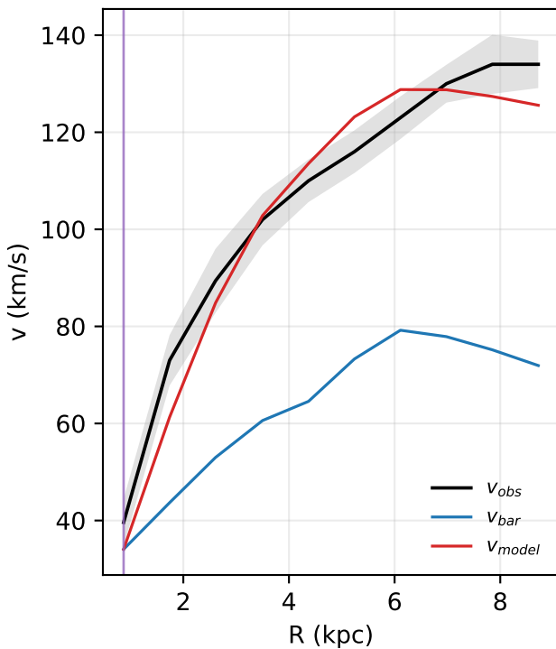
NGC3972: rotation curve
