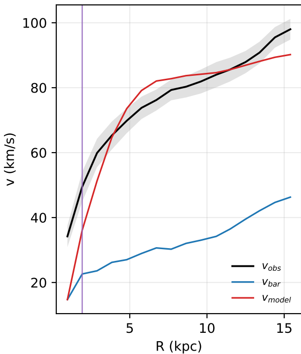
UGC12732: rotation curve
