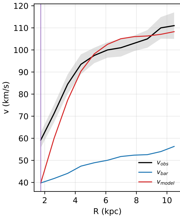
UGC06917: rotation curve
