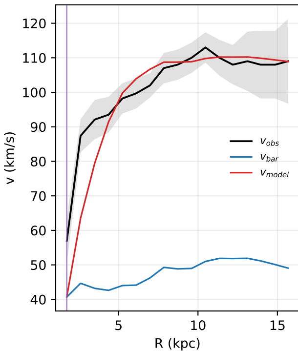
UGC06983: rotation curve
