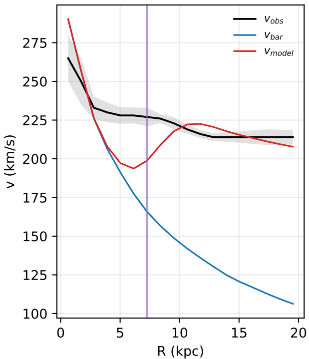
NGC7814: rotation curve
