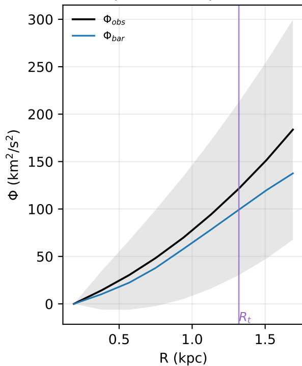
Inferred potential (up to constant)
