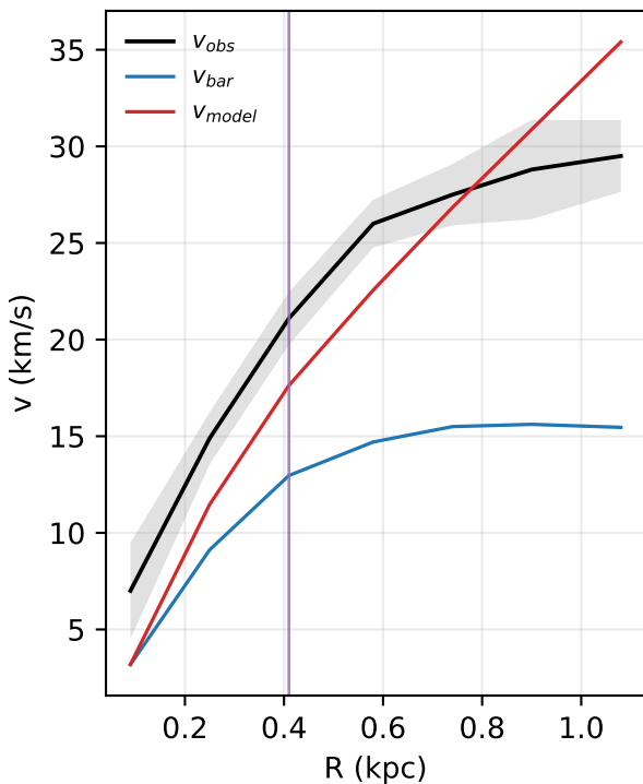
UGCA281: rotation curve
