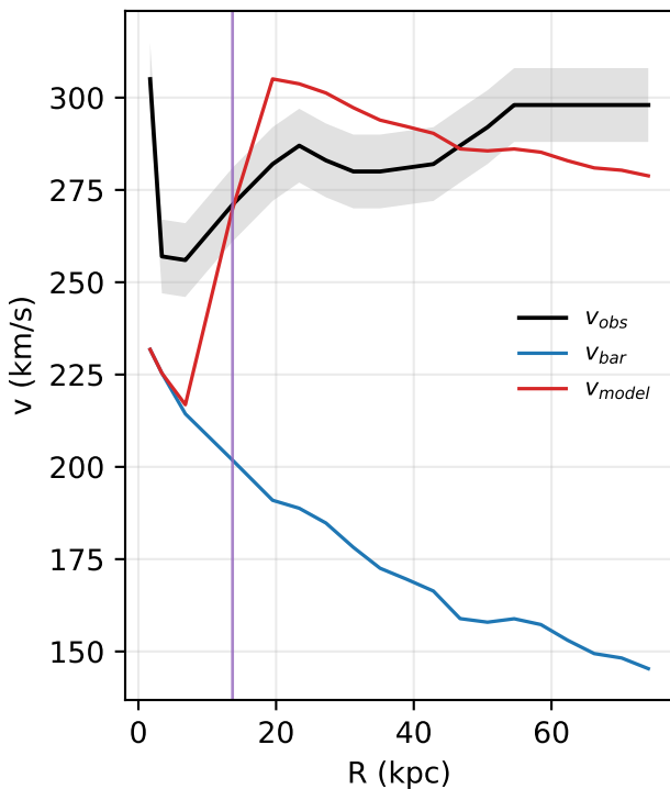
UGC02885: rotation curve
