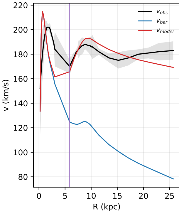
UGC08699: rotation curve
