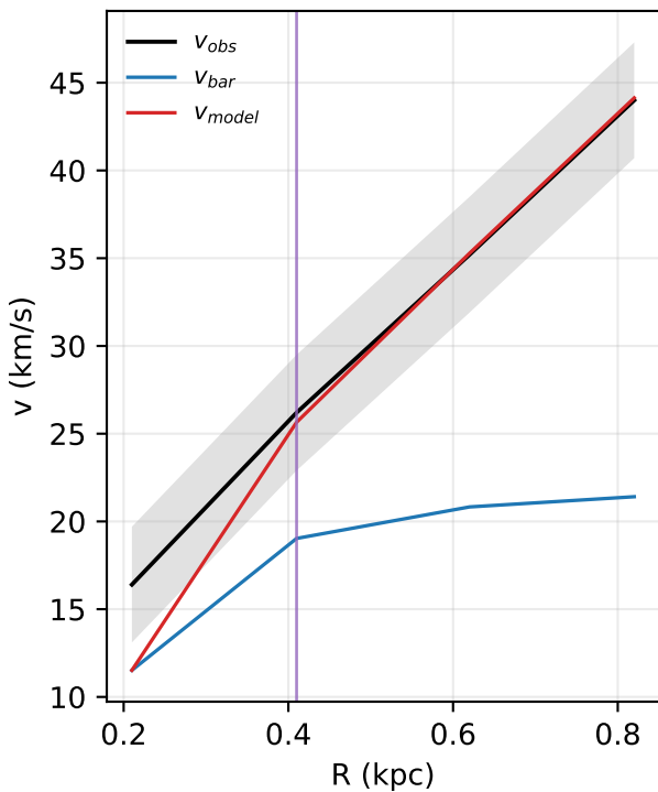
UGC07232: rotation curve
