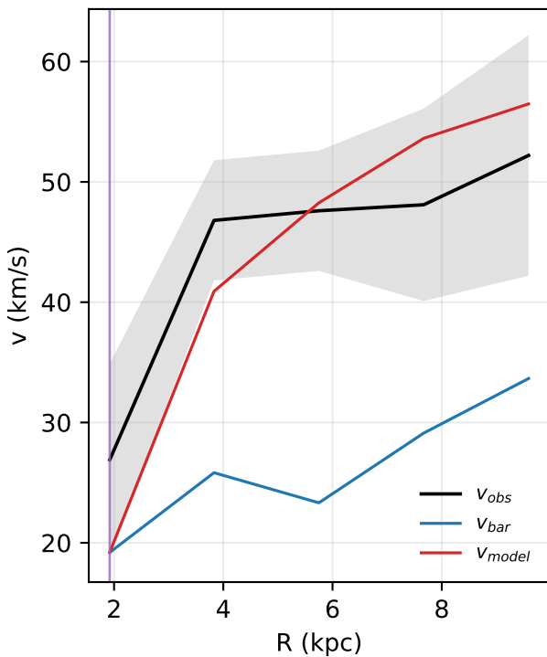
F567-2: rotation curve
