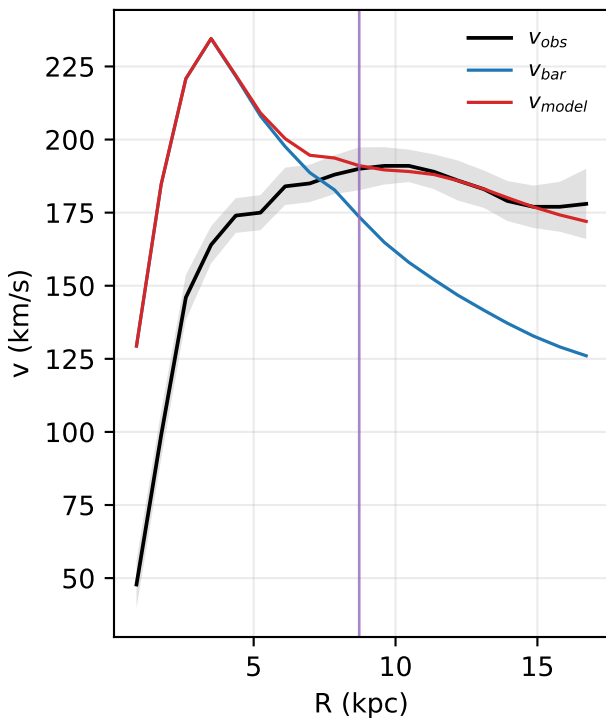
NGC4217: rotation curve
