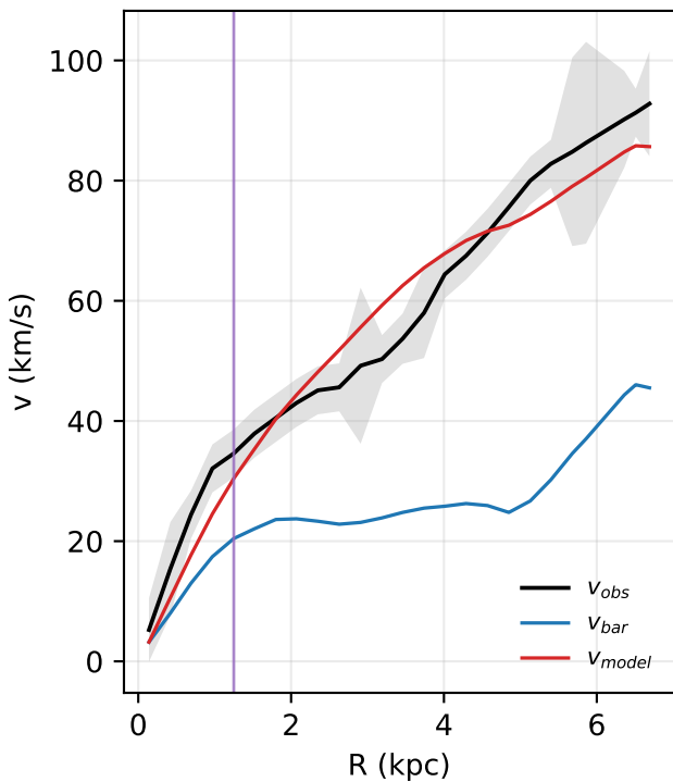
UGC04278: rotation curve
