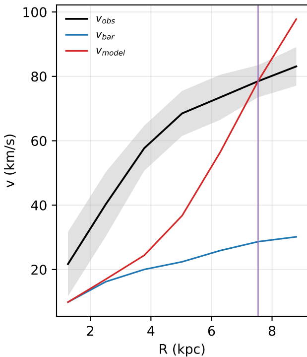
F565-V2: rotation curve
