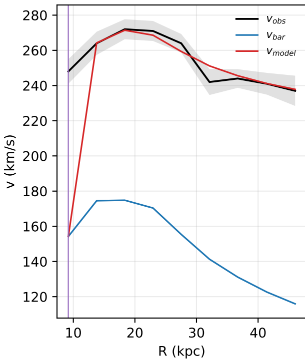
NGC3992: rotation curve
