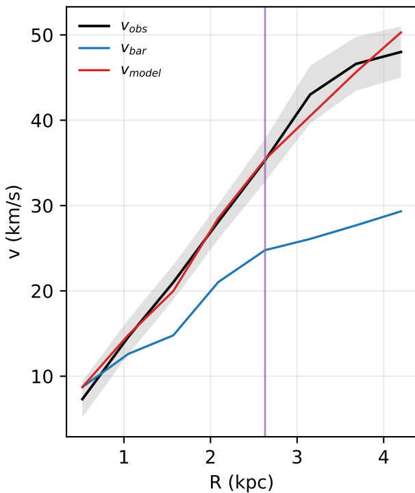
UGC08837: rotation curve
