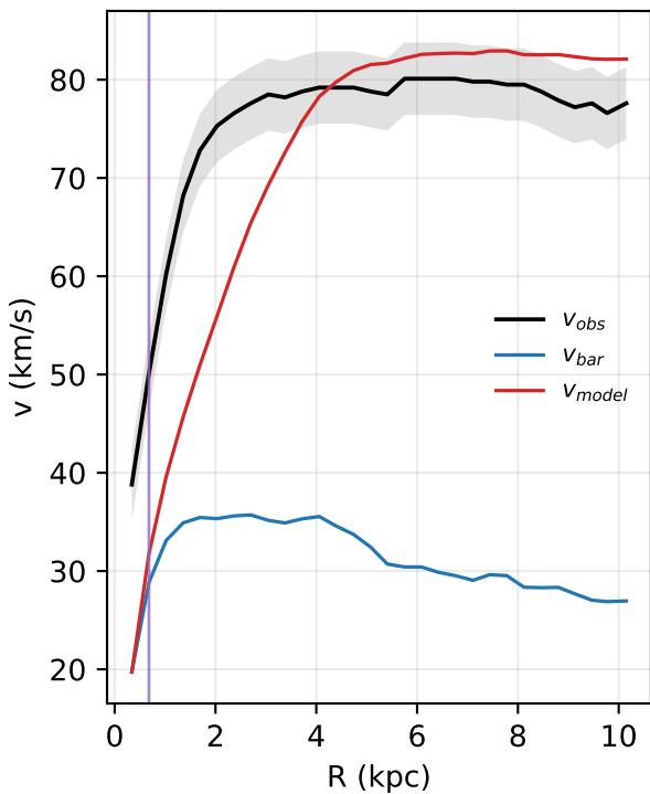
UGC08490: rotation curve
