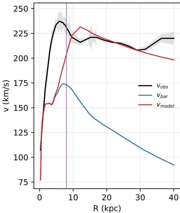
UGC03205: rotation curve
