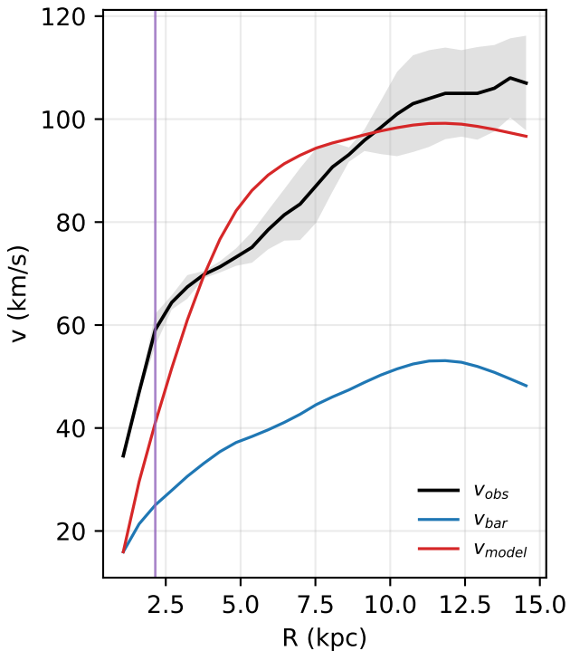
NGC0247: rotation curve
