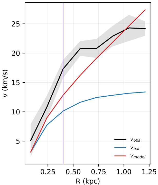
UGC04483: rotation curve
