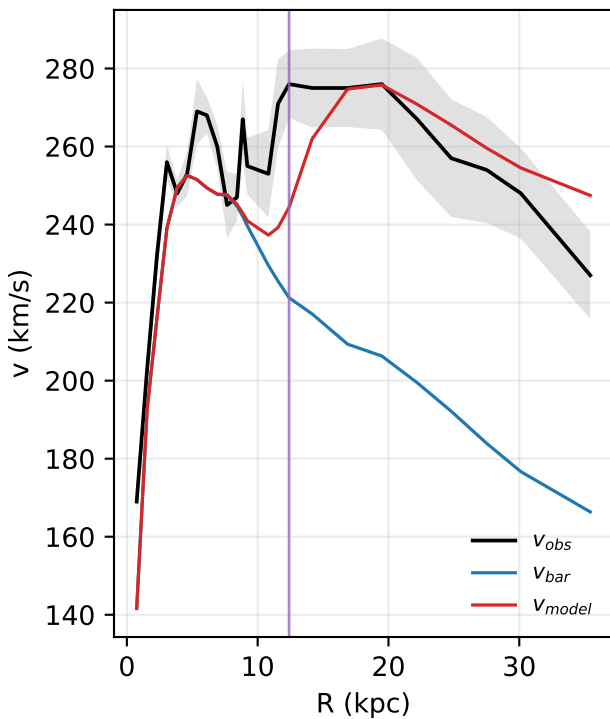
NGC2955: rotation curve
