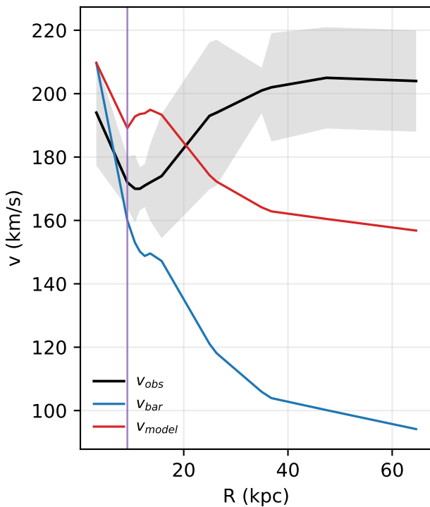
UGC06614: rotation curve
