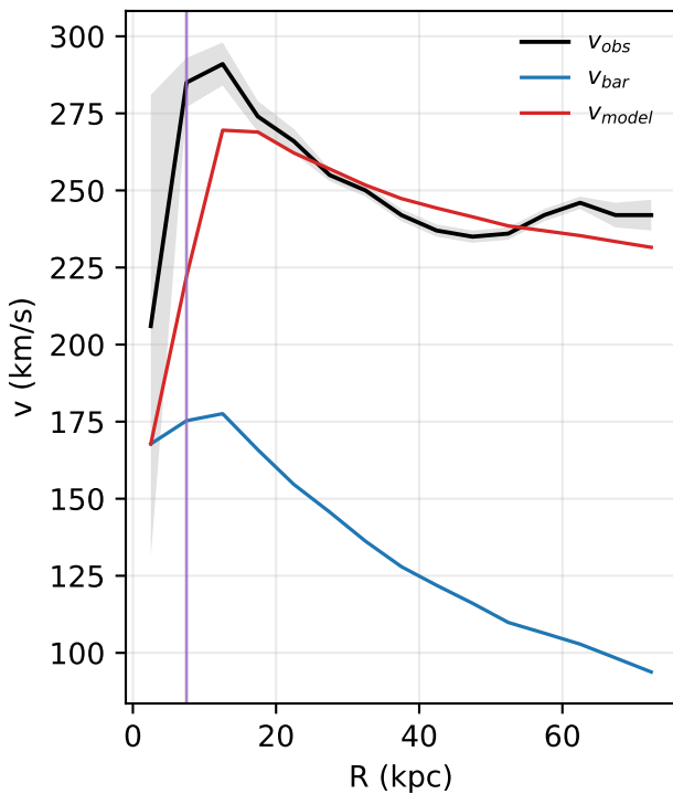
NGC6674: rotation curve
