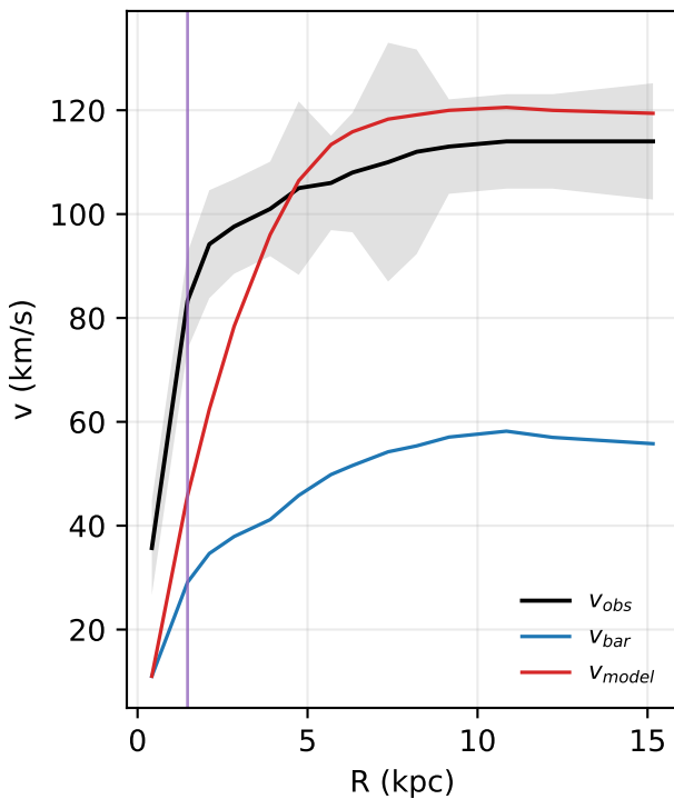
F579-V1: rotation curve
