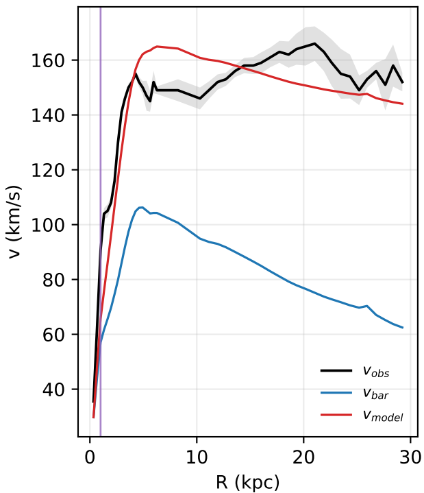
NGC6015: rotation curve
