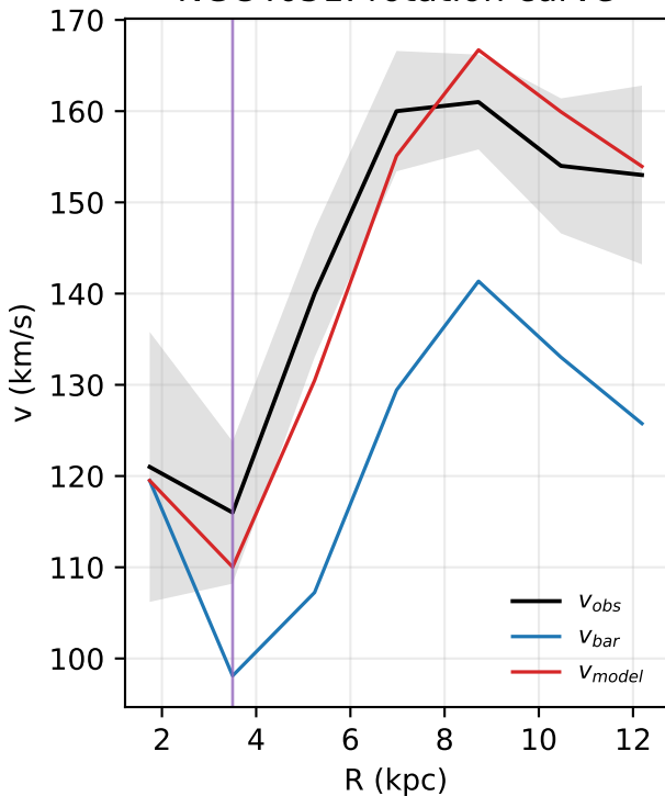
NGC4051: rotation curve
