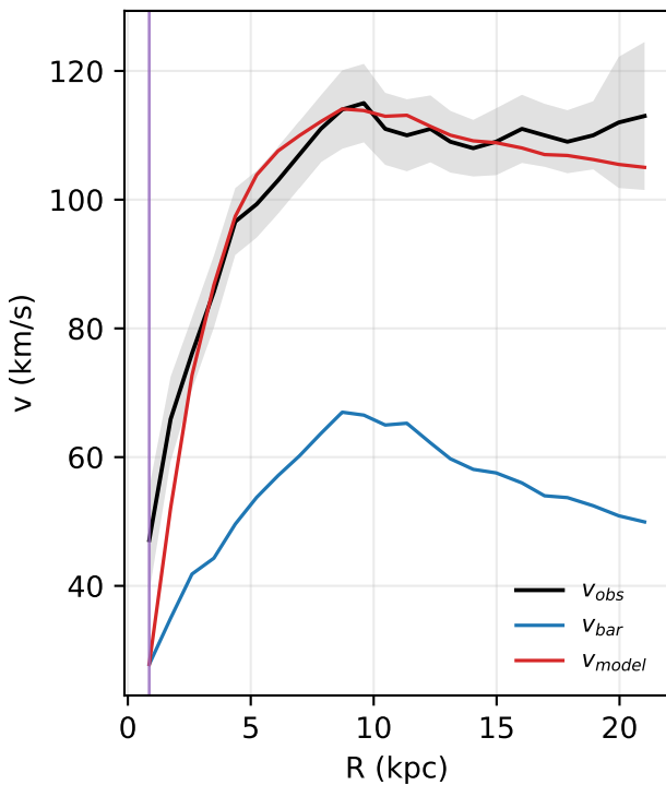
NGC4183: rotation curve
