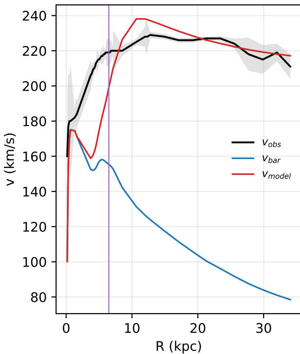
UGC06786: rotation curve
