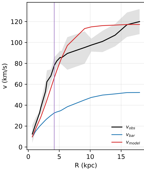
F568-3: rotation curve
