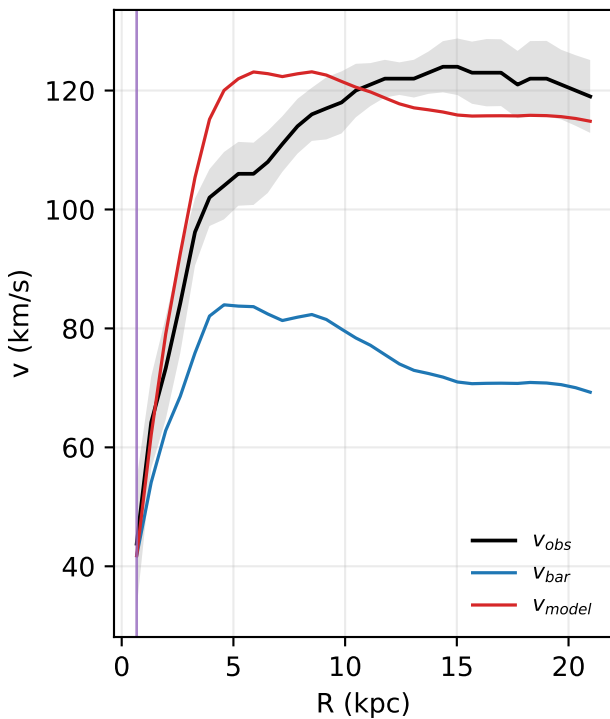
NGC4559: rotation curve
