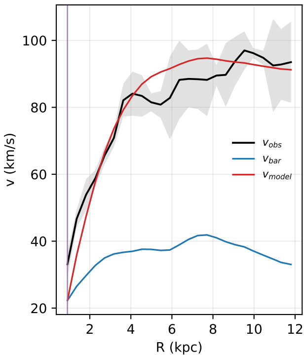
NGC0300: rotation curve
