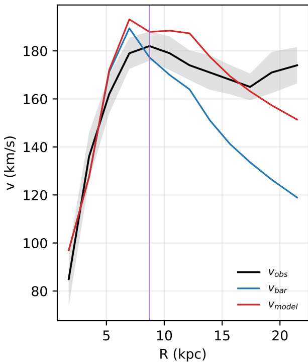
NGC4088: rotation curve
