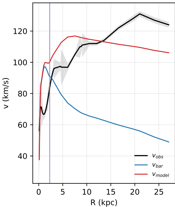
UGC03580: rotation curve
