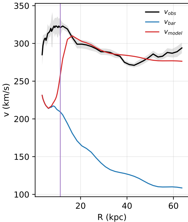
NGC2841: rotation curve
