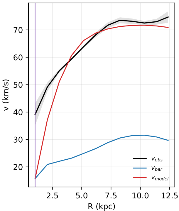
UGC05716: rotation curve
