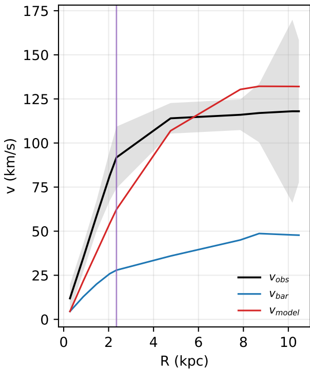
F563-V2: rotation curve
