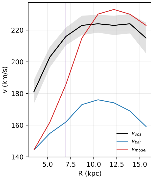
NGC3953: rotation curve
