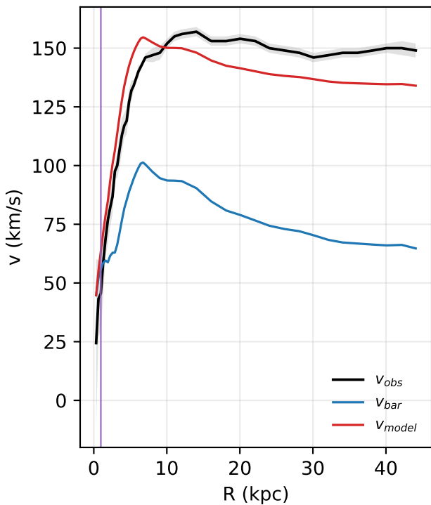
NGC3198: rotation curve
