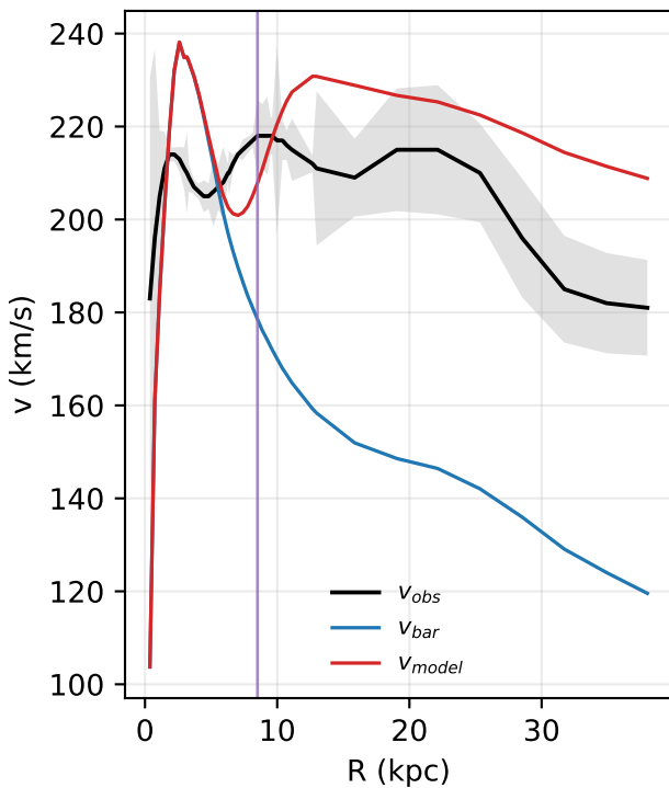
UGC02916: rotation curve
