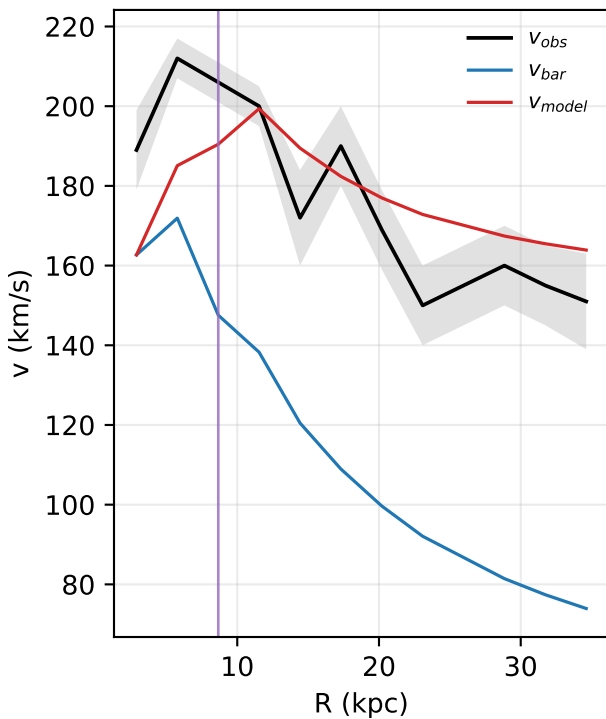
NGC2683: rotation curve
