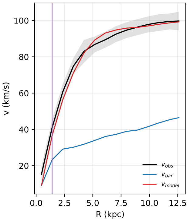
F574-1: rotation curve
