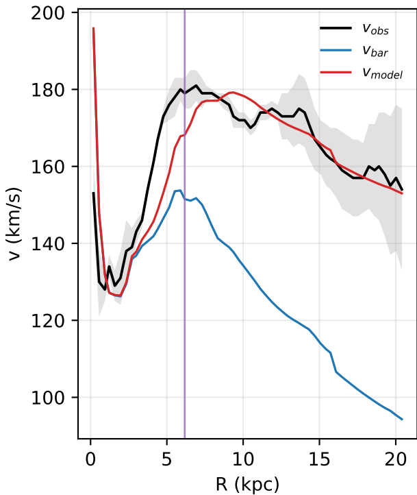
NGC6946: rotation curve
