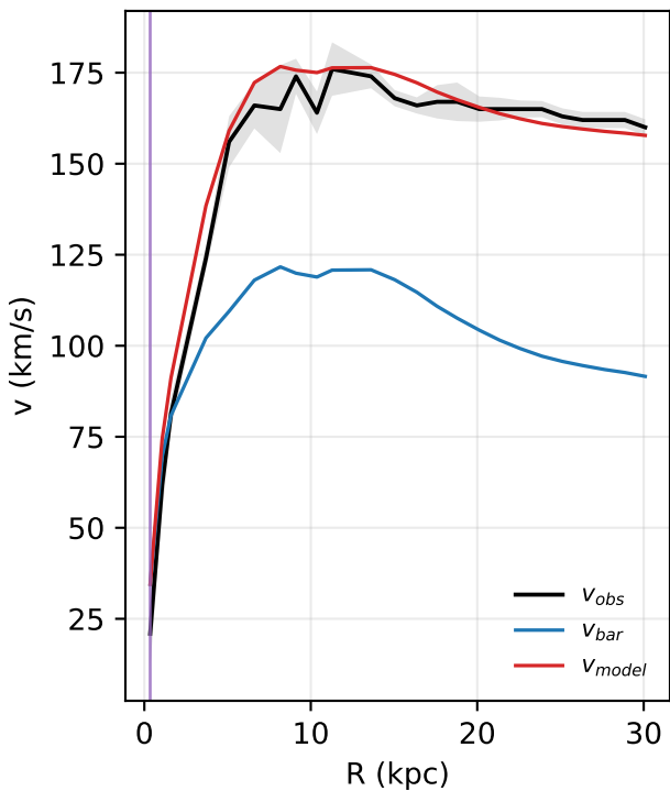
NGC1090: rotation curve
