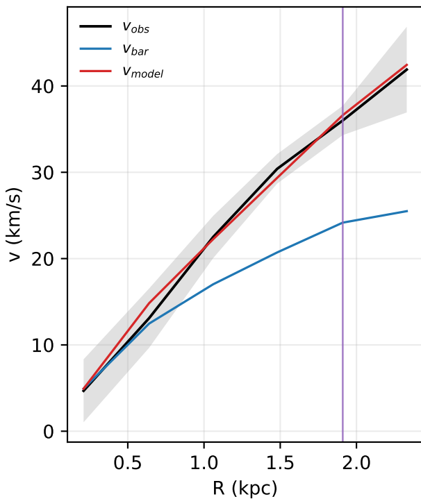
NGC4068: rotation curve
