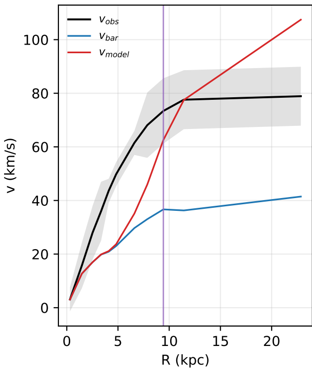
UGC05750: rotation curve
