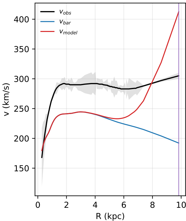
UGC11914: rotation curve
