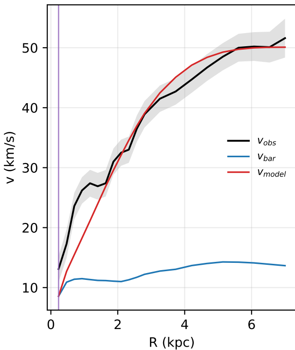
NGC3741: rotation curve
