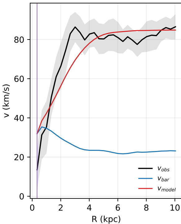
NGC2915: rotation curve
