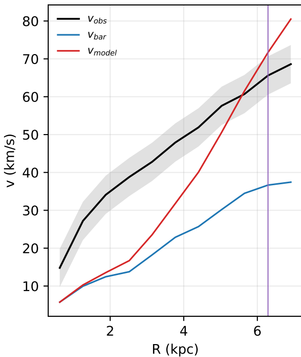
UGC05829: rotation curve
