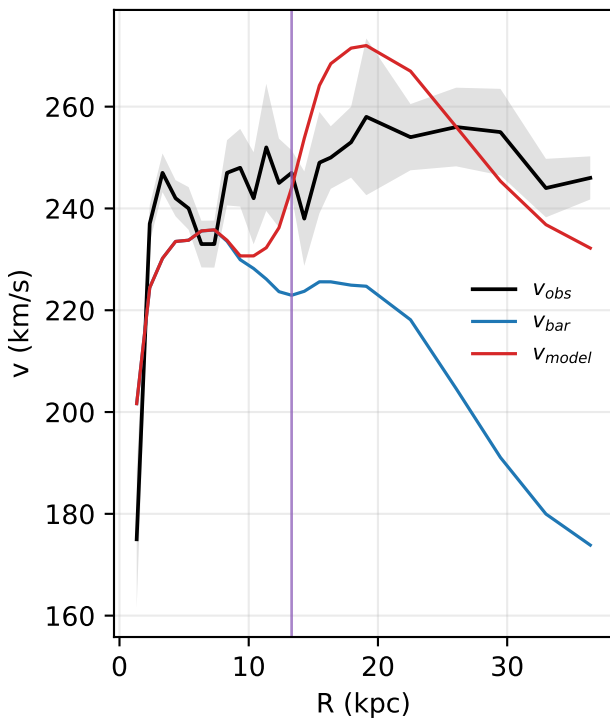
NGC6195: rotation curve
