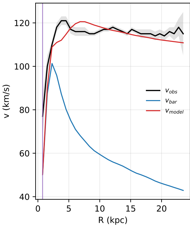
NGC6503: rotation curve
