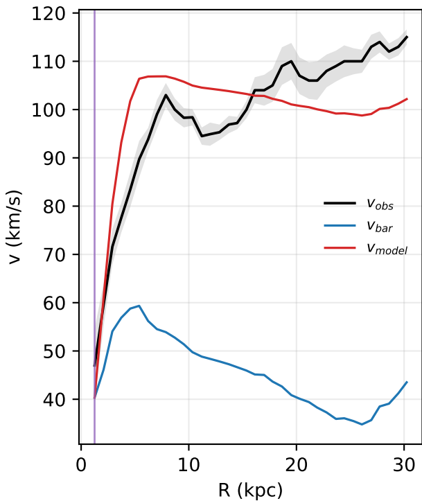
NGC1003: rotation curve
