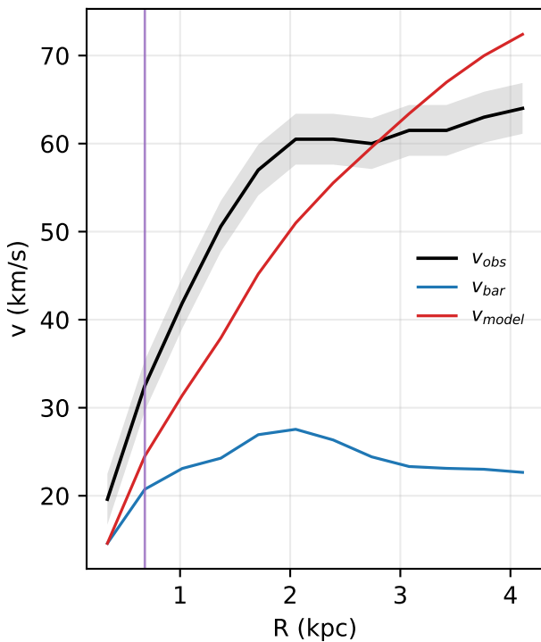
UGC07603: rotation curve
