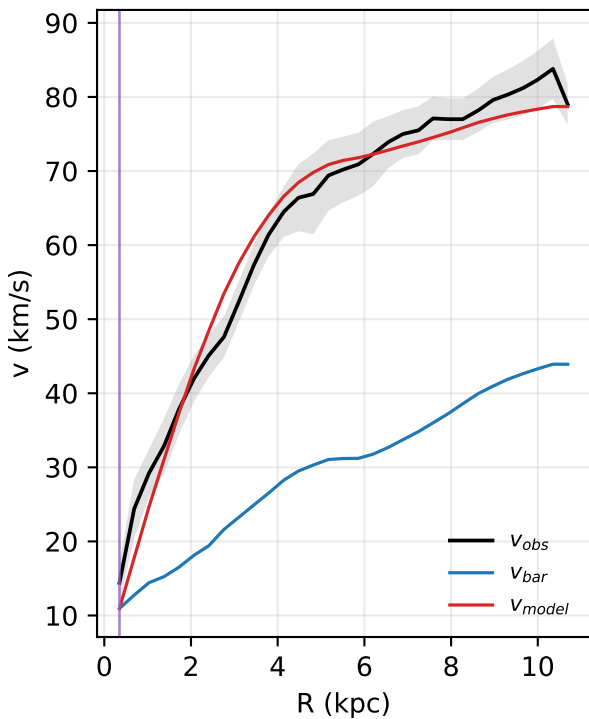
UGC07524: rotation curve
