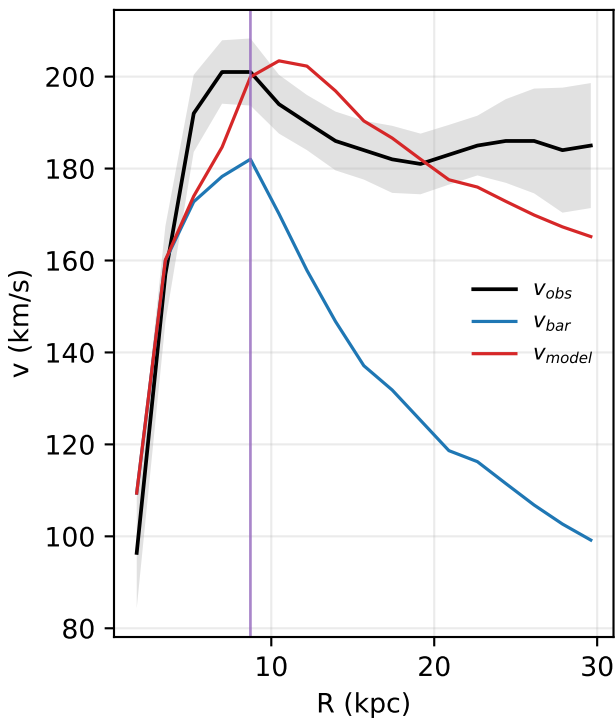
NGC4157: rotation curve
