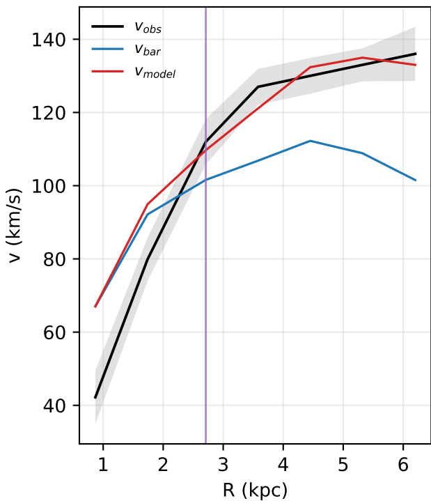
NGC4085: rotation curve
