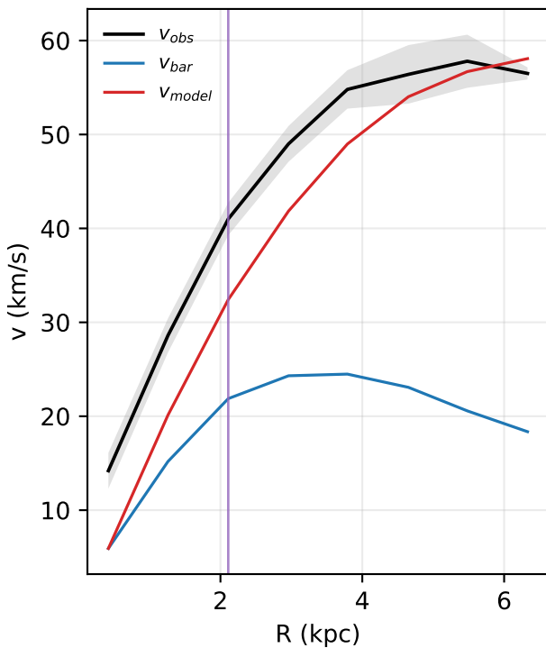
UGCA442: rotation curve
