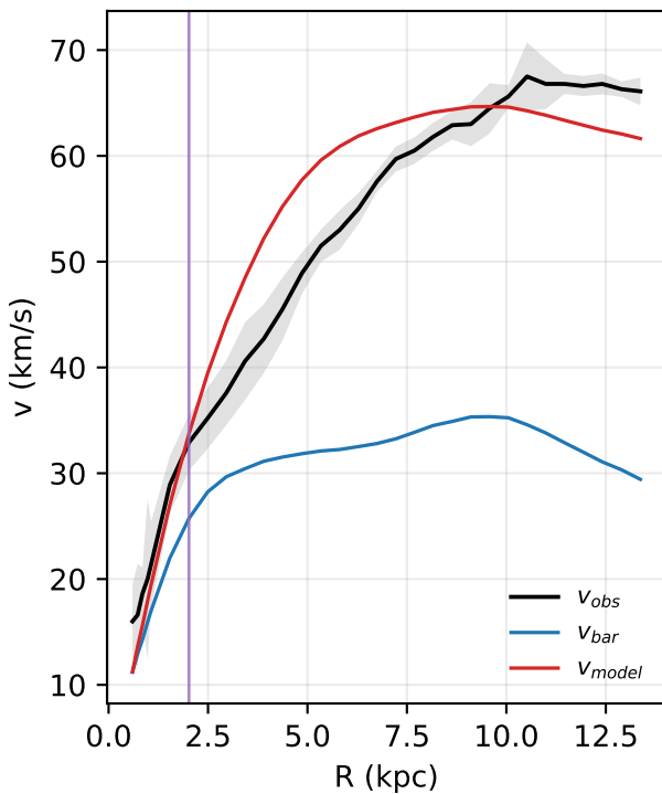
DDO161: rotation curve
