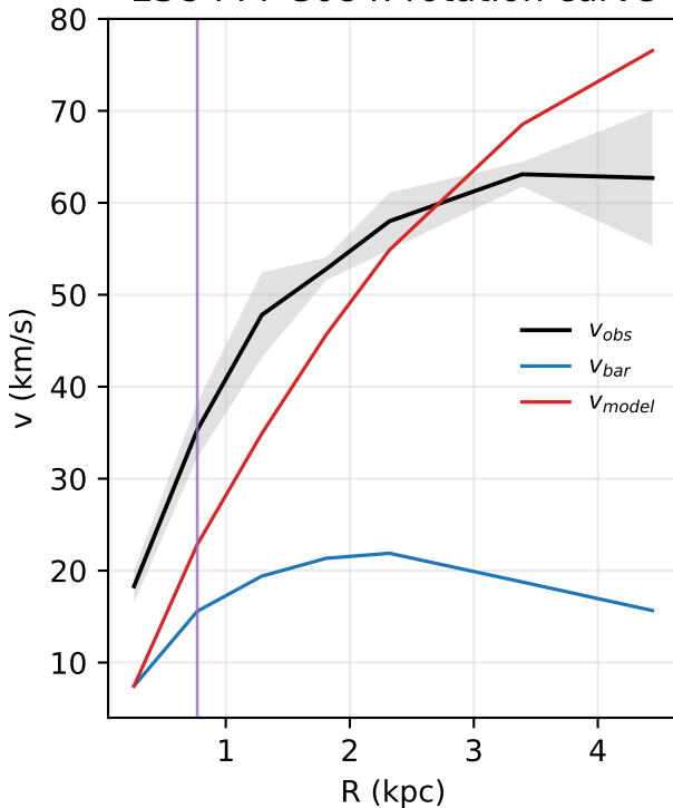
ESO444-G084: rotation curve
