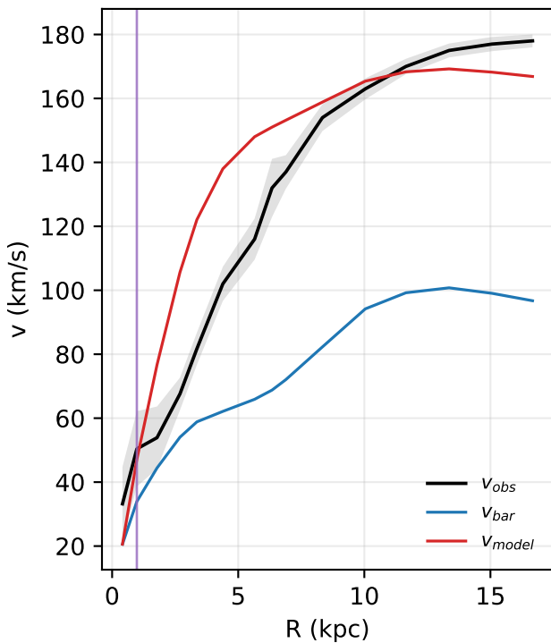
ESO079-G014: rotation curve
