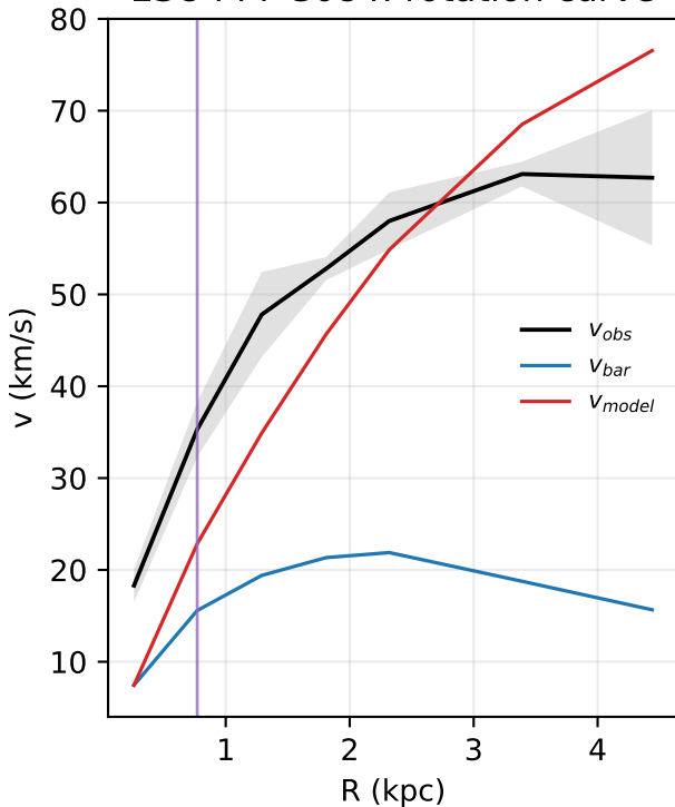
ESO444-G084: rotation curve
