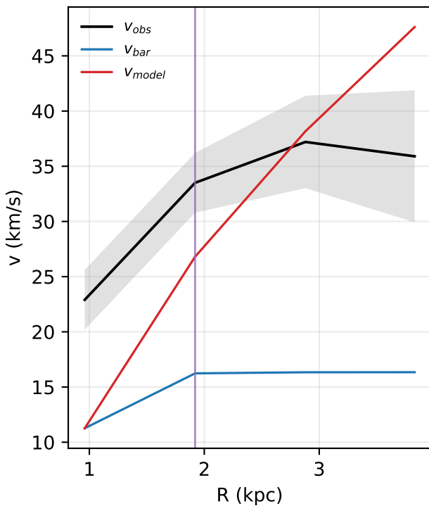
D512-2: rotation curve
