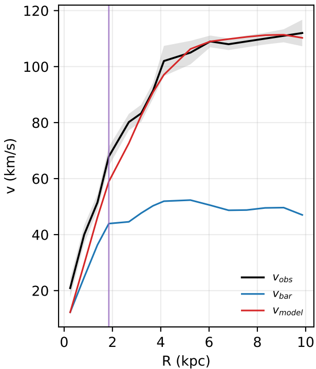
ESO116-G012: rotation curve
