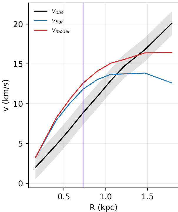
CamB: rotation curve
