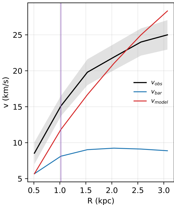
D564-8: rotation curve
