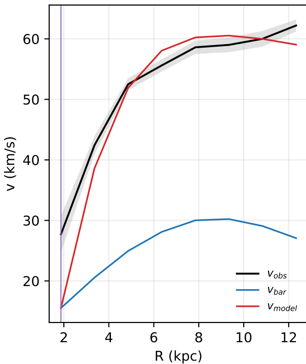
DDO170: rotation curve
