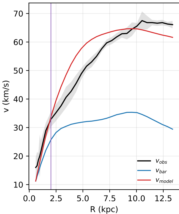
DDO161: rotation curve
