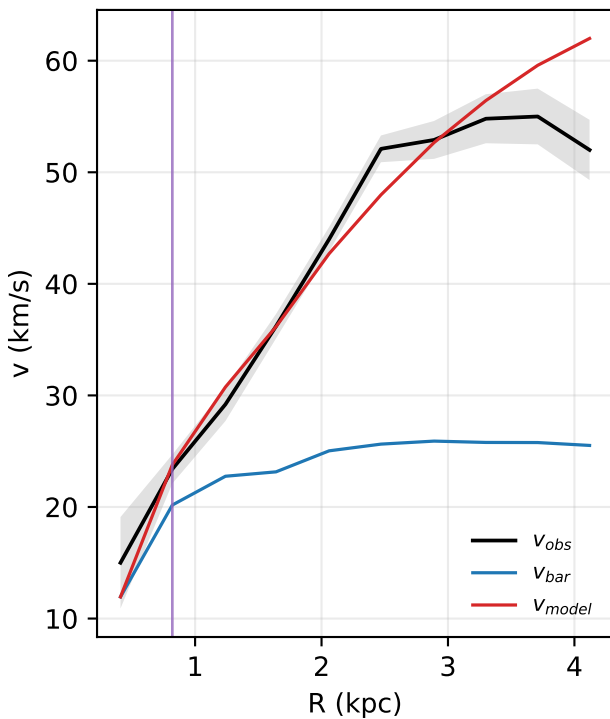
DDO168: rotation curve
