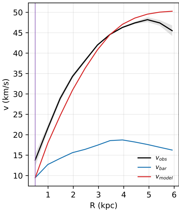
DDO154: rotation curve
