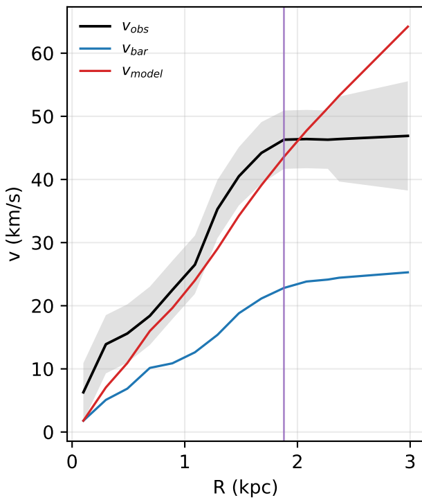
DDO064: rotation curve
