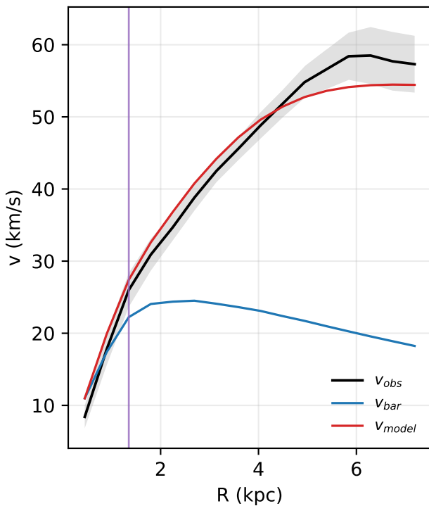
D631-7: rotation curve
