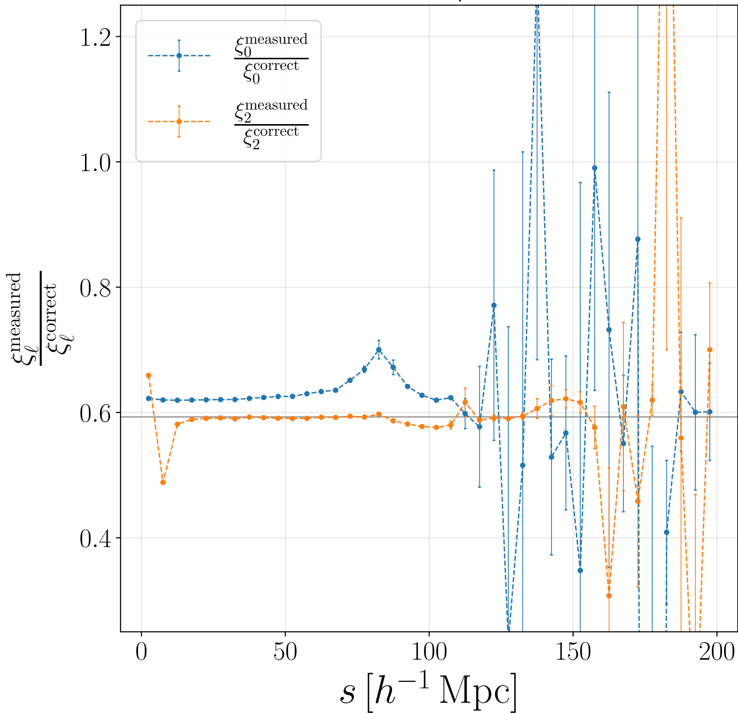
Ratio multipoles
