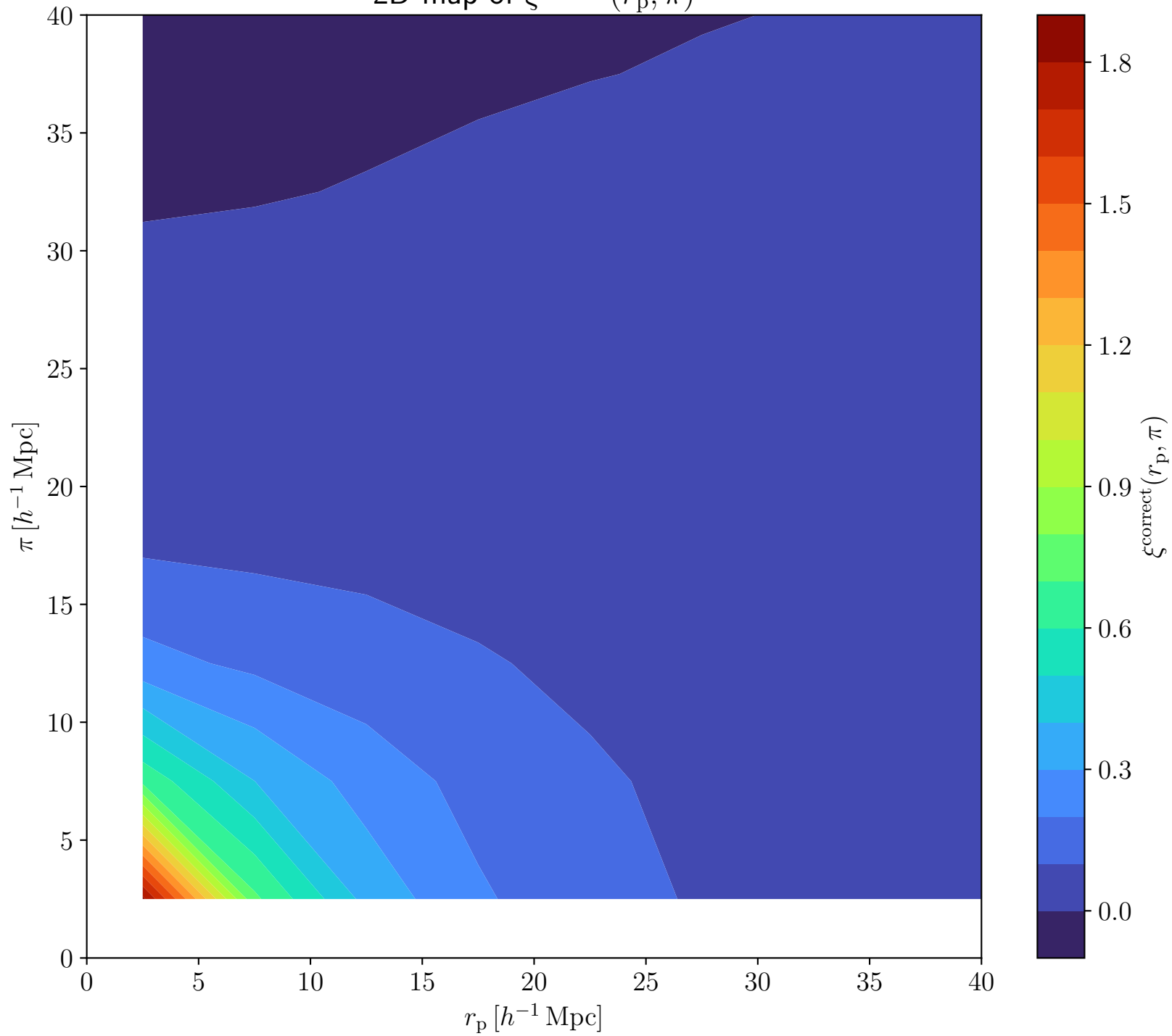
2D map of \xi^{\text{correct}}(r_p, \pi)
