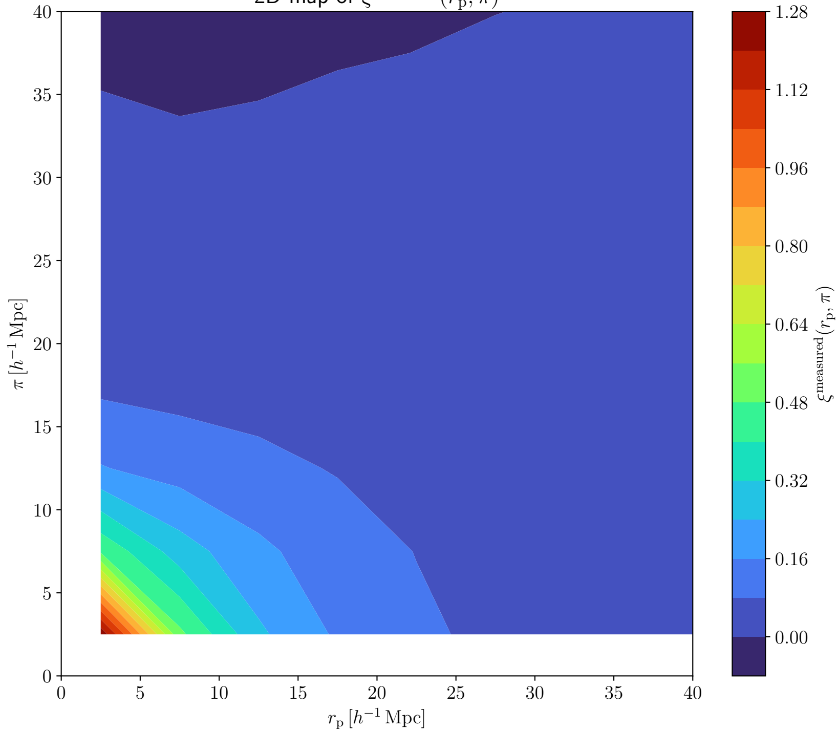
2D map of \xi^{\text{measured}}(r_p, \pi)
