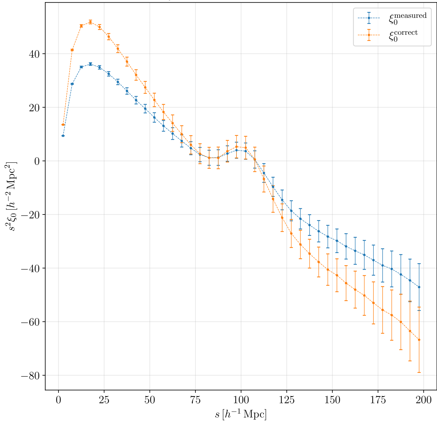
Multipole l = 0 Measured VS Correct
