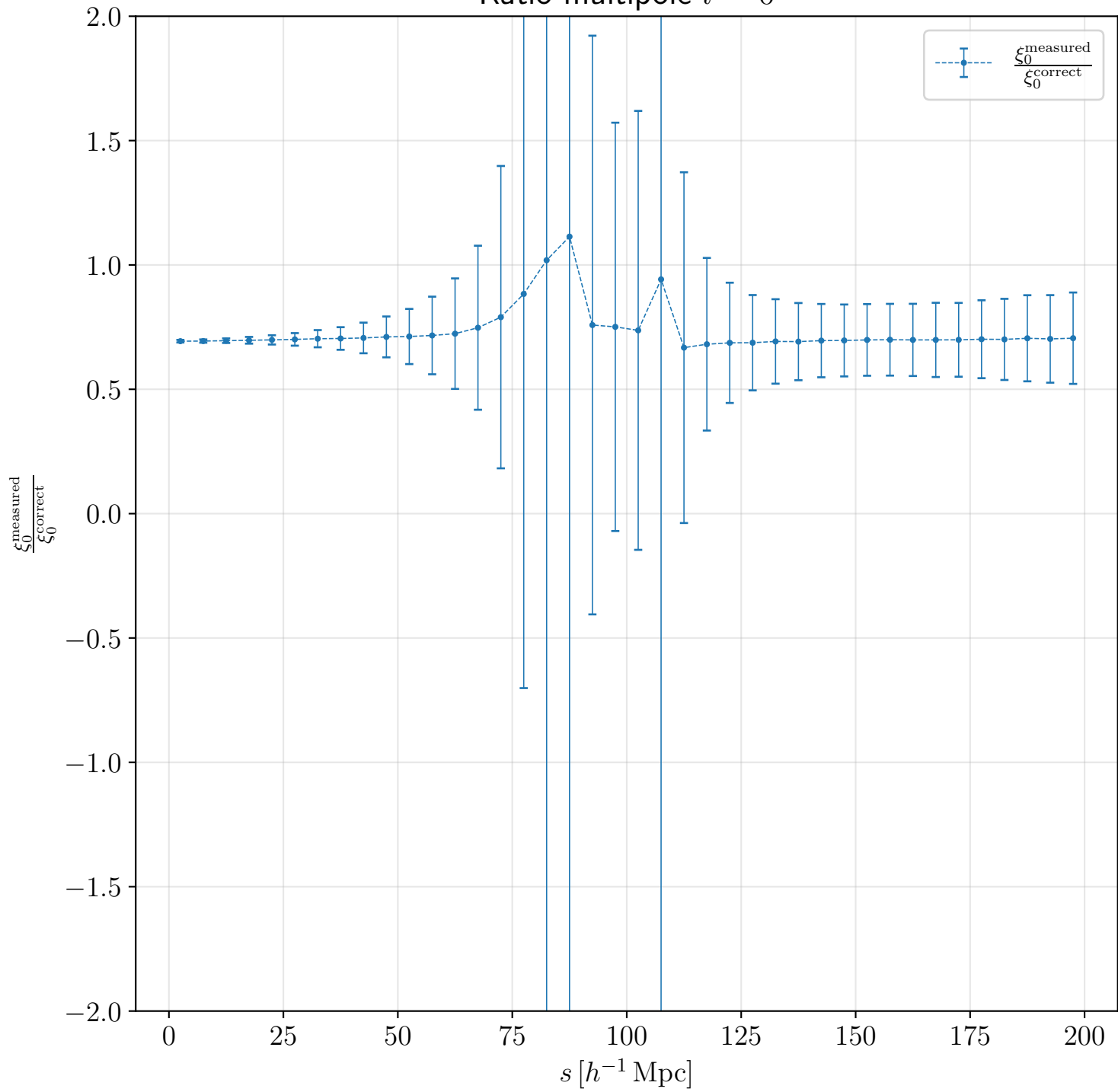
Ratio multipole l = 0
