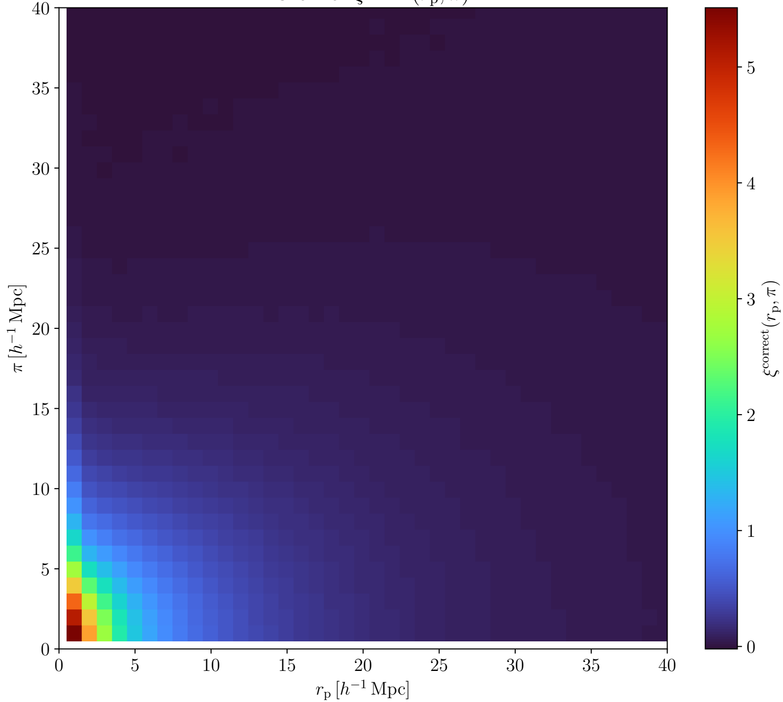
imshow of \xi^{\text{correct}}(r_p, \pi)
