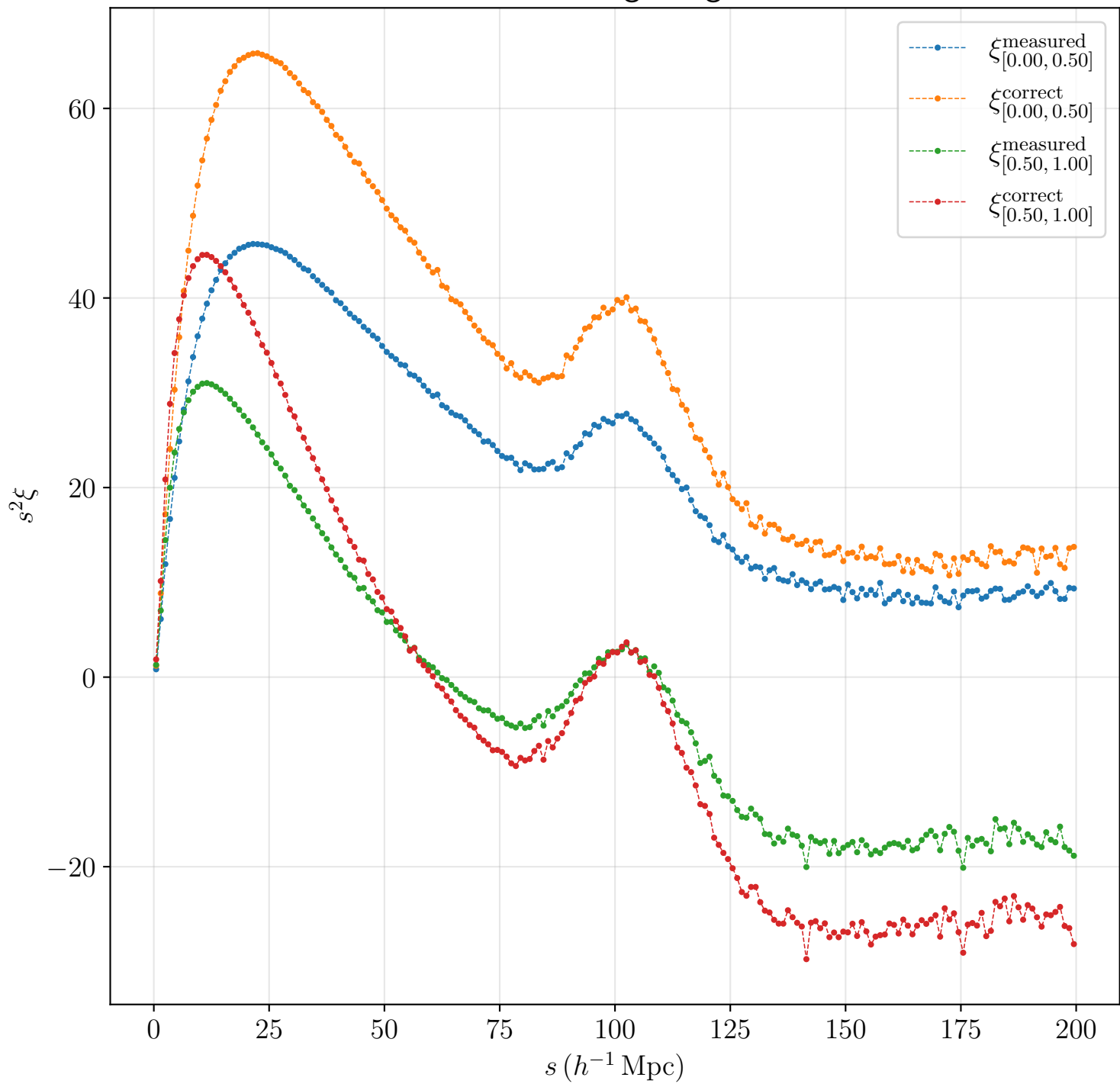
2 clustering wedges
