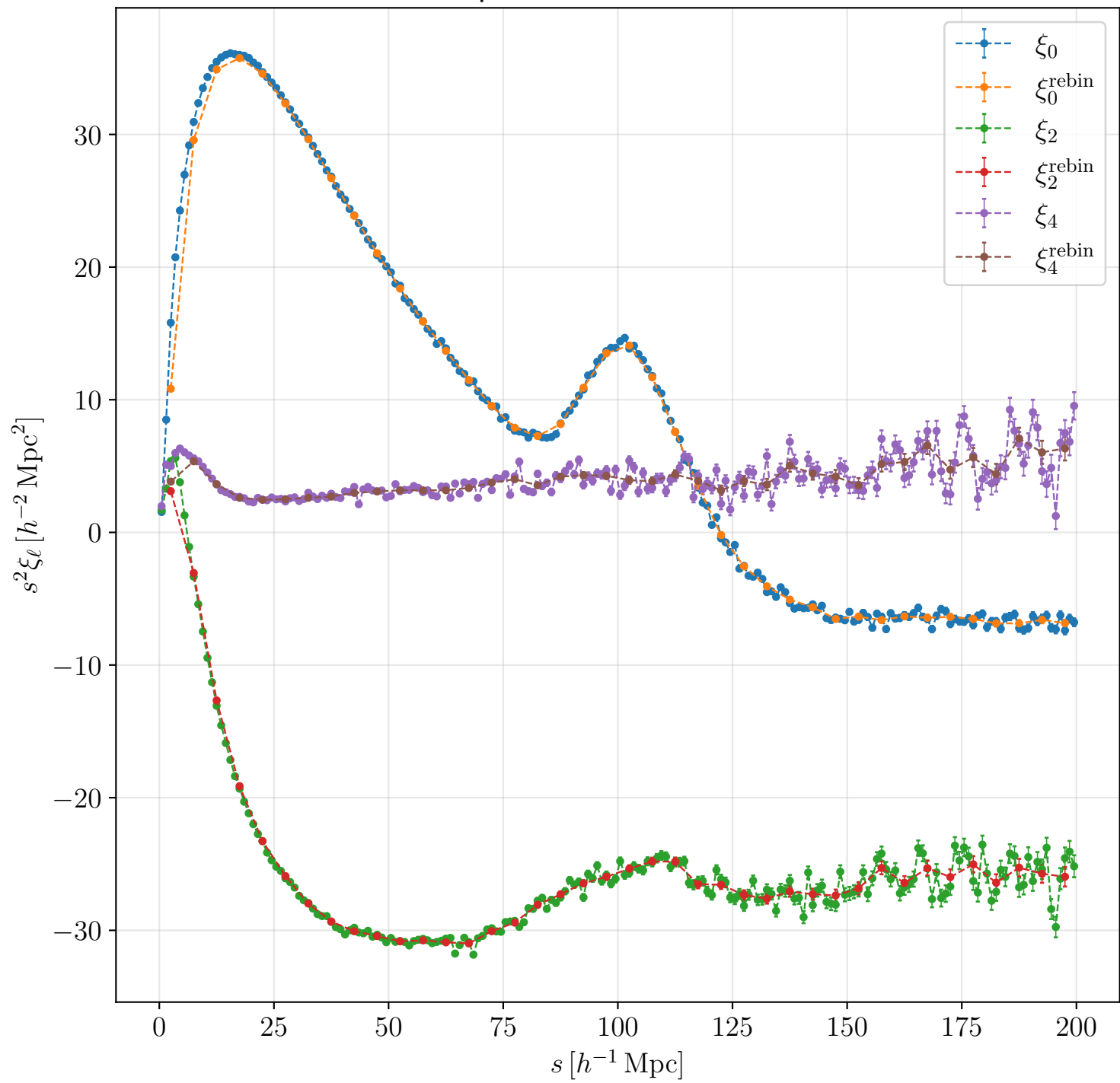
Multipoles Rebin VS Not rebin
