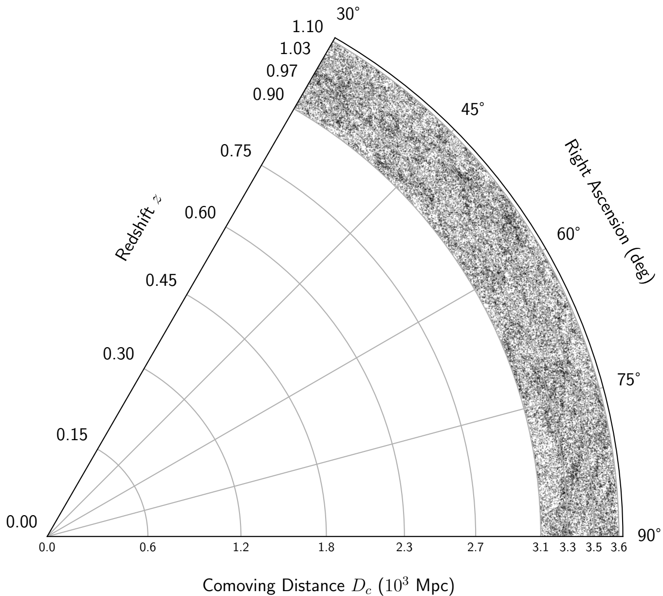
Wedge diagram within 48.0^\circ \leq \text{DEC} \leq 53.0^\circ
