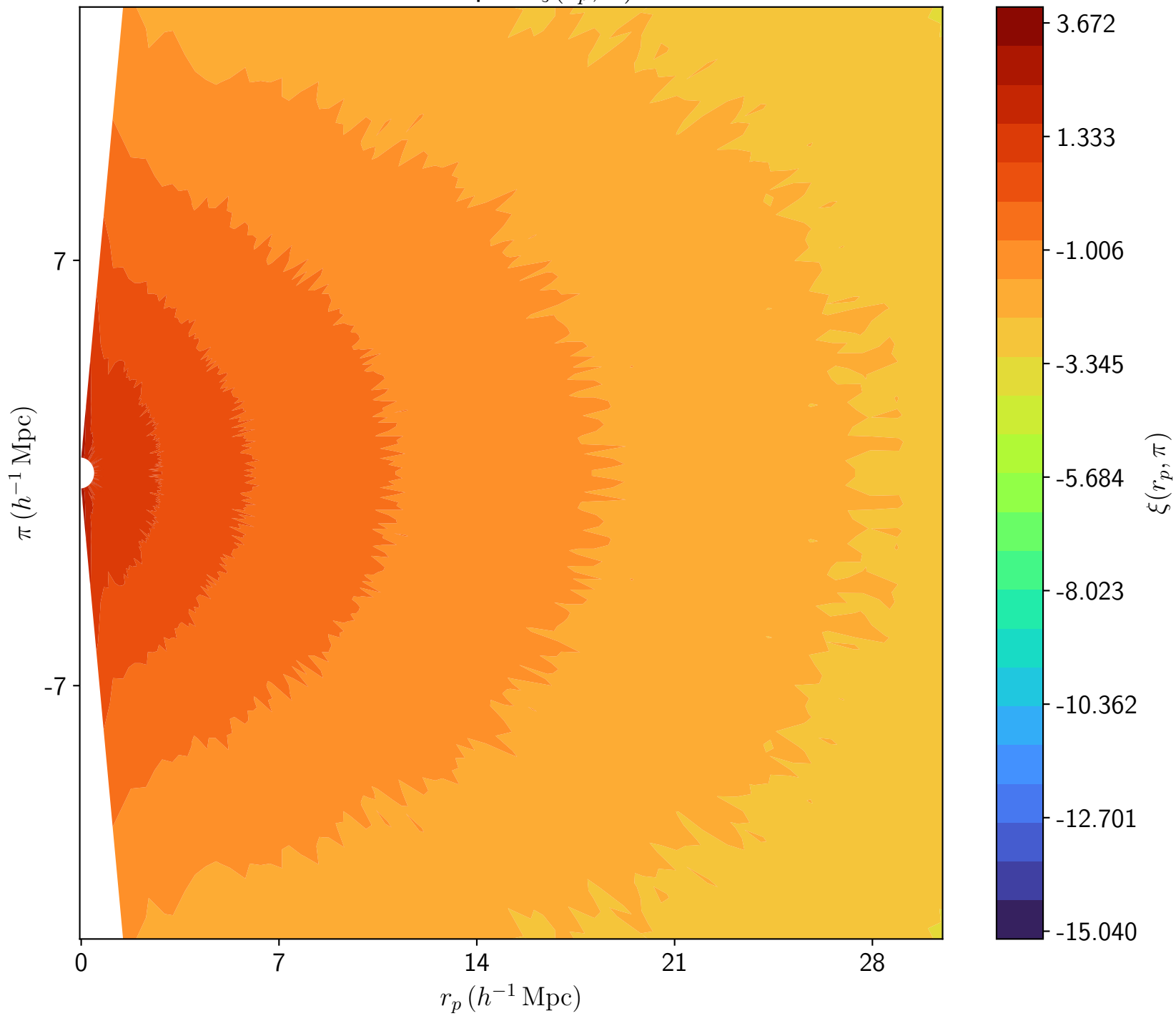
2D map of \xi(r_p, \pi)
