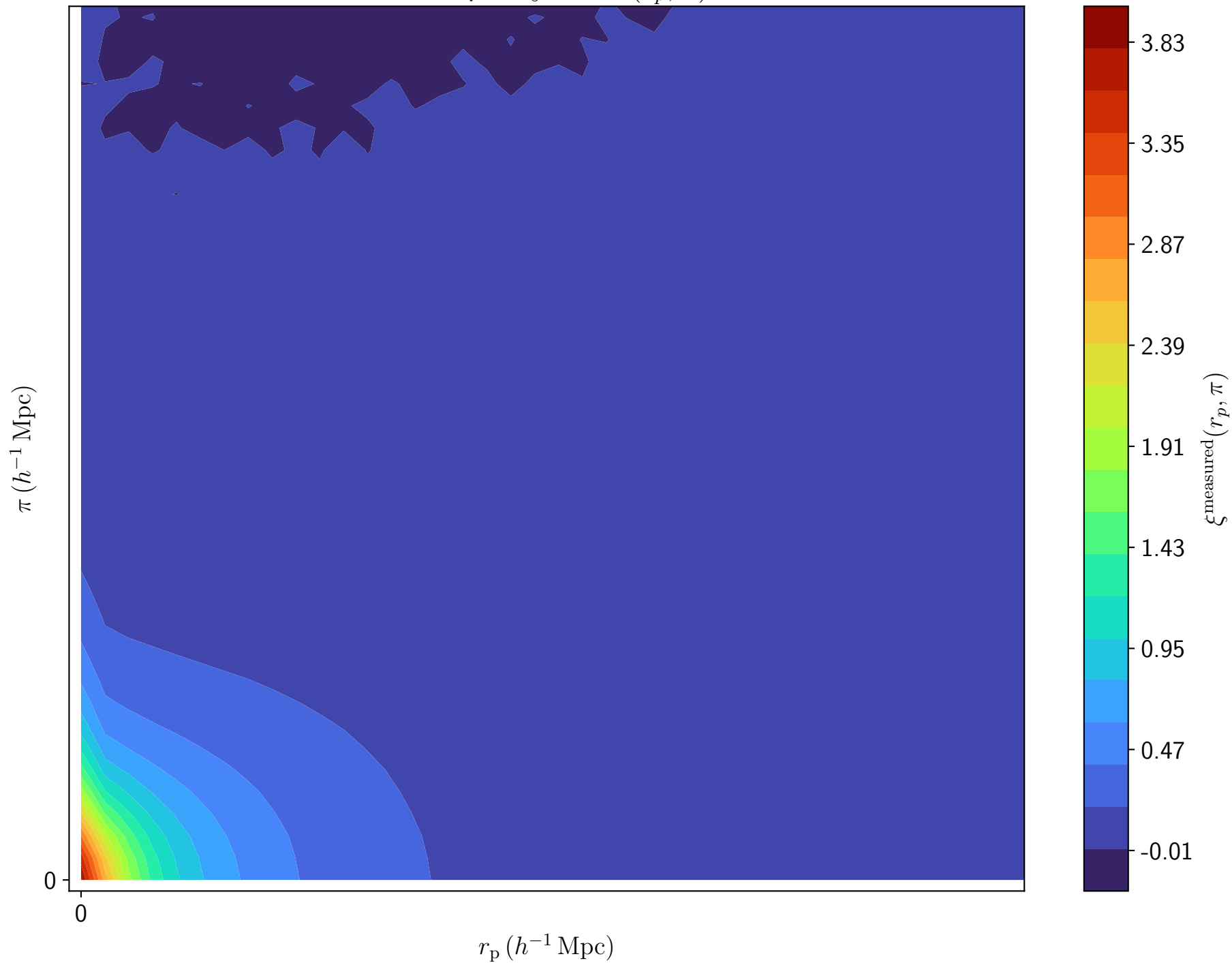
2D map of \xi^{\text{measured}}(r_p, \pi)
