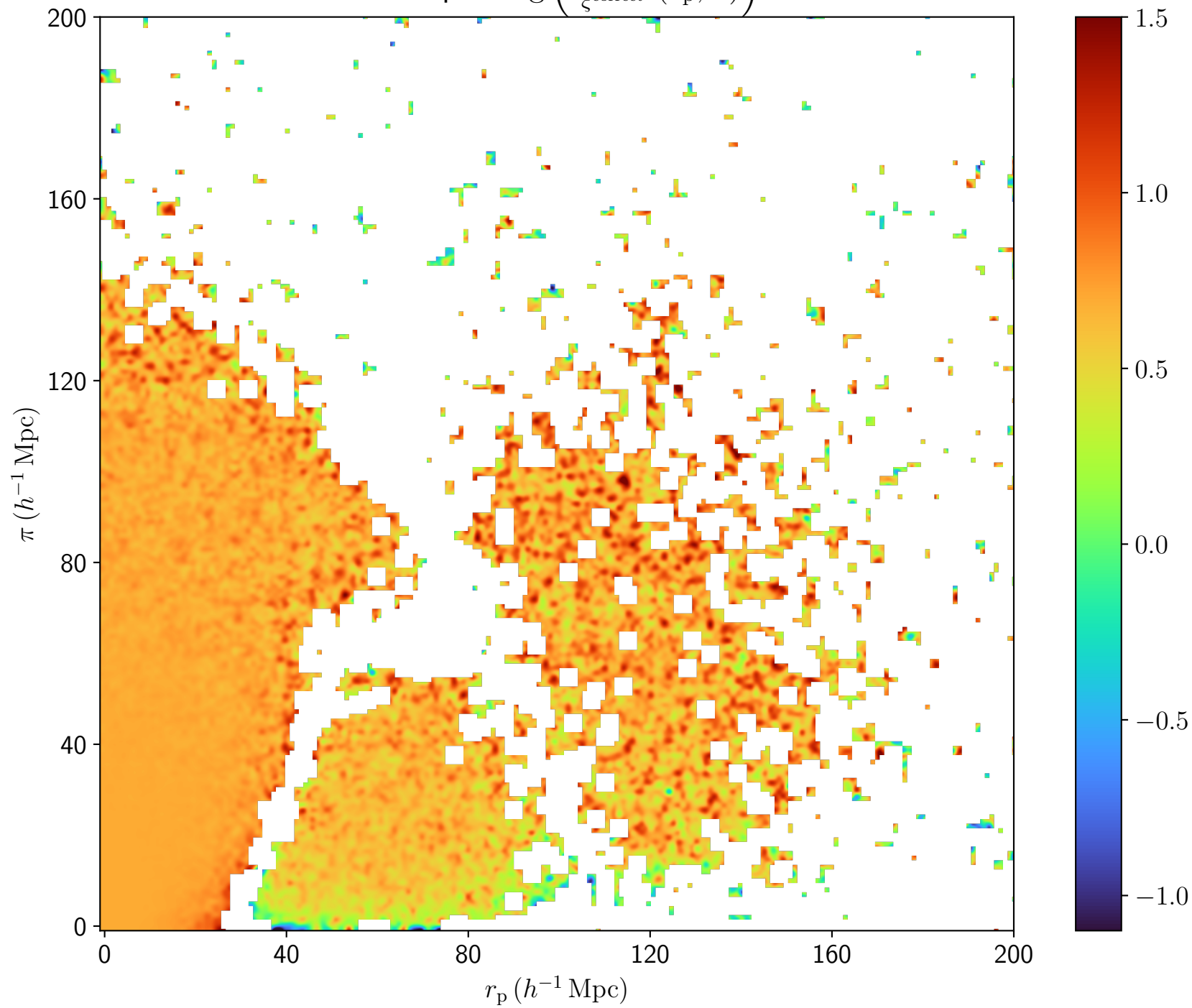
2D map of \log\left(\frac{\xi_{\text{measured}}}{\xi_{\text{correct}}}(r_p, \pi)\right)
