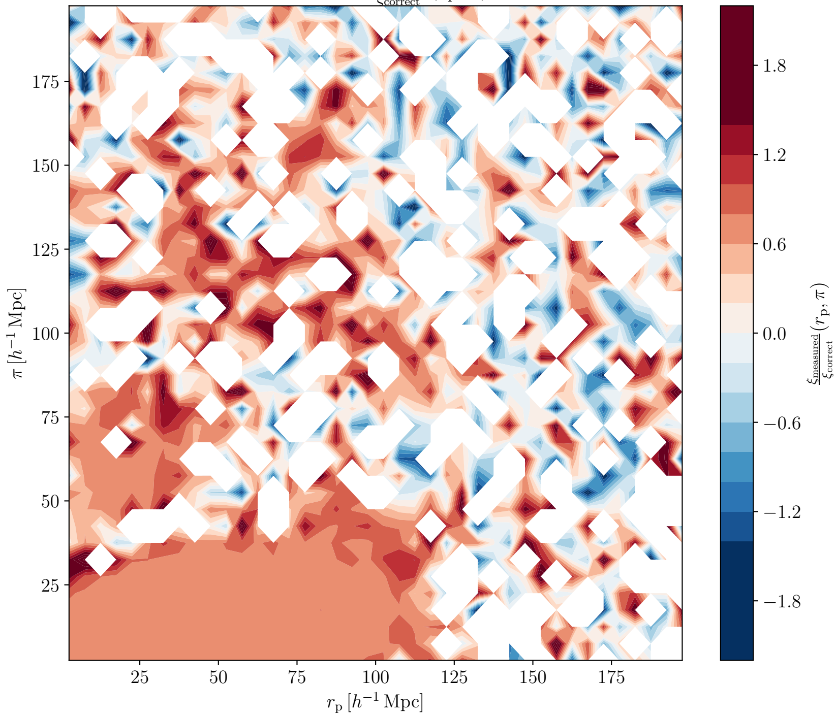
2D map of \frac{\xi_{\text{measured}}}{\xi_{\text{correct}}}(r_p, \pi)
