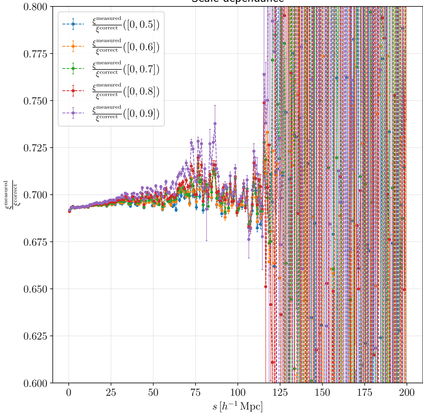
Scale dependence
